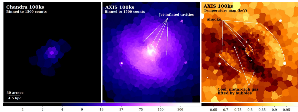
Figure 6. (Left,Center): Chandra (at launch) and AXIS-simulated images of AGN feedback in NGC 5813 (100 ks) with spatial binning for 1500 counts per region. Color bars are matched and units are counts arcsec -2 . The radio jet has carved out large cavities in the galaxy’s hot atmosphere, which are visible in the AXIS simulation as depressions in the X-ray surface brightness. With 1500 counts per region, AXIS will map the gas properties on these spatial scales to an accuracy of a few percent points in temperature. The spatial bins are generated with the contour binning algorithm and group pixels with similar surface brightness [50]. All panels cover the same field of view. (Right): Simulated temperature map in keV for a 100 ks AXIS observation, which probes the thermodynamic properties on the scales of the bubble rims, shocks, and cool gas plumes [51,52].
