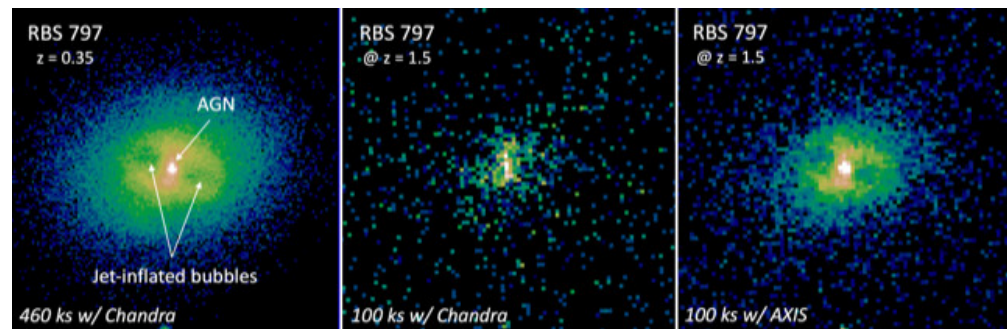
Figure 11. (Left): Chandra observation of the X-ray cavities in RBS797. Two cavities are visible \sim 30 kpc to the E and W of the AGN and are each \sim 30 kpc across (e.g., [81]). (Center) and (right): Chandra and AXIS simulations of RBS797 scaled for a mass of M_{500} = 5 \times 10^{14} M_{\odot} at z = 1.5 (applying cosmological dimming, reducing angular size, etc.). AXIS will extend measurements of AGN feedback in these environments into the high redshift regime for the first time.
