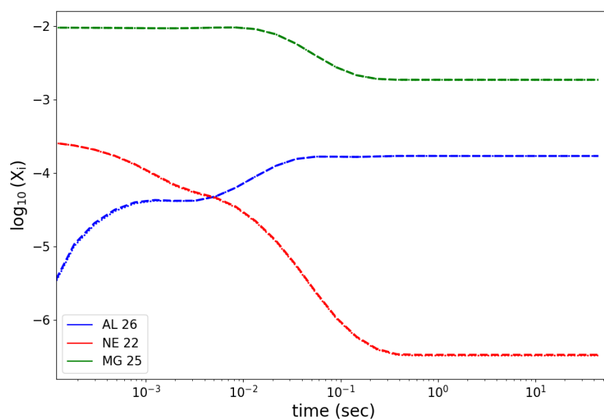
Figure 5. The evolution of the isotopic abundances (mass fractions) of ^{22}\text{Ne} , ^{25}\text{Mg} , and ^{26}\text{Al} is shown during the CCSN explosion using the JINA rates (thin lines) and LUNA rates (thick lines).
