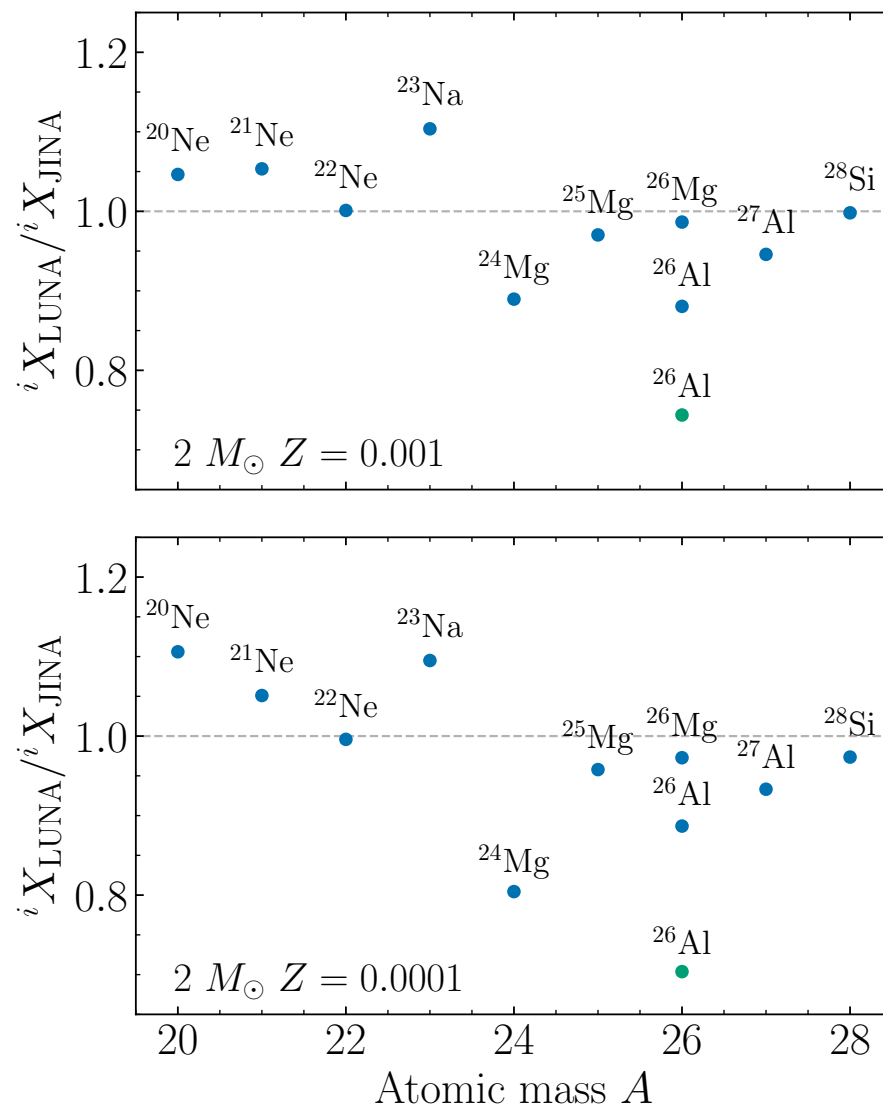
Figure 2. (Upper panel): Final surface abundance ratios in our low-mass AGB models at Z = 0.001 of the |LUNA| case relative to the |JINA| case for Ne, Na, Mg, Al and Si stable isotopes and ^{26}\text{Al} . The two data points for ^{26}\text{Al} show the results obtained adopting two different mass-loss prescriptions (see text for details). (Lower panel): same as in the upper panel, but for the Z = 0.0001 case.
