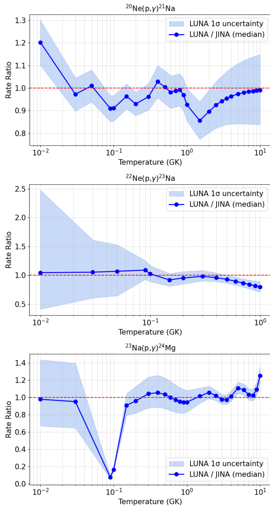
Figure 1. (Upper panel): Comparison of the LUNA and JINA ^{20}\text{Ne}(p,\gamma)^{21}\text{Na} nuclear reaction rate ratio as a function of temperature. The uncertainty band at the 1\sigma level is also included for the LUNA rates. (Middle panel): same as in the upper panel, but for the ^{22}\text{Ne}(p,\gamma)^{23}\text{Na} reaction. (Lower panel): same as in the upper panel, but for the ^{23}\text{Na}(p,\gamma)^{24}\text{Mg} reaction.
