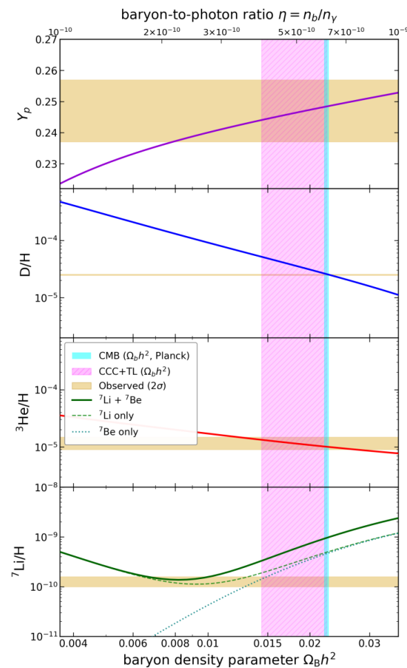
Figure 6. Schramm plot of BBN elemental abundances. The CCC+TL vertical column shows the spread in the values of baryon density calculated using Pantheon+ (lower value edge) and the CMB
