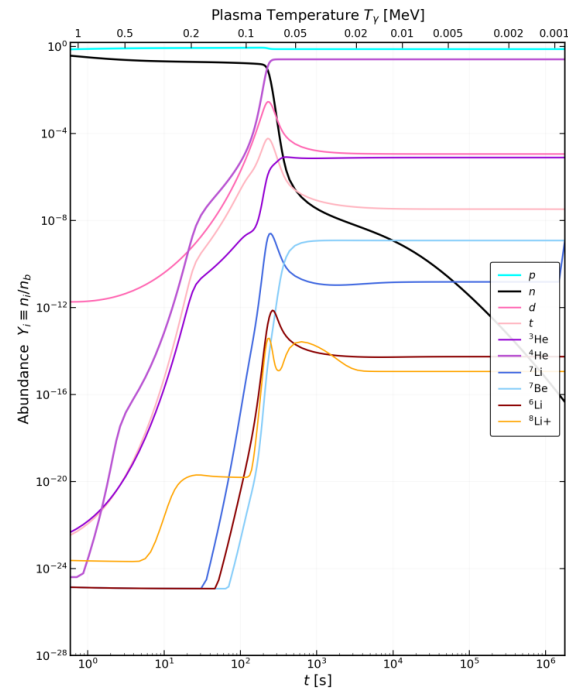
Figure 5. Abundance of light elements' nucleosynthesis with time using the \Lambda CDM clock. The abundance cut-off was set at 10^{-25} . The temperature scales are the same in the \Lambda CDL and CCC+TL models, but the clock is three times slower in CCC+TL.
