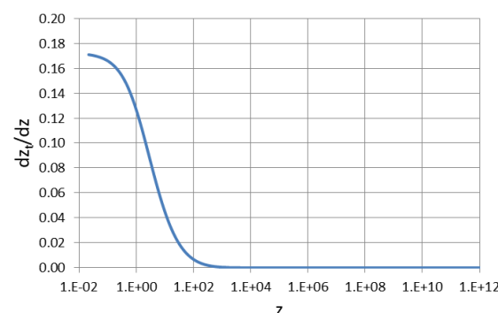
Figure 1. The tired light contribution to the observed redshift with typical H_{c,0} and \alpha parameters. It shows a complete absence of the tired light effect at the BBN epoch.
