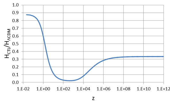
Figure 3. Variation of H_{CTL}/H_{\Lambda CDM} with z . The ratio has a fixed value, 1/f_{max} , at BBN redshifts.
