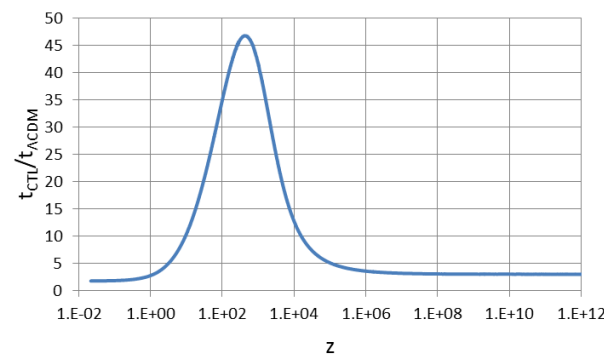
Figure 4. Variation of t_{CTL}/t_{\Lambda CDM} with z . The ratio has a fixed value, f_{max} , at BBN redshifts.
