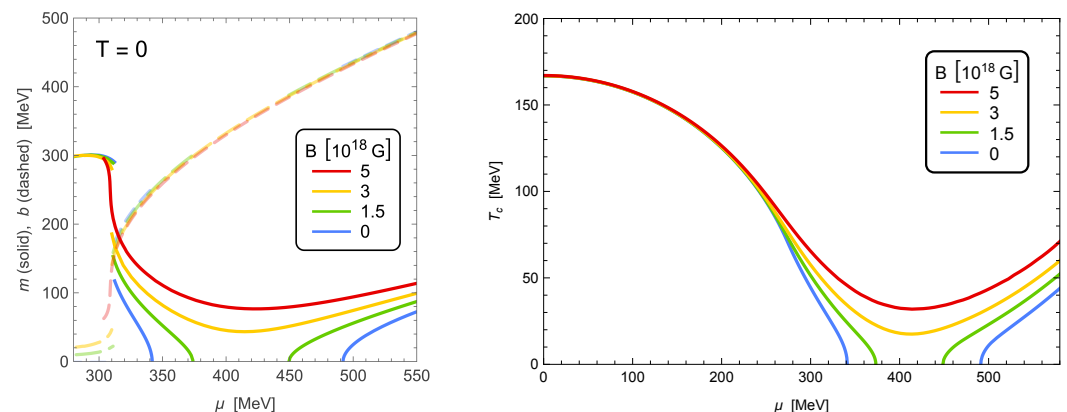
Figure 3. Order parameters (left panel) and critical temperature (right panel) of MDCDW at various magnetic fields from 0 – 5 \times 10^{18} G. All data are computed with a 30th-order GL expansion. Small but nonzero “remnant” values of m and T_c at intermediate \mu for 1.5 \times 10^{18} G are not captured by the GL expansion; thus, the curves vanish over this region, even though in principle T_c > 0 everywhere. The (right panel) is adapted from Figure 4 of Ref. [35].
