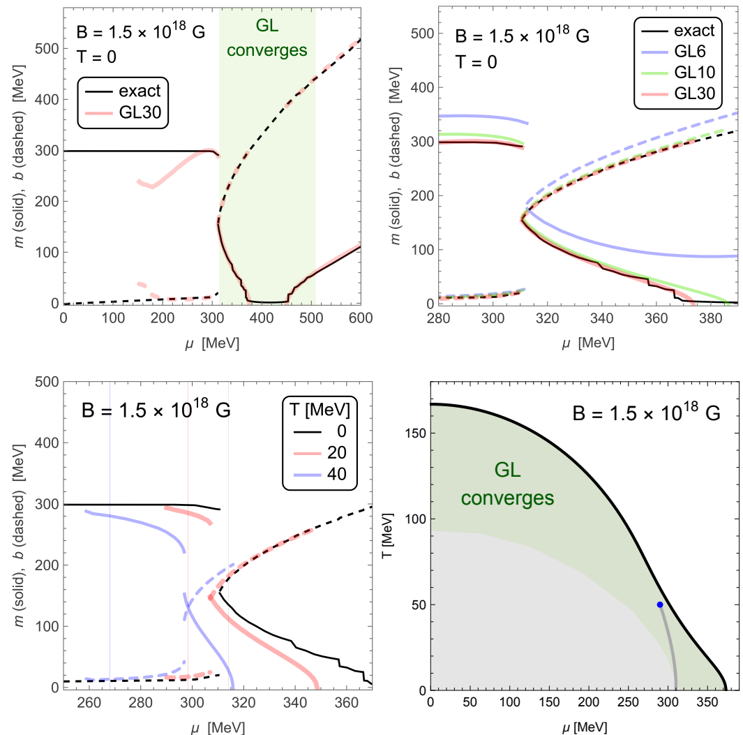
Figure 2. Ground state order parameters and phase diagrams of the MDCDW phase at B = 1.5 \times 10^{18} G. In all panels except the (bottom-right), m is plotted with solid lines and b with dashed lines. Each panel here is the analogous version at 1.5 \times 10^{18} G of the corresponding panel in Figure 1. Key differences between the two panel sets are discussed in the text.
