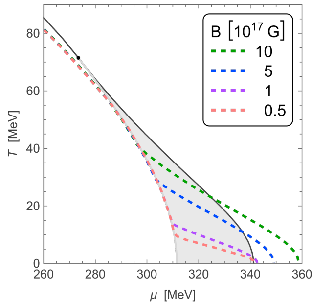
Figure 8. Threshold temperature curves of Figure 7 superposed on the phase diagram of DCDW. The gray shaded region indicates where the DCDW phase is inhomogeneous. The threshold temperature for MDCDW vanishes as B \rightarrow 0 only over the region of chemical potentials where the inhomogeneous phase is favored in the limit. At smaller \mu , the threshold temperature stabilizes along the homogeneous–inhomogeneous phase boundary. This figure is adapted from Figure 6 of Ref. [36].
