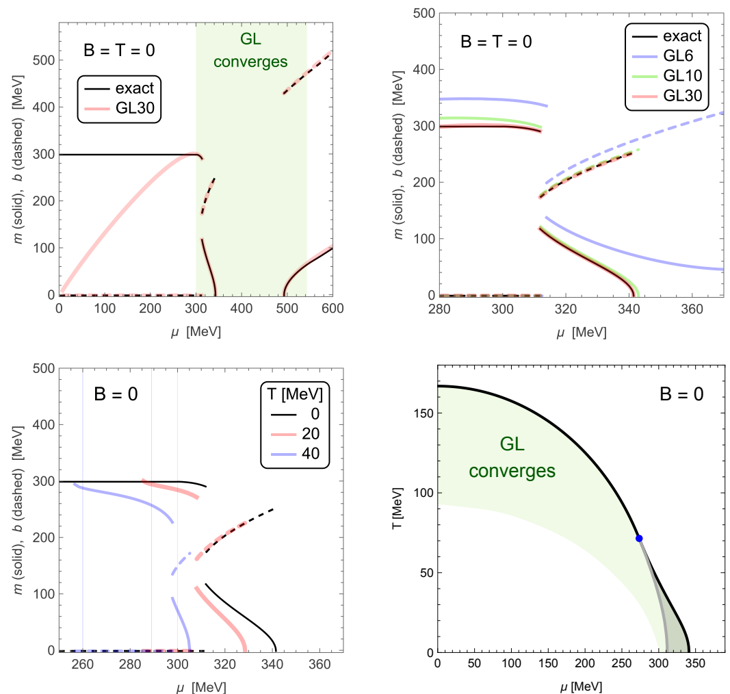
Figure 1. Ground state order parameters and phase diagrams of the DCDW phase ( B = 0 ). In all panels except the ( bottom-right ), m is plotted with solid lines and b with dashed lines. ( Top ): Both upper panels show values of m and b that minimize the free energy at T = 0 , computed using the exact free energy (black curves) and GL expansions of various orders (colored curves). The green region in the ( top-left ) panel indicates where m + b < \mu and hence the GL expansion is reliable. ( Bottom Left ): m and b are plotted at three temperatures. Data for T > 0 are computed with a 30th-order GL expansion. The thin vertical lines indicate where m = \mu for the corresponding temperature, which is the edge of the region where the GL expansion is reliable. ( Bottom Right ): The black curve shows the critical temperature, i.e., where m vanishes and chiral symmetry is restored. The condensate is inhomogeneous in the gray shaded region, which is separated from the homogeneous phase by a first-order transition depicted by a gray line. The blue dot is a critical point where the first-order transition disappears; in the B = 0 case, this point occurs at the critical temperature (compare with the B > 0 case in Figure 2). The green shaded region (which encompasses the entire inhomogeneous region) indicates where m + b < \sqrt{\mu^2 + (\pi T)^2} , and hence the GL expansion converges in the ground state.
