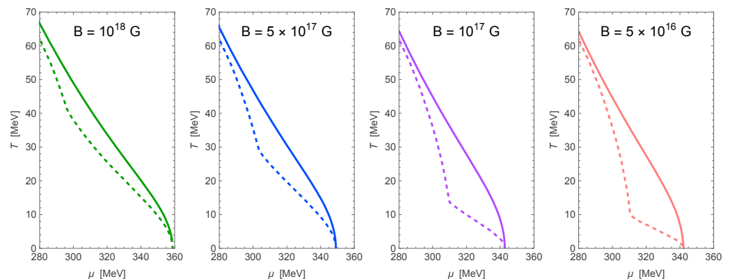
Figure 7. Critical temperature (solid) and threshold temperature (dashed) at magnetic fields ranging from 5 \times 10^{16} – 10^{18} G in decreasing order. As the magnetic field decreases, the threshold temperature decreases, both absolutely and relative to T_c , for \mu > 311 MeV. This is the region where DCDW is inhomogeneous, so the LP instability returns in the limit B \rightarrow 0 . This figure is adapted from Figure 5 of Ref. [36].
