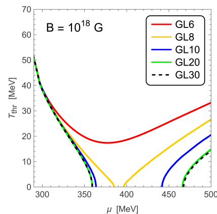
Figure 5. Threshold temperature at B = 10^{18} G computed at various orders of the GL expansion. The lower-order expansions are not very accurate, but results stabilize by at least 30th order. This figure is adapted from Figure 1 of Ref. [36].
