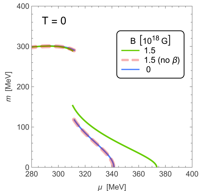
Figure 4. The order parameter m for MD CDW with a magnetic field of 1.5 \times 10^{18} G, calculated using a GL expansion that includes the \beta_{i,j} coefficients (green curve) and one that does not include the \beta_{i,j} coefficients (red dotted curve). The latter is indistinguishable from the same curve for the DCDW phase, where B = 0 (blue curve).
