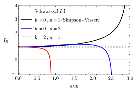
Figure 6. Regular integral as a function of parameter a .
