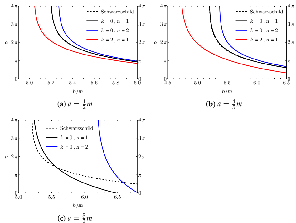
Figure 7. Strong field approximation for different space-times and fixed a .
