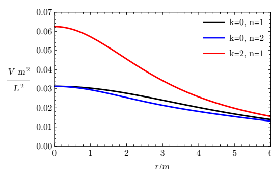
Figure 4. Effective potential for different spacetimes with large a ( a = 4m ). It is evident that r = 0 represents a potential peak, i.e., a photon sphere, for all metrics considered.
