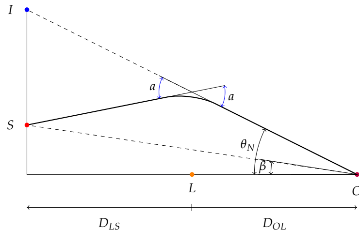
Figure 8. Schematic representation of the observer (O), the source (S), the lens (L) and the image (I).
