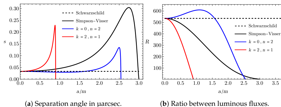
Figure 9. Observables as a function of parameter a with Sagittarius A* acting as a gravitational lens.
