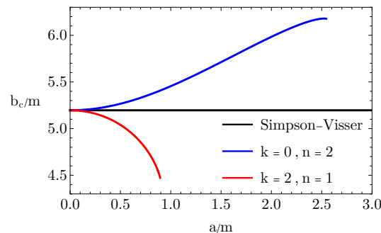
Figure 5. Critical impact parameter, equivalently the shadow radius r_s = b_c , as a function of the bounce parameter a for the Simpson–Visser and generalized black-bounce geometries.
