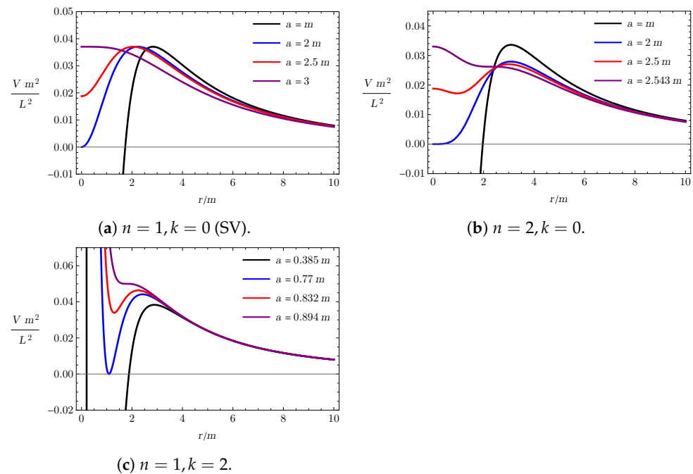
Figure 1. Effective potentials for some specific black-bounce spacetimes.
