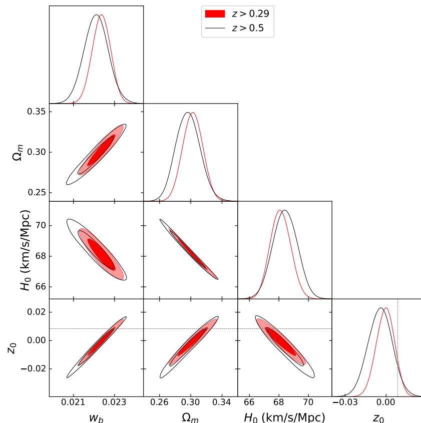
Figure 2. Triangle plot showing the inferred parameters with data from z > 0.5 (open black contours) or z > 0.29 (filled red contours). We show the 1\sigma and 2\sigma error ellipses in panels involving two parameters. The dotted line shows the a priori prediction that z_0 = 0.84\% (Section 5.3.3 of [73]).
