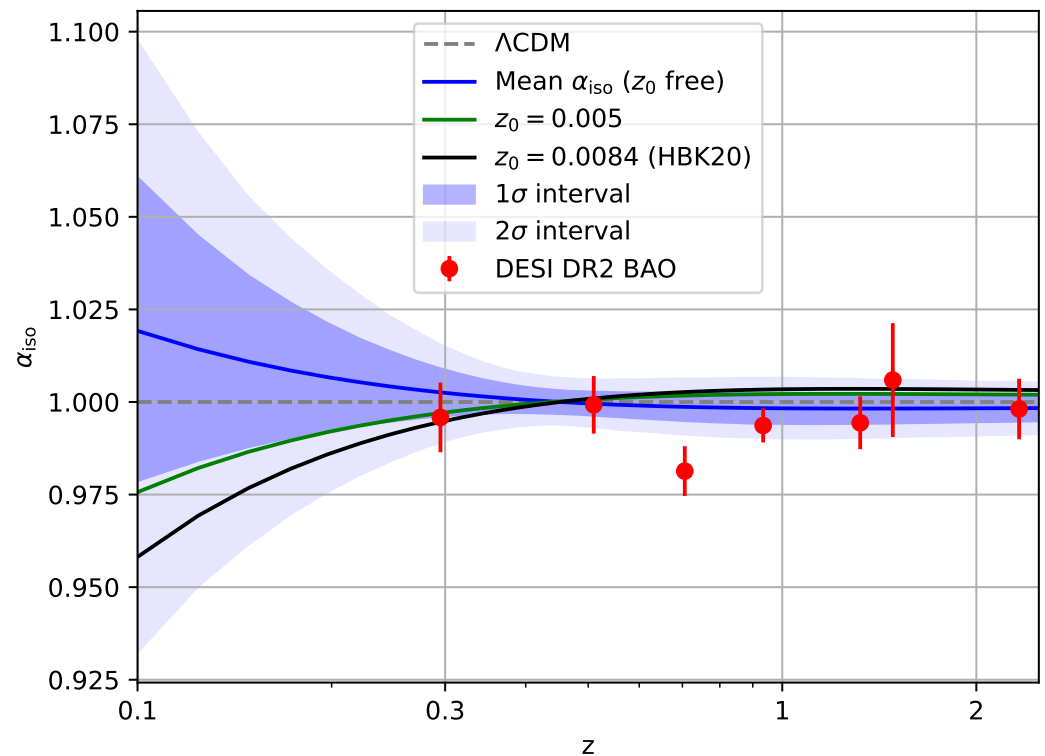
Figure 3. Reconstructed \alpha_{\text{iso}}(z) \equiv D_V/r_d in units of its fiducial value at each redshift, which, here, is the mean value from our \Lambda\text{CDM} nested sampling analysis using data at z > 0.5 (see the text). The solid blue line shows the mean result using our free z_0 analysis with the same data, while the shaded blue bands show the 1\sigma and 2\sigma uncertainties using Gaussian equivalent percentiles. The red data points with uncertainties show DESI DR2 measurements [50]. The solid green line shows the best-fitting model with z_0 = 0.5\% , while the solid black line assumes the previously expected value of z_0 = 0.84\% [73].
