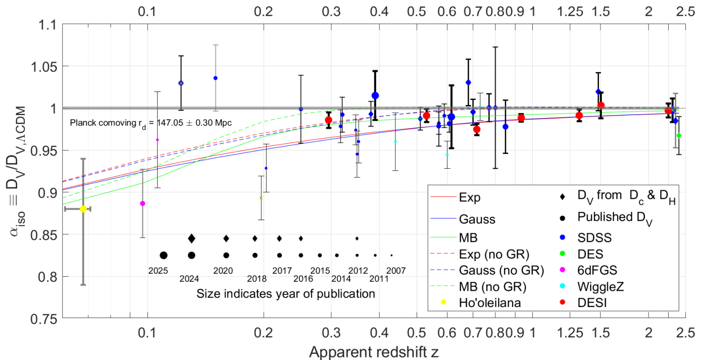
Figure 1. Ratio between the isotropically averaged BAO distance scale ( D_V ) and the \Lambda CDM prediction based on Planck observations of the CMB [10]. The shaded grey horizontal band shows a 0.2% uncertainty on the \Lambda CDM prediction due to the Planck uncertainty on r_d [10], though this does not properly account for the uncertainties (see the text). The coloured lines show predictions of the best-fitting void models from [73] with an initial underdensity profile that is exponential (red), Gaussian (blue), or Maxwell–Boltzmann (green). Solid lines show predictions including both non-cosmological redshift contributions in Equation (2), while the dashed lines in the same colour show the corresponding results without the GR contribution. This highlights that the dominant non-cosmological contribution is the Doppler effect at low redshift, while GR dominates at high redshift. Points with uncertainties show BAO measurements over the last 20 years, with different colours indicating different surveys and larger markers indicating more recent results, as indicated towards the bottom left. Reproduced from Figure 4 of Banik and Kalaitzidis [52].
