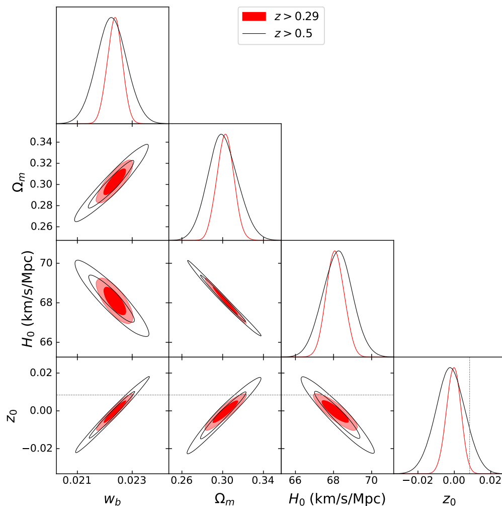
Figure 4. Triangle plot shown similarly to Figure 2 including also DES-Dovekie SNe Ia. The posteriors are now tighter than before, but the previously predicted z_0 = 0.84\% is still allowed at just over 2\sigma .
