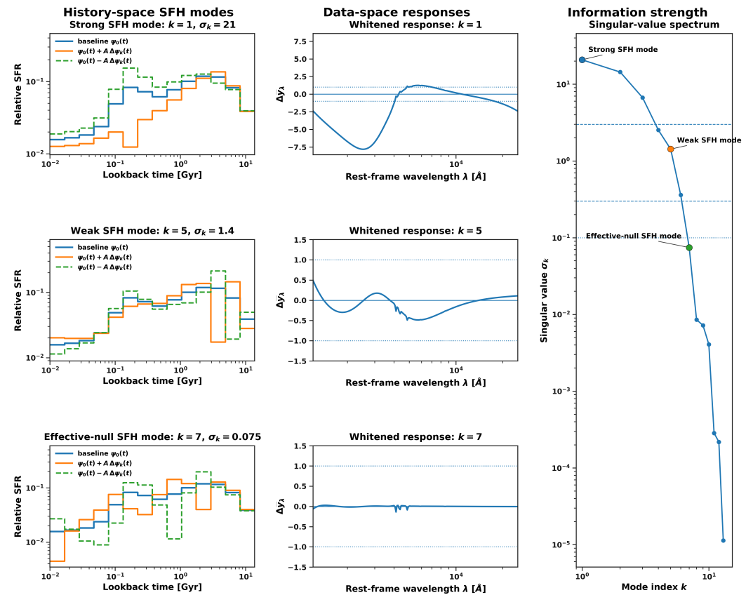
Figure 3. Illustrative singular-mode structure of an SFH inverse problem constructed with a reduced SSP library. The left panels show perturbations of a baseline SFH along representative right singular vectors, the middle panels show the corresponding whitened spectral responses, and the right panel shows the singular-value spectrum. Strong, weak, and effectively null modes illustrate how nominal SFH freedom is compressed into a smaller set of information-supported historical combinations.
