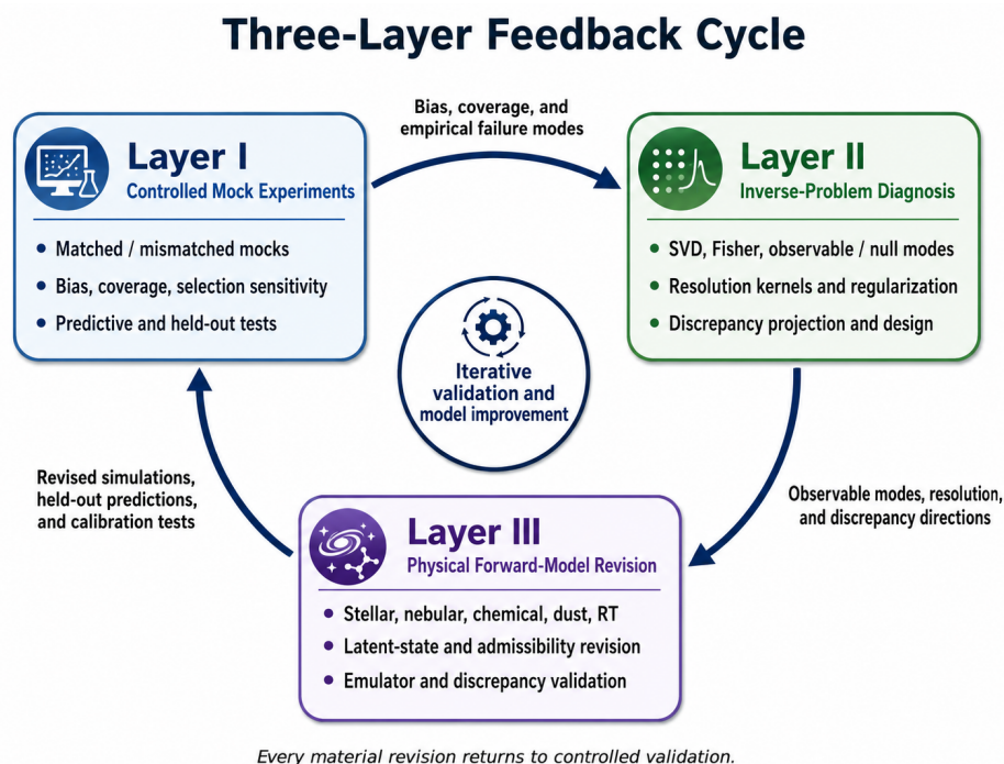
Figure 5. Three-layer feedback cycle for Integrated Galactic Archaeology. Layer I identifies empirical failure modes through controlled mock experiments, Layer II diagnoses their structural origins through inverse-problem analysis, and Layer III revises the state representation and forward-model hierarchy. Revised simulations and predictions then return to Layer I for renewed validation, so that every material change in the representation or forward model is tested within the complete cycle.
