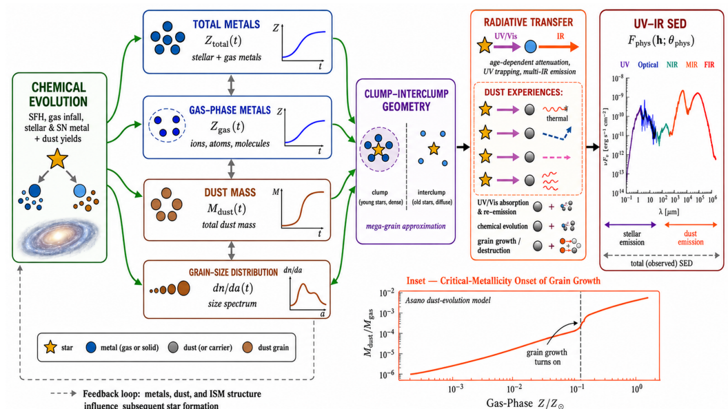
Figure 2. Schematic coupling of chemical evolution, dust evolution, subresolution geometry, and radiative transfer in a chemically consistent galaxy-SED model. Chemical evolution jointly determines the total and gas-phase metal states, dust mass, and grain-size distribution, which are coupled by grain growth, shattering, coagulation, and supernova destruction. Efficient interstellar grain growth produces a rapid increase in dust content after a critical metallicity is reached, as illustrated in the inset. The evolved dust state enters a clump–interclump radiative-transfer model that produces age-dependent attenuation, ultraviolet trapping, infrared re-emission, and the emergent UV–IR SED. All curves and internal tracks are schematic.
