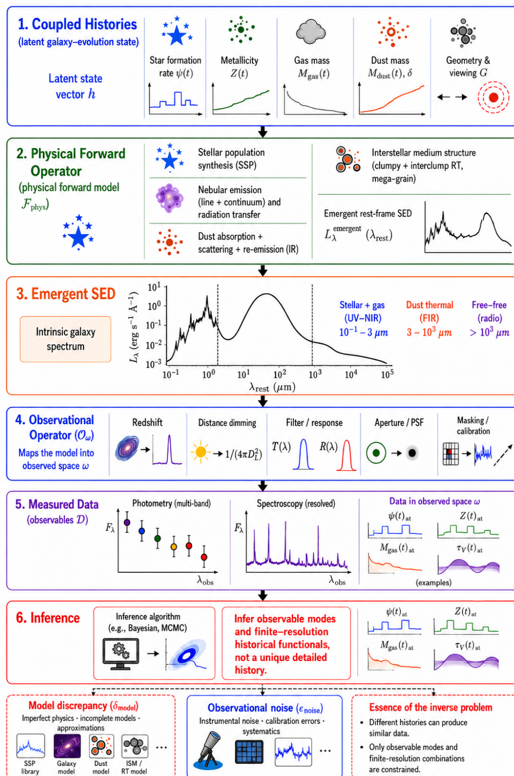
Figure 1. Conceptual overview of integrated galactic archaeology. Coupled histories of star formation, chemical enrichment, gas, dust, and geometry are mapped by the physical forward operator into an emergent rest-frame SED and then by the observational operator into photometric or spectroscopic data. Observational noise and model discrepancy enter as distinct limitations of this mapping. The inverse problem does not generally identify a unique detailed history, but constrains observable modes and finite-resolution historical functionals under the adopted physical, observational, and inferential model. The displayed spectral components and wavelength ranges are schematic.
