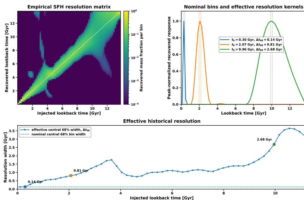
Figure 4. Illustrative injection-and-recovery analysis of nominal and effective SFH resolution. A localized formed-mass component is injected into each uniformly spaced lookback-time bin and recovered using a reduced SSP library, an illustrative UV–NIR observational operator, and a non-negative regularized inversion. The upper-left panel shows the resulting resolution matrix, the upper-right panel shows representative averaging kernels, and the lower panel shows their central 68% widths as a function of lookback time; the dashed line marks the corresponding width of one nominal bin. The broadening of the kernels toward older epochs illustrates that fine input binning does not imply equally fine historical resolution.
