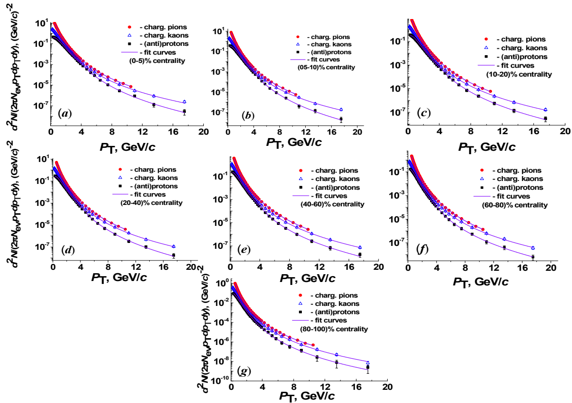
Figure 1. Simultaneous minimum \chi^2 fits (solid blue curves) with two-component model (THMTF) function (Equation (5)) of experimental midrapidity p_T spectra (symbols) of the charged pions and kaons, protons and antiprotons in different centrality classes of p +Pb collisions at \sqrt{s_{nn}} = 5.02 TeV: (a)–(0–5)%, (b)–(05–10)%, (c)–(10–20)%, (d)–(20–40)%, (e)–(40–60)%, (f)–(60–80)%, and (g)–(80–100)% centrality.
