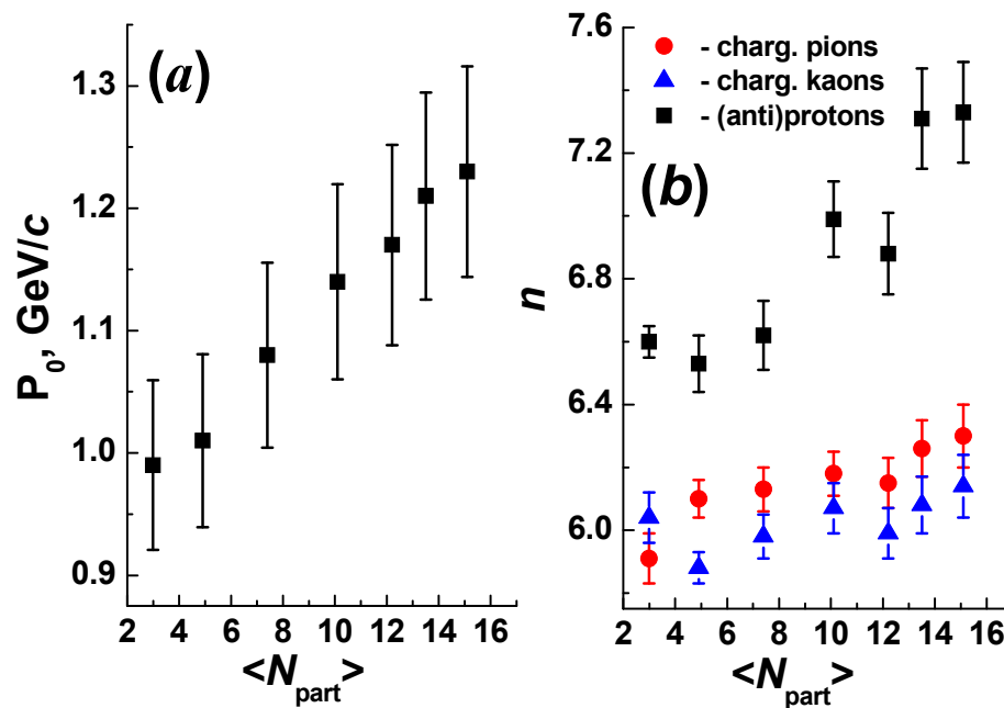
Figure 3. The dependencies of the obtained parameters P_0 (a) and n (b) of the two-component model (THMTF) function (Equation (5)), given in Table 2, on the average number of participant nucleons ( \langle N_{part} \rangle ) in p+Pb collisions at \sqrt{s_{nn}} = 5.02 TeV.
