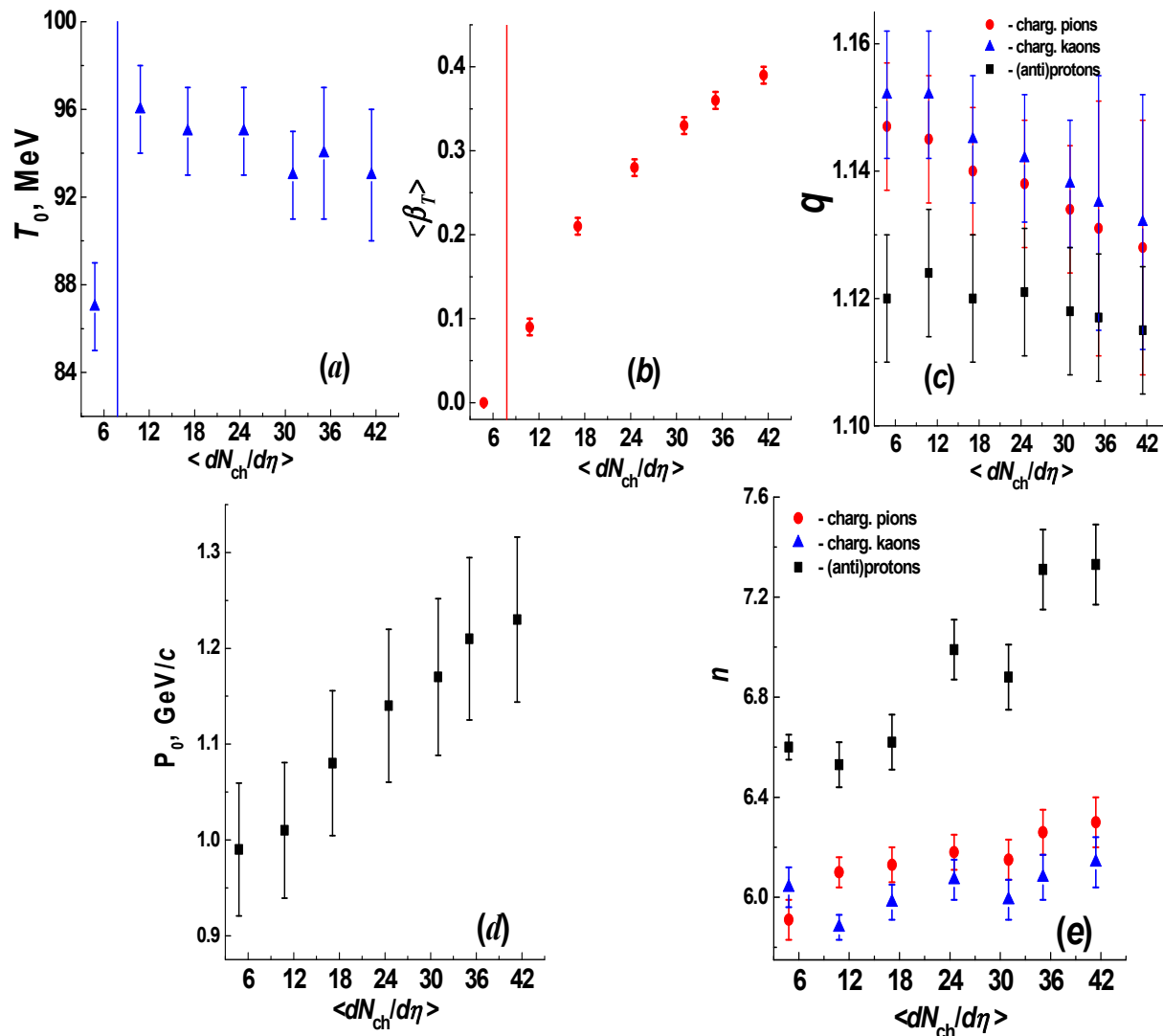
Figure 4. The dependencies of the obtained parameters T_0 (a), \langle \beta_T \rangle (b), q (c), P_0 (d) and n (e) of the two-component model (THMTF) function (Equation (5)), given in Table 2, on \langle dN_{ch}/d\eta \rangle in p+Pb collisions at \sqrt{s_{nn}} = 5.02 TeV.
