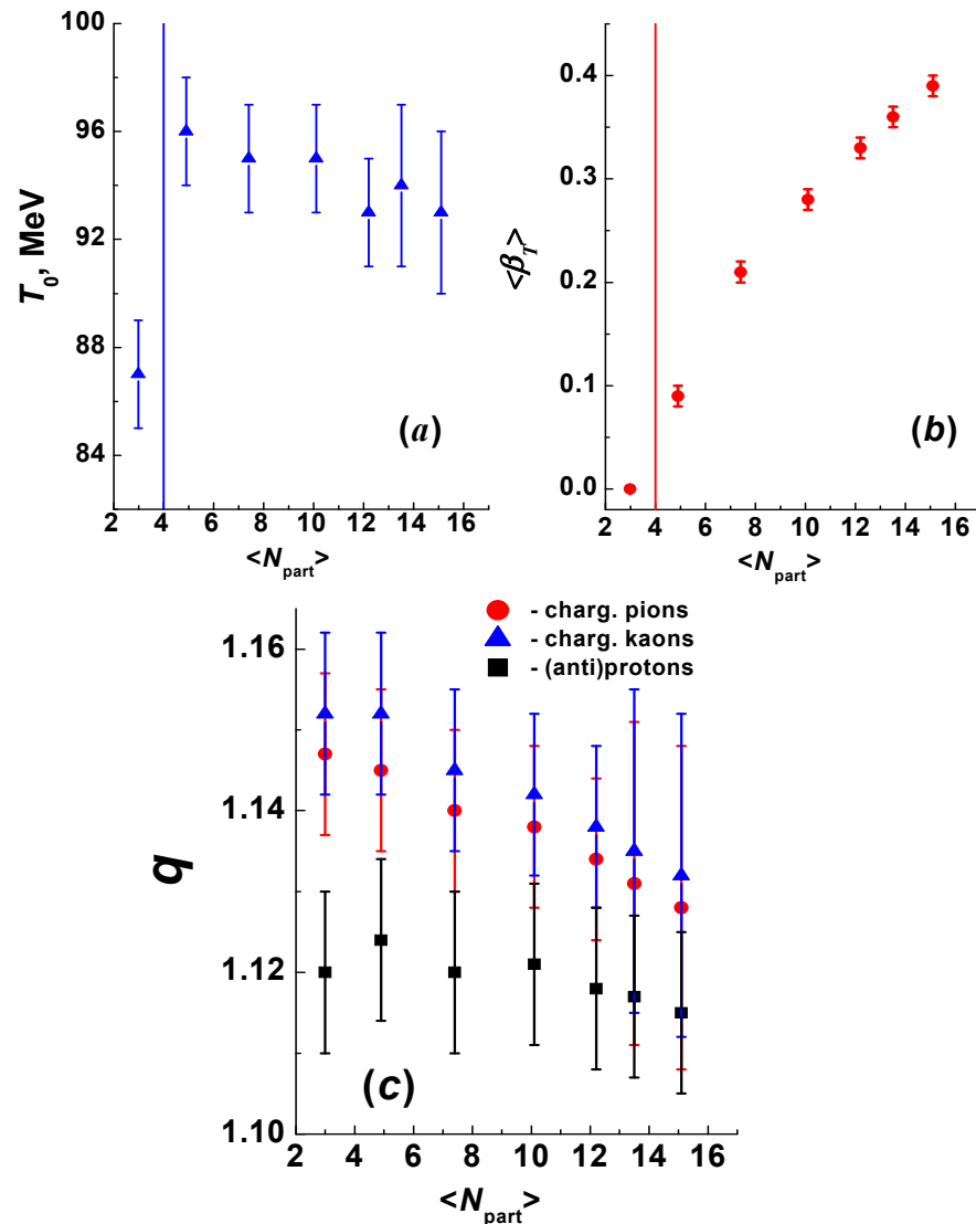
Figure 2. The dependencies of the obtained parameters T_0 (a), \langle \beta_T \rangle (b), and q (c) of the two-component model (THMTF) function (Equation (5)), given in Table 2, on the average number of participant nucleons ( \langle N_{part} \rangle ) in p +Pb collisions at \sqrt{s_{nn}} = 5.02 TeV. The vertical lines in panels (a) and (b).
