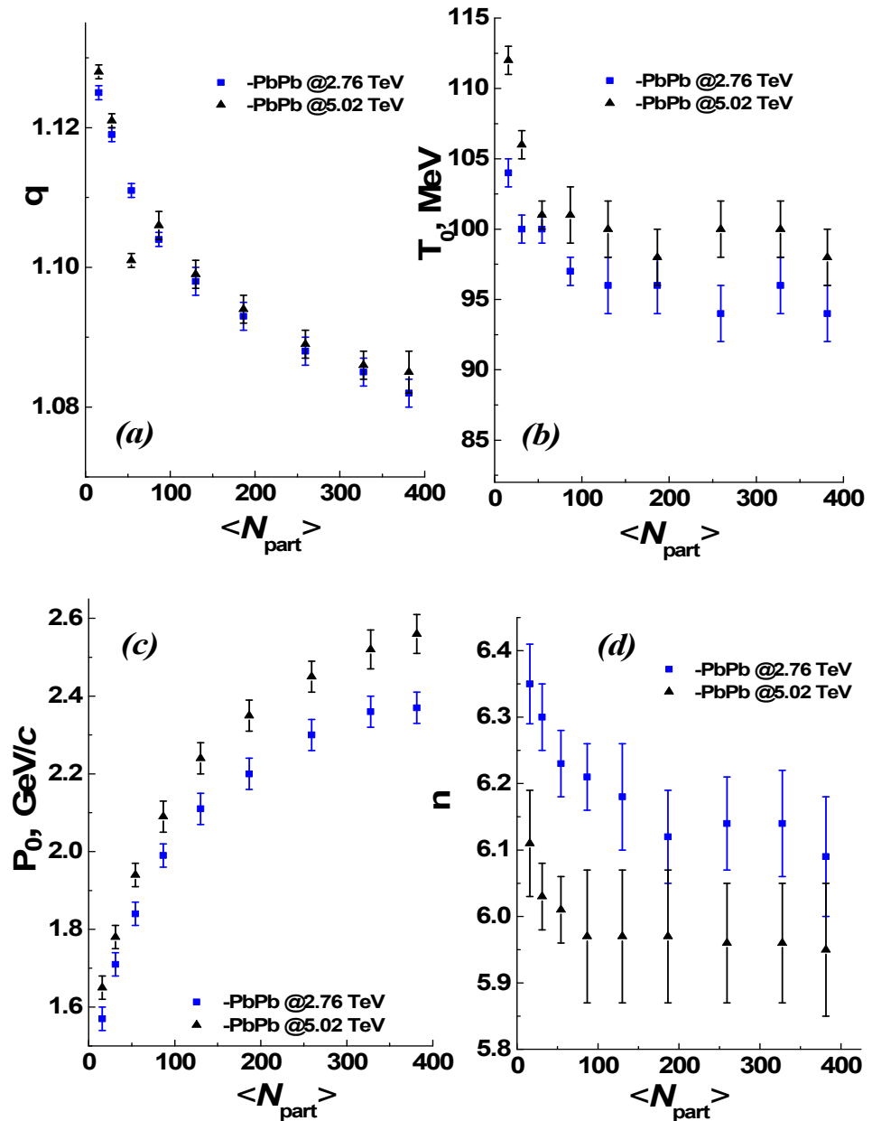
Figure 5. The dependencies of the parameters q (a), T_0 (b), P_0 (c), and n (d) on the average number of participant nucleons ( \langle N_{part} \rangle ), obtained in Ref. [50] from minimum \chi^2 fits with a two-component model (THMTF) function of the experimental transverse momentum spectra of the primary charged particles at nine centrality classes in Pb+Pb collisions at \sqrt{s_{nn}} = 2.76 and 5.02 TeV.
