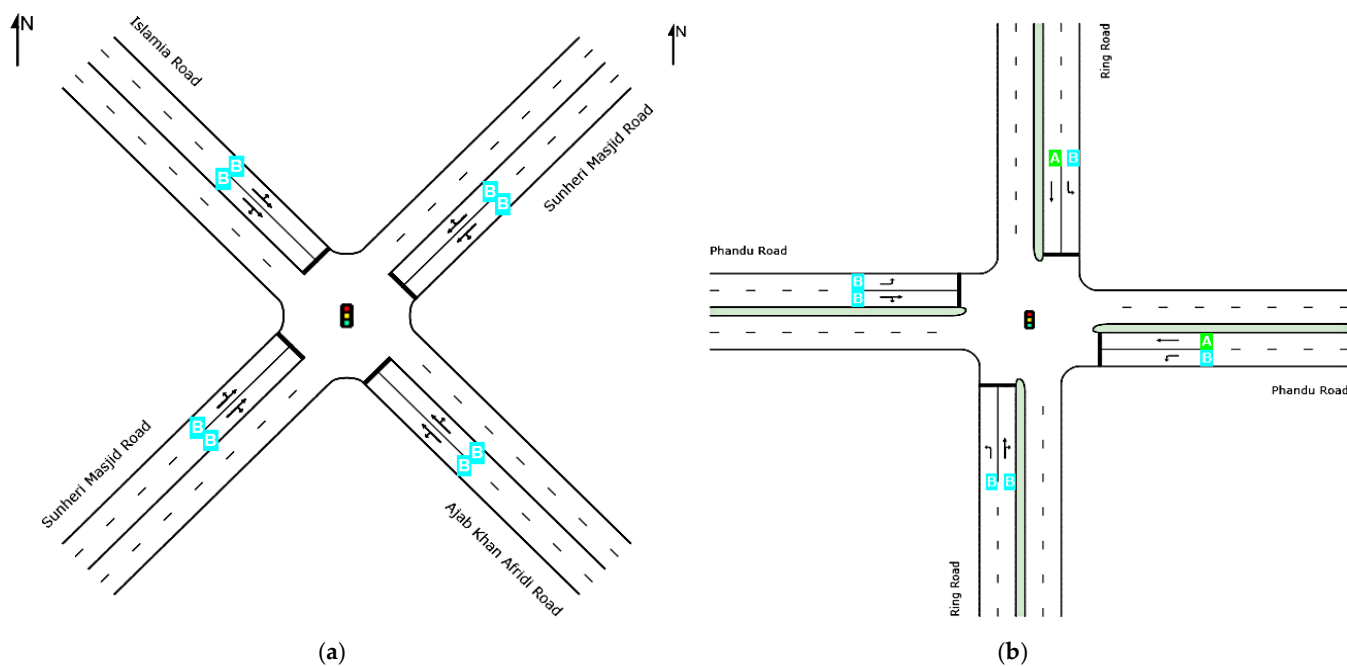
Figure 10. (a) Proposed Pre-Timed Signal Timings for FC Chowk. (b) Proposed Pre-Timed Signal Timings for Jameel Chowk.
