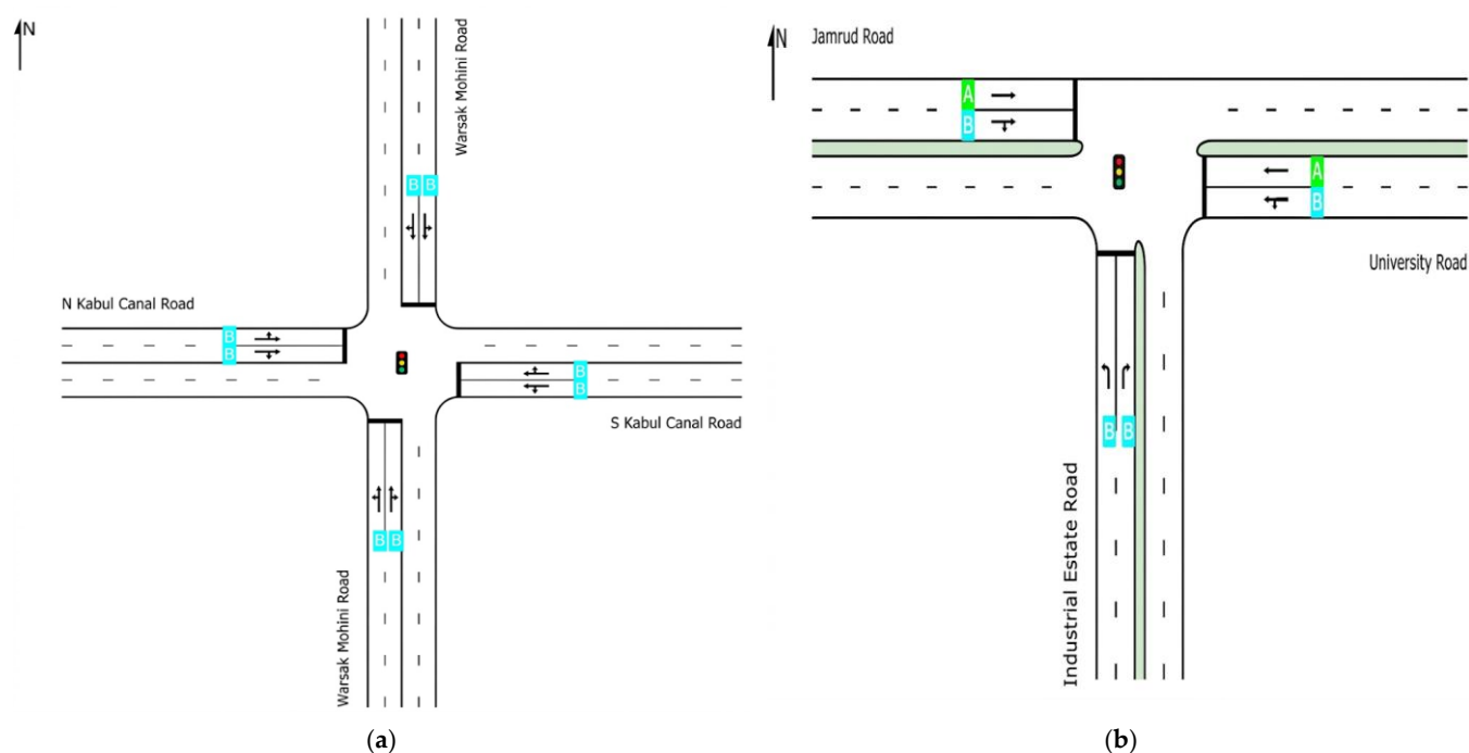
Figure 11. (a) Proposed Pre-Timed Signal Timings for Kababian Chowk. (b) Proposed Pre-Timed Signal Timings for Karkhano Chowk.
