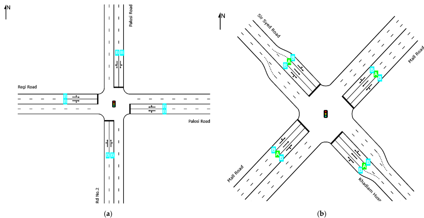
Figure 12. (a) Proposed Pre-Timed Signal Timings for Palosi Chowk. (b) Proposed Pre-Timed Signal Timings for Peshawar Services Chowk.
