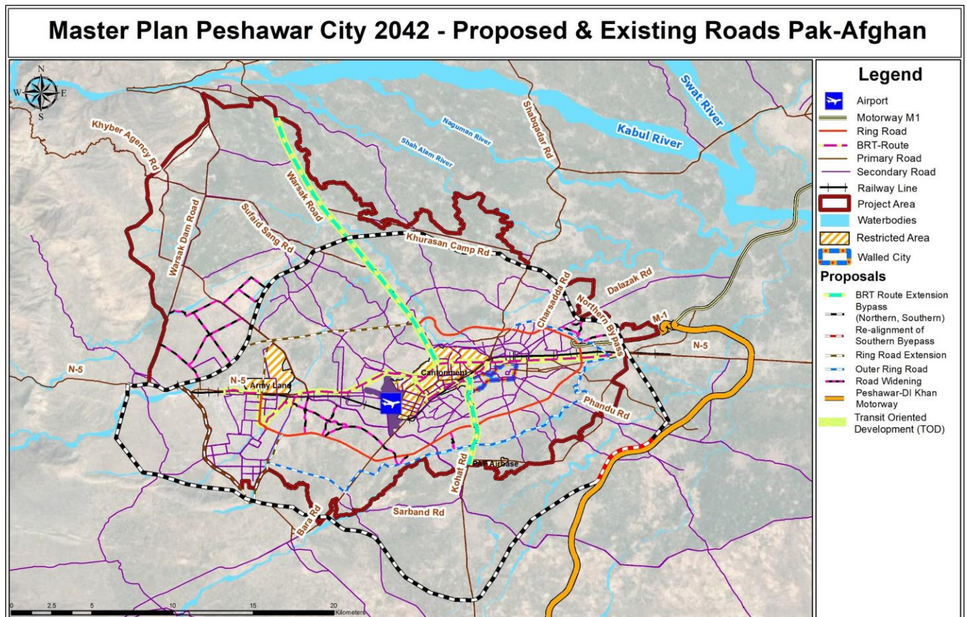
Figure 5. Proposed Roads and Widenings with Already Proposed Regional Connectivity (Northern and Southern Bypass—Pak-Afghan Corridor).
