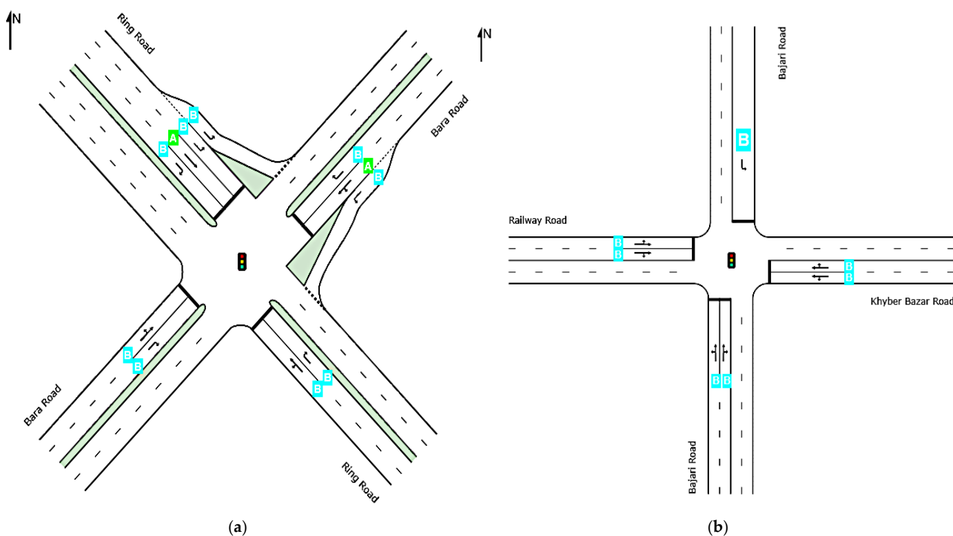
Figure 13. (a) Proposed Pre-Timed Signal Timings for Pistakhara Chowk. (b) Proposed Pre-Timed Signal Timings for Shuba Chowk intersection.
