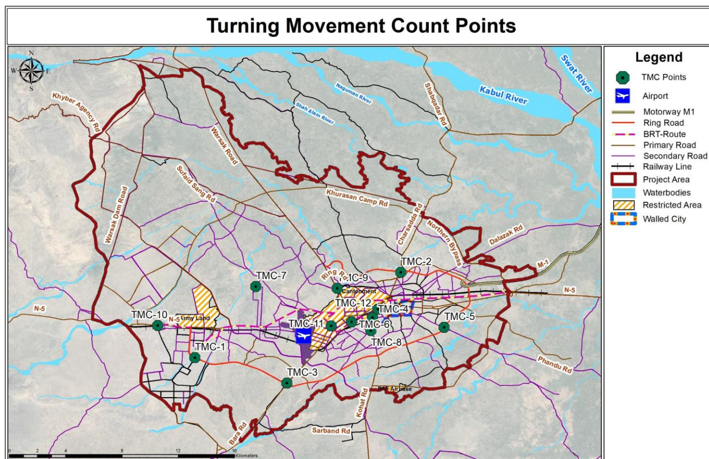
Figure 6. Turning Movement Count Points.
