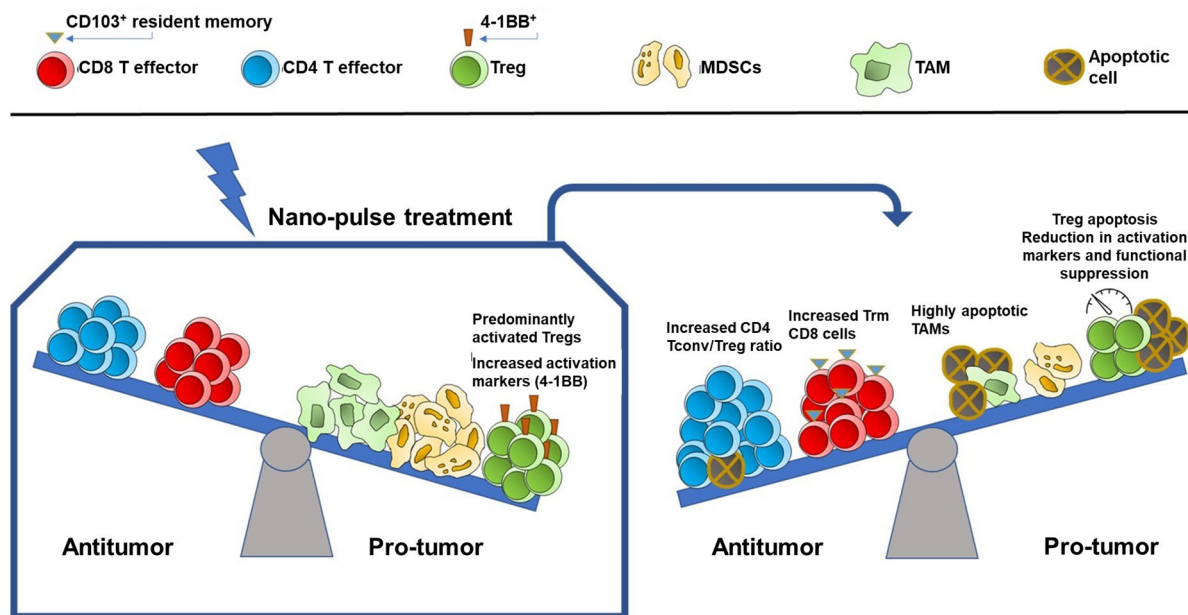
Figure 7. The impact of NPT on the TME in breast cancer. NPT shifts the immune cell dynamics from a pro-tumor to an antitumor environment. Suppressor cells, including Tregs, TAMs, and MDSCs, are diminished. Tregs undergo apoptosis, exhibit a shift from an activated 4-1BB + to a naïve 4-1BB − phenotype, and demonstrate reduced functional suppression capacity post-treatment. Antitumor CD4 Tconv and CD8 + CD103 + resident memory T cells increase in frequency.
