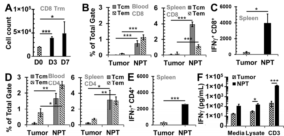
Figure 2. NPT elicits antitumor memory response. (A) Cell counts of CD8^+ Trms per million CD44^+ cells in dLNs. D0, D3, and D7: Days 0, 3, and 7. (B,D) CD8^+ (B) and CD4^+ (D) memory T cells in the blood and spleens of mice. Tcm: CD44^+CD62L^+ T cells; Tem: CD44^+CD62L^- T cells. (C,E) IFN-\gamma^+ CD8^+ (C) and CD4^+ (E) T cells from splenocytes after 6 h incubations with plate-bound anti-CD3. (F) IFN-\gamma product of splenocytes after 24 h incubation with tumor lysate. Groups: Tumor: untreated tumor-bearing mice, and NPT: NP-treated mice. Note: in B–F, tumor mice were at the end point for euthanasia (age 15–16 weeks), while NPT mice were euthanized post-treatment at 3 months (age 21–22 weeks). N = 3 –5. Error bars: SD. *: p < 0.05 , **: p < 0.01 , and ***: p < 0.001 (one-way ANOVA or t -test).
