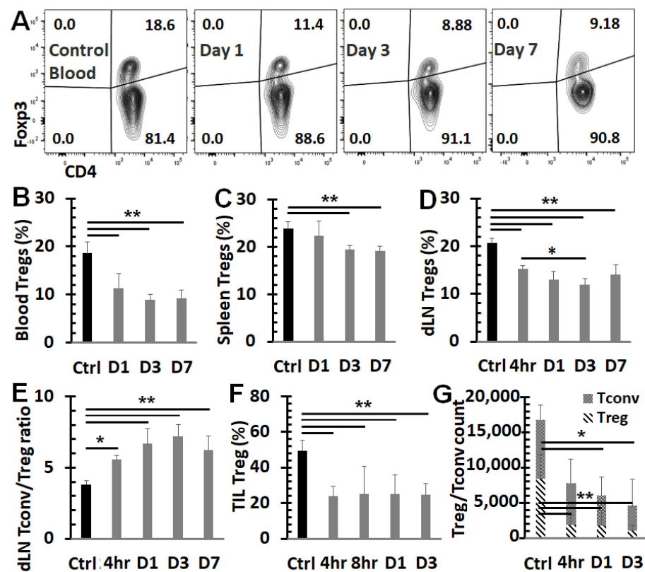
Figure 3. NPT reverses the Treg dominance locally and systemically. Breast tumors were established with an injection of 1 \times 10^6 4T1-luc cells into the posterior part of the mammary fat pad. The control group ( n = 4 ) received the tumor inoculation only. The remaining mice underwent NPT (100 ns pulses, 50 kV/cm, 3 Hz, 1000 pulses) on Day 11 following tumor inoculation. The treated mice were euthanized 4 h (4 h), 8 h (8 h), and on Day 1 (D1), Day 3 (D3), and Day 7 (D7) post-NPT. Their tumor tissues, tumor-draining lymph nodes (dLNs), blood, and spleens were harvested. Control tissues were obtained from mice with untreated tumors. (A) Summary flow plots represent Foxp3 + Tregs and Foxp3 - Tconv among the total CD4 + T cell population in the blood. (B–D) Quantitative bar graphs depict the percentage of Tregs among the CD4 + T cell population in blood (B), spleens (C), or dLNs (D). (E) The Tconv/Treg ratios dLNs. (F) TIL Tregs are represented in quantitative bar graphs as the percentage of Tregs among CD4 + TILs. (G) A standardized CD4 Treg vs. CD4 Tconv cell count. N = 4 per group. Error bars, SD. **: p < 0.01 and *: p < 0.05 (one-way ANOVA).
