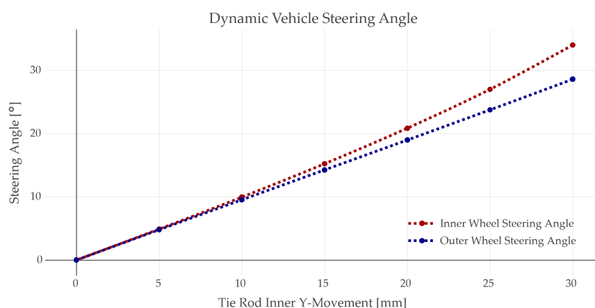
Figure 4. Vehicle steering characteristics.
