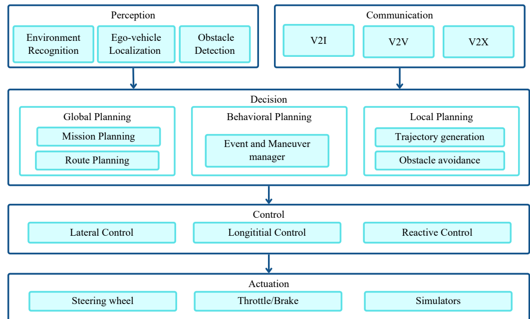
Figure 6. General architecture of an ADS within an AD/ADAS.
