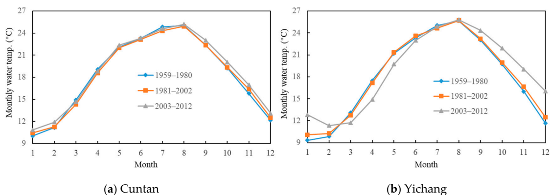
Figure 6. Impact of reservoirs on the monthly distribution of water temperature.
