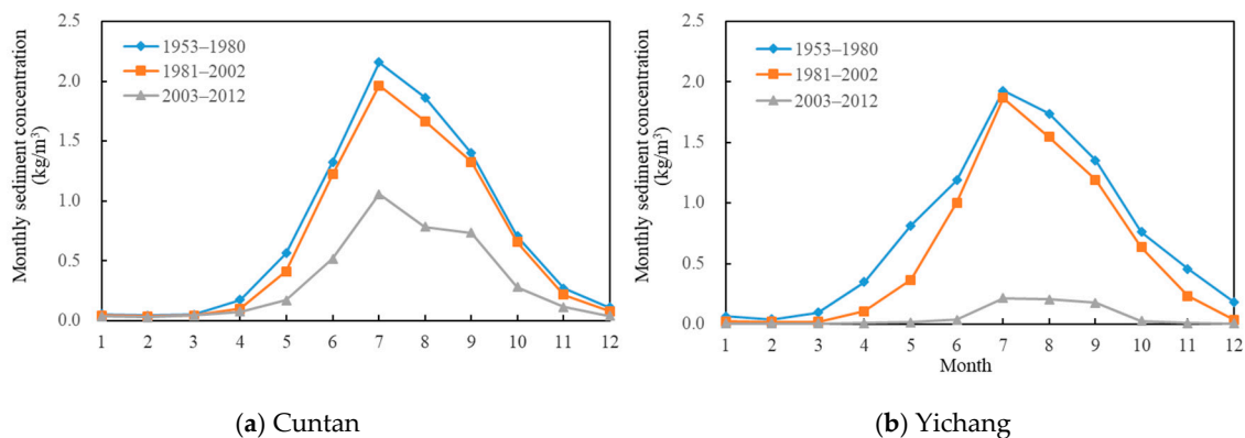
Figure 4. Impact of reservoirs on the monthly distribution of sediment concentration. Notes: the average monthly sediment concentration ( \text{kg/m}^3 ) was calculated using the average monthly sediment discharge ( \text{kg/s} ) divided by the average monthly flow discharge ( \text{m}^3/\text{s} ) according to the Code of Hydrologic Data Compilation [32].
