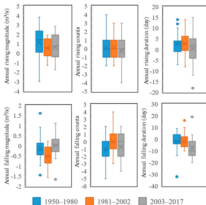
Figure 8. Boxplots of flow rising/falling characteristic difference between Yichang and Cuntan during May–June/October–November. The upper and lower parts of the boxes represent the 75th and 25th percentiles, respectively; the whiskers indicate the 90th and 10th percentiles; and the lines within the boxes are the median values.
