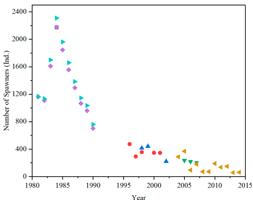
Figure 9. Temporal variations of adult CS population at the Gezhouba spawning site in the Yangtze River. Note: Blue square represents the data collected from Ke et al. [33], red dot from Wei et al. [34], blue triangle from Qiao et al. [35], green inverted triangle from Tao et al. [36], purple diamond from Huang et al. [37], left brown triangle from Wu et al. [38], right green triangle from Huang et al. [39].
