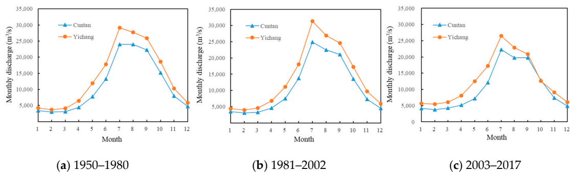
Figure 2. Impact of reservoir regulation on mean monthly discharge.
