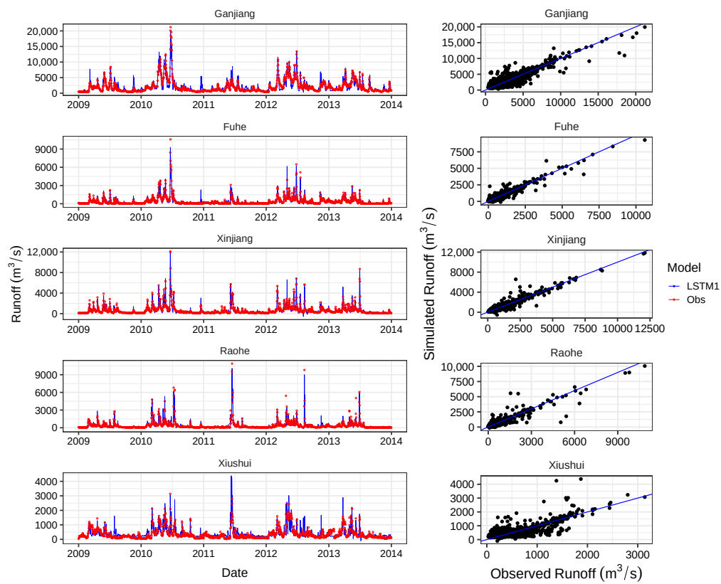
Figure 7. Performance of LSTM 1 during the validation period for all five sub-basins.
