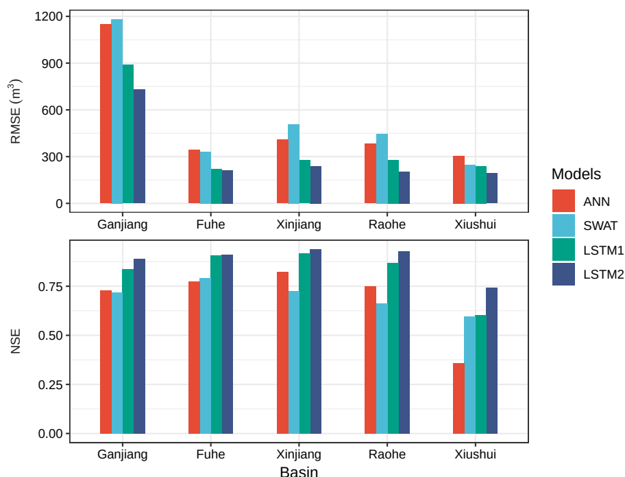
Figure 9. Performances of LSTMs, ANN and Soil & Water Assessment Tool (SWAT) model in simulating the runoff.
