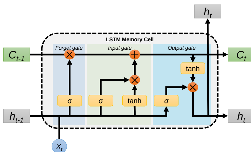
Figure 2. The architecture of Long Short Term Memory (LSTM) cell.
