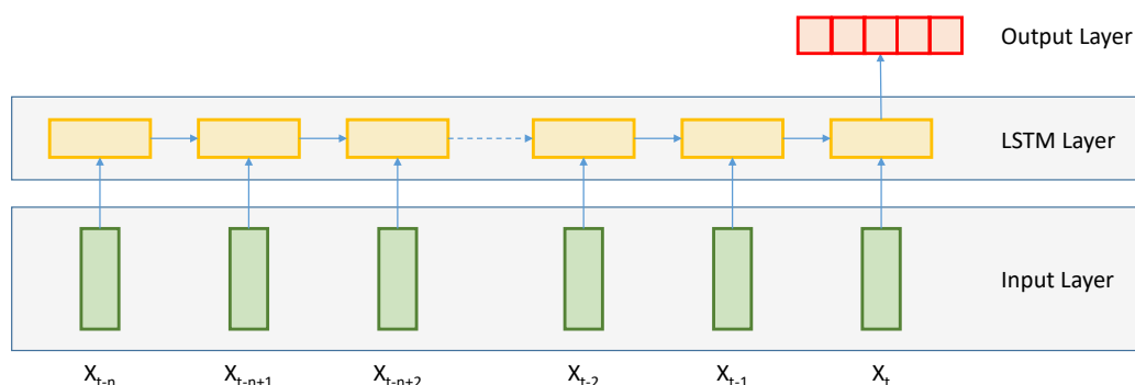
Figure 3. The architecture of the proposed LSTM model.
