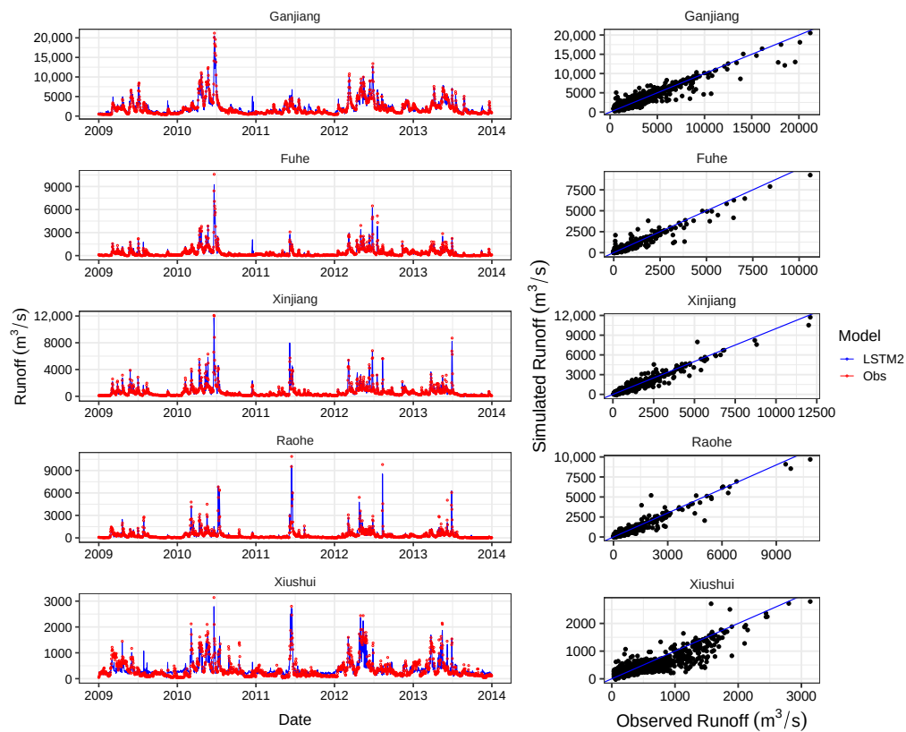
Figure 8. Performance of LSTM 2 during the validation period for all five sub-basins.
