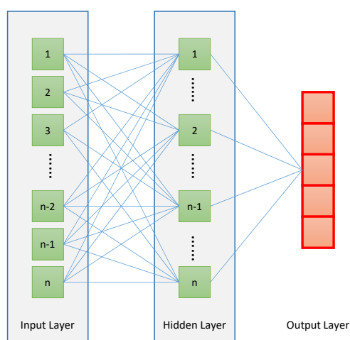
Figure 4. The architecture of the proposed Artificial Neural Network (ANN) model.
