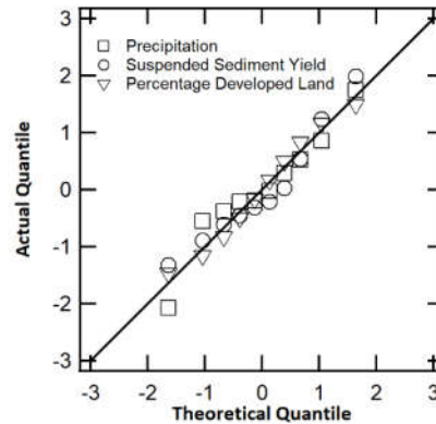
Figure 12. The Quantile–Quantile plot shows that variables are multivariate.
