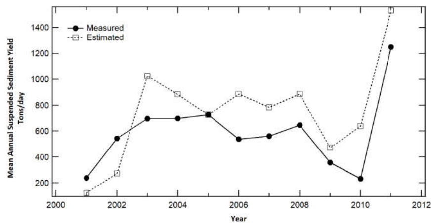
Figure 8. Comparison of estimated and measured suspended sediment yield.
