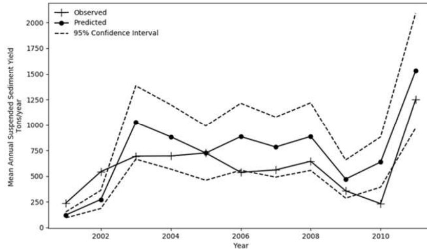
Figure 10. 95% Confidence interval for suspended sediment yield by MLR model.
