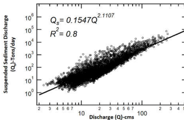
Figure 3. Suspended sediment rating curve created from data from 1950 to 2002 at the Independence stream gage.
