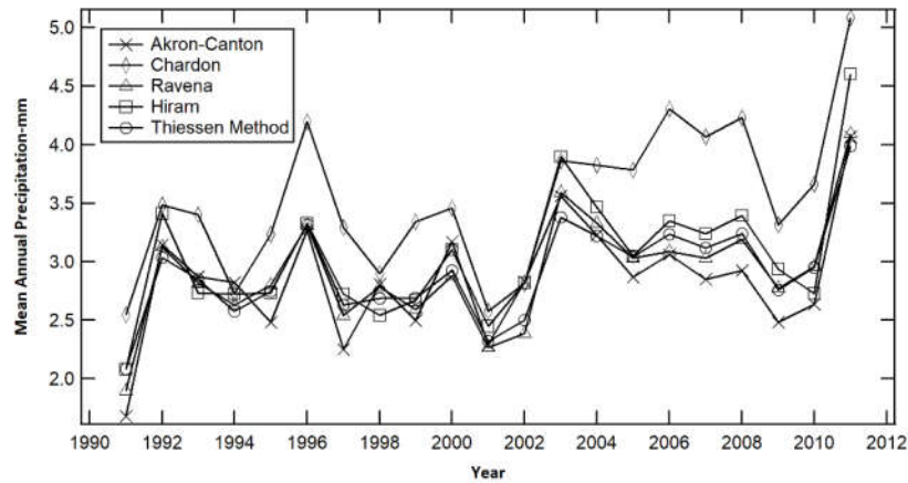
Figure 2. Mean annual precipitation measured across the watershed. The Thiessen method is used to estimate the average precipitation from the four gages.
