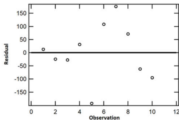
Figure 13. Residual plot confirms homoscedasticity assumption.
