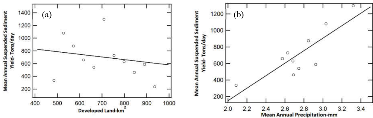
Figure 11. Relationship between (a) developed land area and mean annual suspended sediment yield, and (b) mean annual precipitation and mean annual suspended sediment yield.
