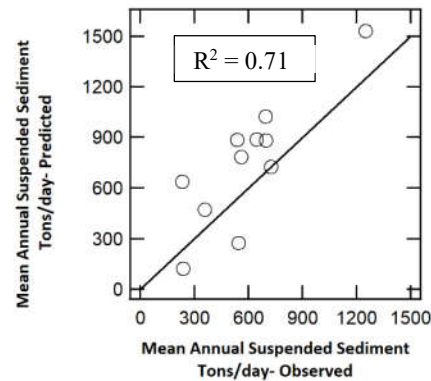
Figure 9. Observed and predicted suspended sediment yield.
