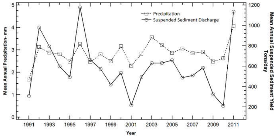
Figure 7. Variation in suspended sediment yield and precipitation.
