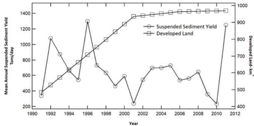
Figure 5. Variation in suspended sediment yield and land development.
