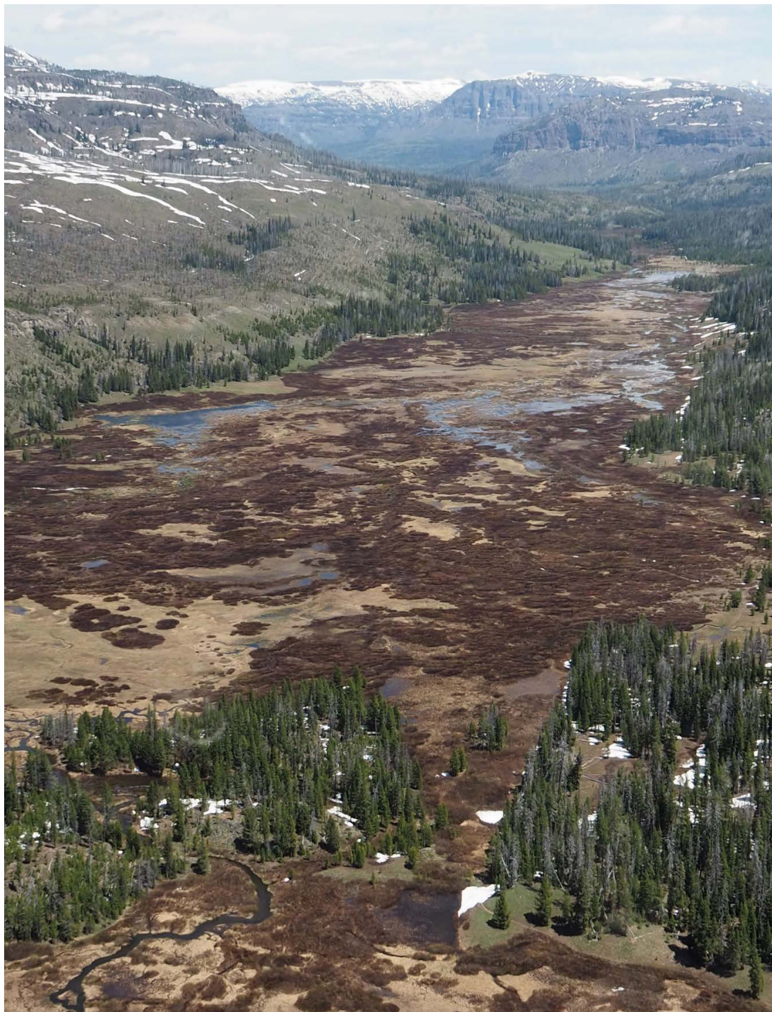
Figure A4. Two Ocean Pass partially flooded following snowmelt run-off in June 2018. Photo is looking east, with Pacific Creek in the foreground and with Atlantic Creek and the Thorofare region (Hawks Rest and the Trident Plateau) of the upper Yellowstone River system in the distance.
