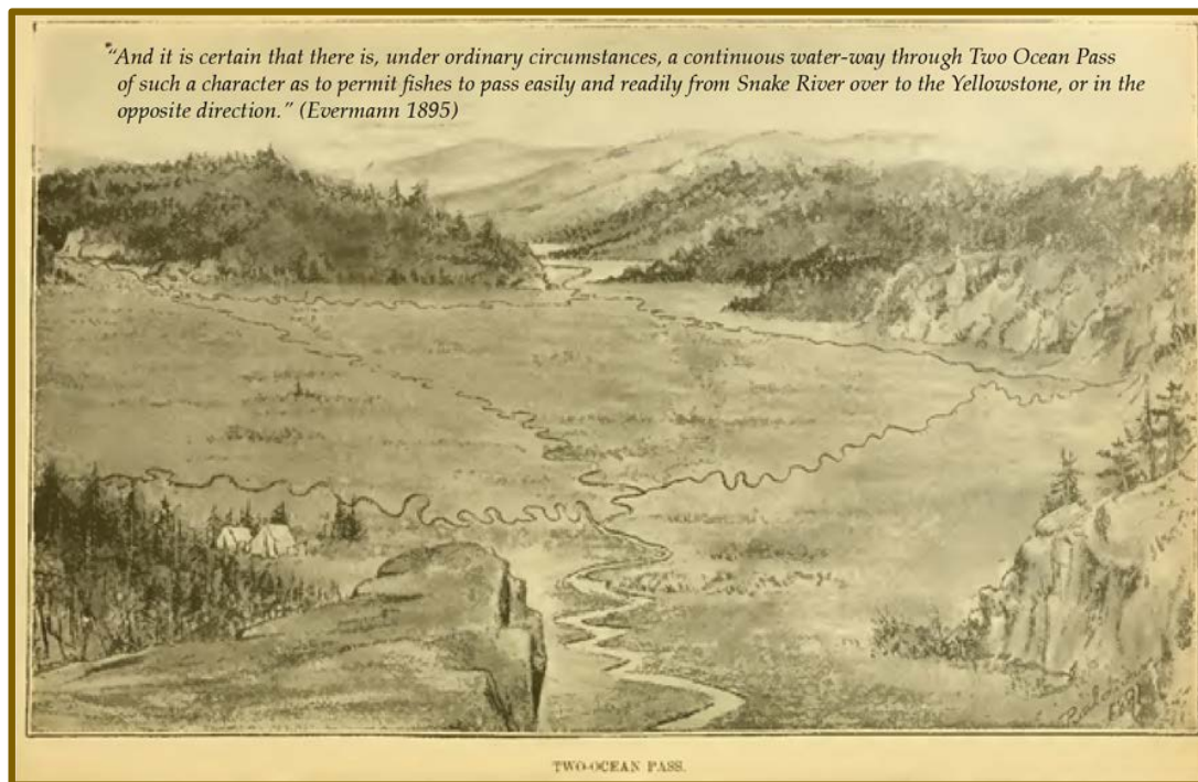
Figure 2. Sketch of Two Ocean Pass with a view to the northeast in 1891, recreated from [14,15]. Atlantic Creek is shown exiting the pass between the hills in the upper part of the image. Pacific Creek exits to the southwest in the lower part of the image. North Two Ocean Creek enters from the left side of the image and divides into its two distributaries. South Two Ocean Creek enters from the right of the image and apparently also divided into two distinct streams at that time. The pass is a nearly level meadow near the center, which is a marsh that becomes a small lake in times of wet weather or snowmelt runoff [14,15].
