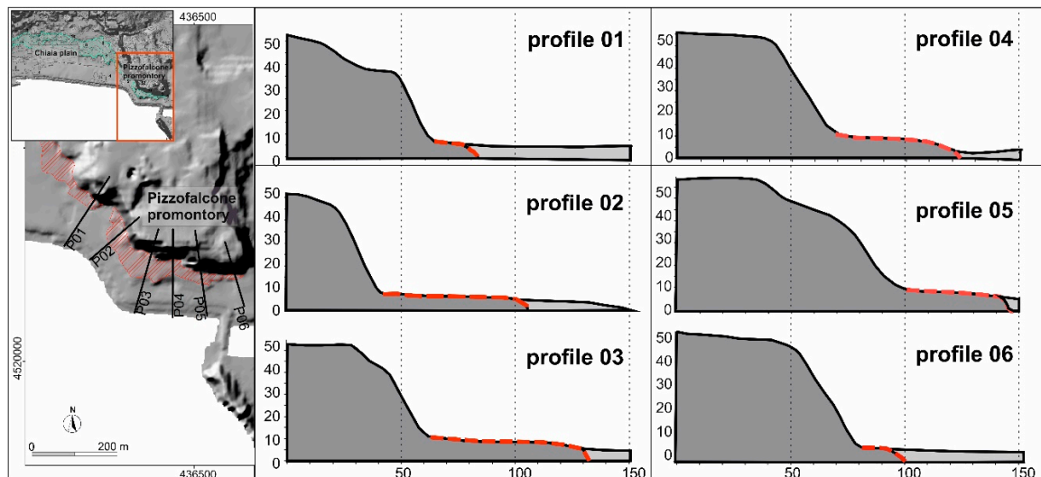
Figure 7. Six topographic profiles across the first-order platform (x and y axis are in metres): the black line is the present profile; the dotted red line is the original profile of the terrace and the light-grey area is the artificial anthropic infill built in the last 150 years. The green area in the inset map defines the perimeter of the 1st order platform and the red box represent the area in which the six profiles were reconstructed.
