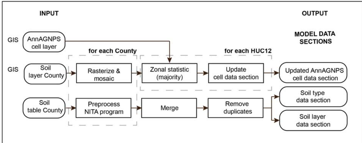
Figure S1. Schematic flowchart of the AnnAGNPS input soil data sections development.
