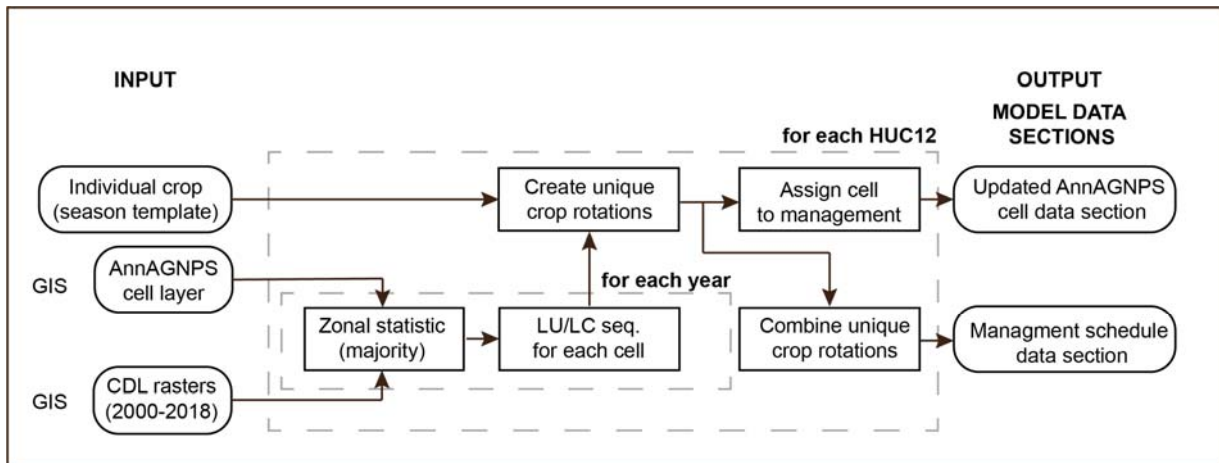
Figure S2. Schematic flowchart of the AnnAGNPS input management data section development.
