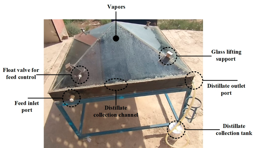
Figure 5. Pyramid shape solar still experimental setup.
