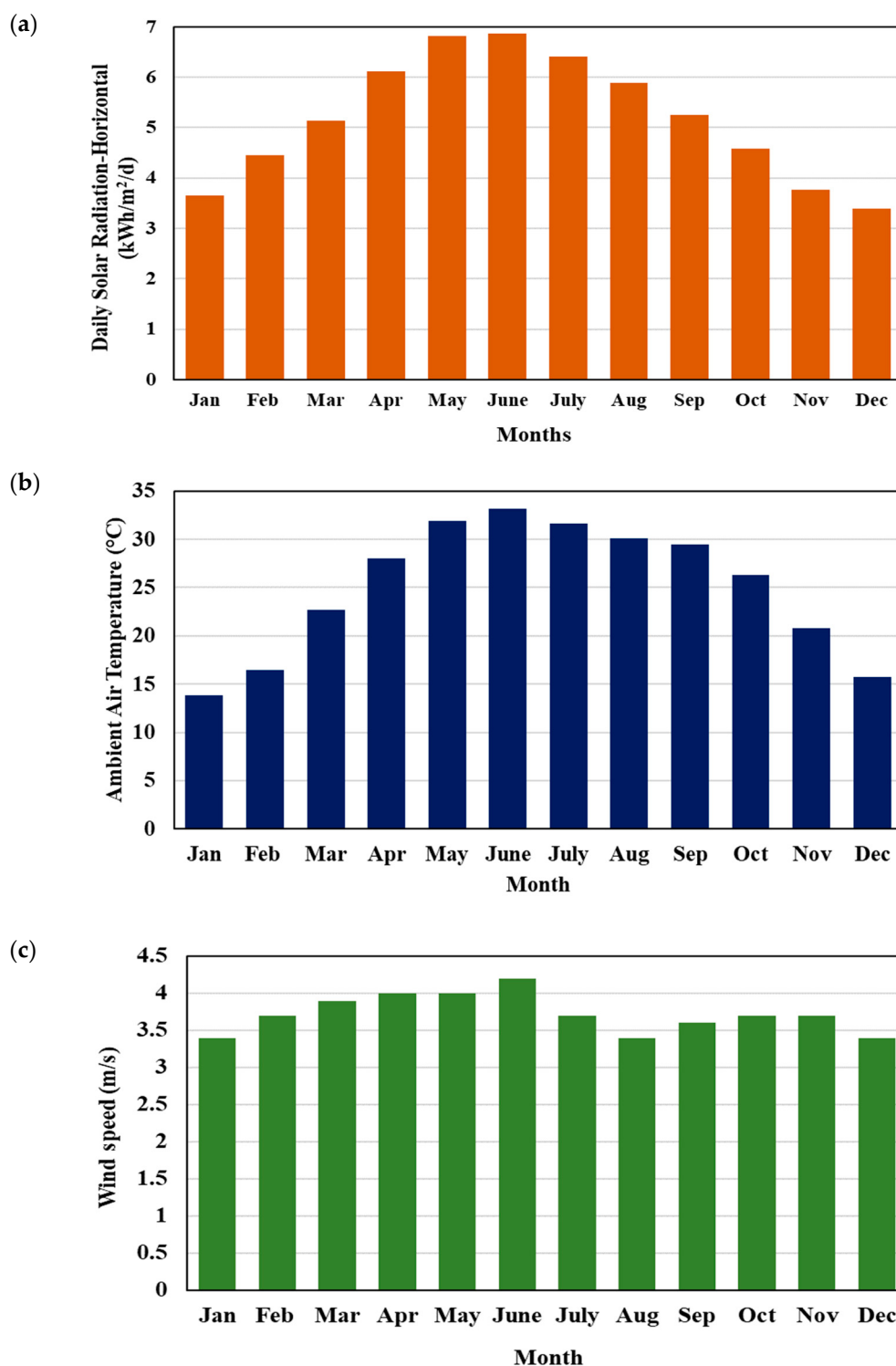
Figure 1. Monthly data for (a) daily solar radiation—horizontal, (b) ambient air temperature, and (c) wind speed [55].
