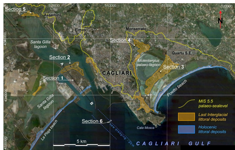
Figure 3. Aerial photograph of the coastal plain of Cagliari showing the main geomorphological features, yellow dashed line indicates the paleo high sea level of MIS 5.5 “Tirreniano”; the littoral deposits of the last interglacial (LI) and the Holocene shore deposits. Location of MIS5 stratigraphic sections: Section (1), geological profile crosses the container port for 4 km; Section (2), the north face of a large paleo barrier island of the MIS 5.5 of Sa Illetta in front of Santa Gilla lagoon [23]; Section (3), located in a quarry in the littoral paleo spit of Is Arenas; Section (4) and (5), marine terraces at the inner margin of the MIS5.5 transgression overlapping fluvial deposits of MIS 6; Section (6). MIS5 deposits intercepted from the dredging embankment at −16.5 m, 4 m below in the seabed.
