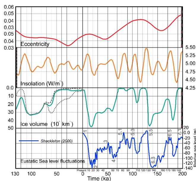
Figure 1. Long-term variations of eccentricity (top), June insolation at 65°N (middle), and simulated Northern Hemisphere ice volume (increasing downward) (bottom) for 200,000 years before the present to 130,000 from now. Time is negative in the past and positive in the future. In the Ice volume graphic for the future, three CO 2 scenarios were used: last glacial–interglacial values (green solid line), a human-induced concentration of 750 ppmv (grey dashed line), and a constant concentration of 210 ppmv (grey dotted line). In the Eustatic Sea level fluctuation graphic the gray numbers represent the Medium isotope stages. Simulation results from [9,10]; eccentricity and insolation from [11]. Figure modified from [10,12].
