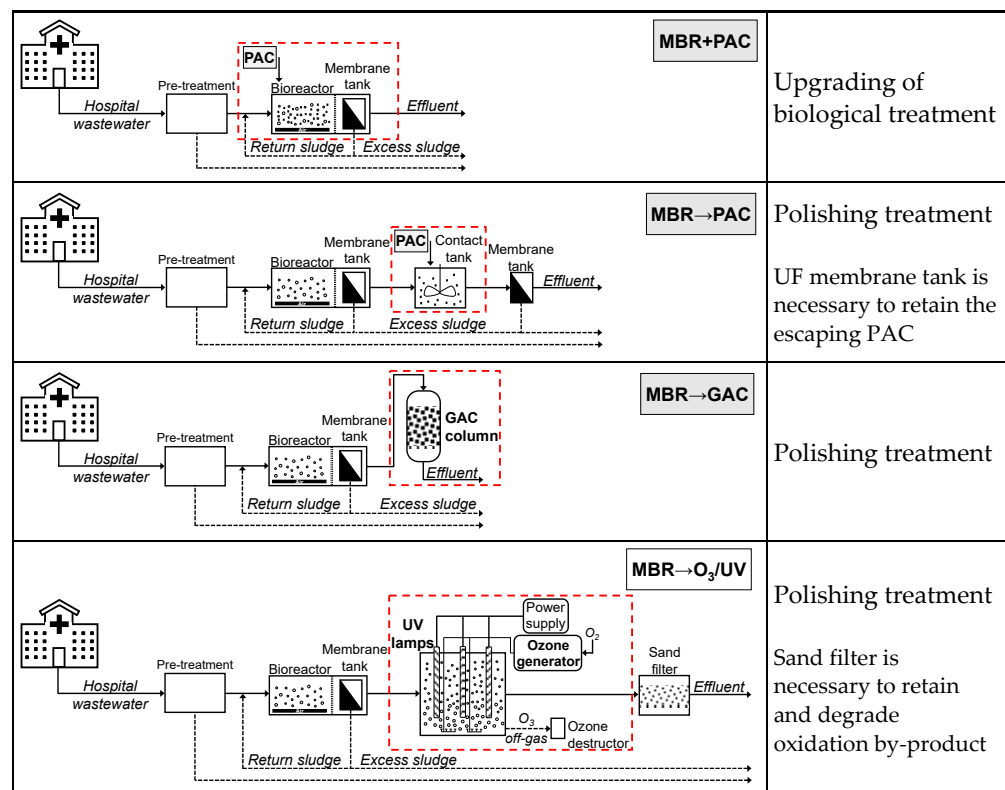
Figure 1. Typical configurations of a membrane bioreactor (MBR) combined with powdered (PAC) or granular (GAC) activated carbon and O 3 /UV. The treatment steps under study are surrounded by red dotted lines.
