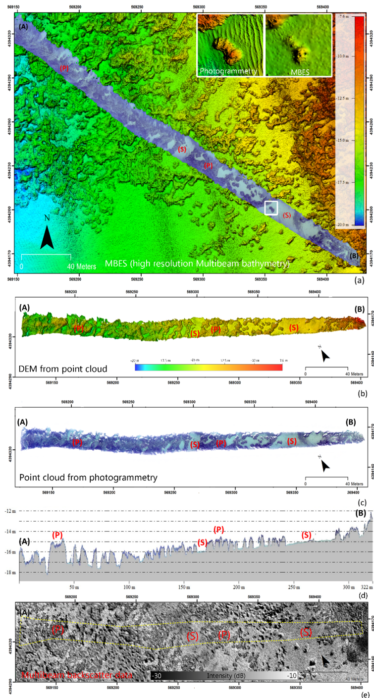
Figure 16. Bathymetric profile along the transect (AB) shows: (a) Co-registration of photogrammetric data from high-resolution (5 cm) multibeam bathymetry. (b) Very high-resolution DEM from point cloud. (c) RGB dense point cloud track line. (d) Bathymetric profile along the transect (AB) shows a comparison between the canopy height from photogrammetry and the DEM from high-resolution multibeam bathymetry. (e) Multibeam backscatter intensity map. The yellow dotted line indicates the area covered by the photogrammetric survey. (P: P. oceanica , S: sand).
