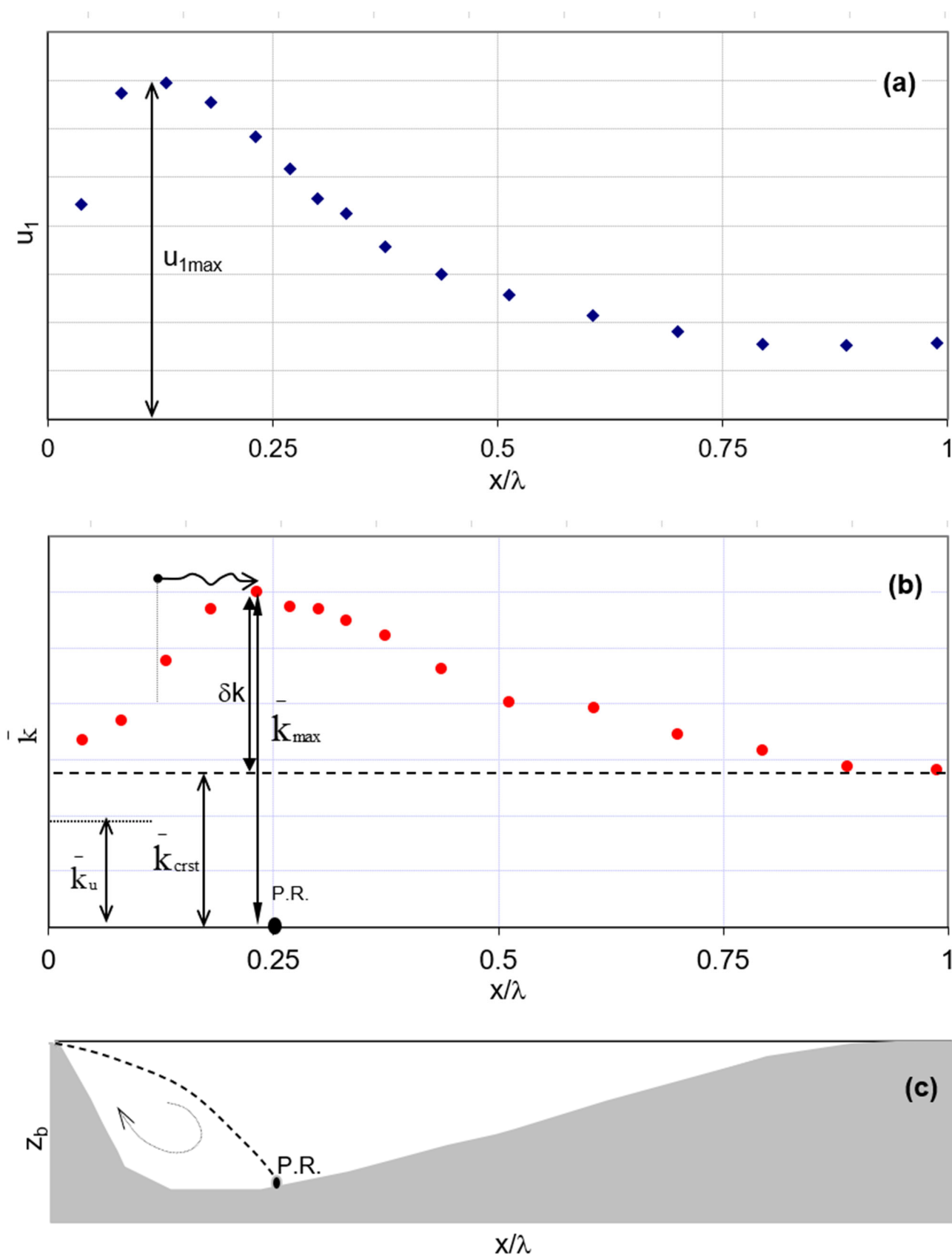
Figure 3. (a) A typical spatial variation for the integral velocity u_1 over one wavelength of a train of bedforms; (b) a typical variation for the depth-averaged turbulent kinetic energy, for fully developed turbulent flow; (c) bed geometry of one wavelength for a train of dunes.
