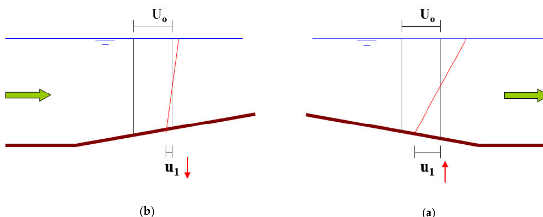
Figure 2. Variation in Moment Velocity Scale u_1 for Accelerating and Decelerating Flow. (a) Decelerating Flow, (b) Accelerating Flow.
