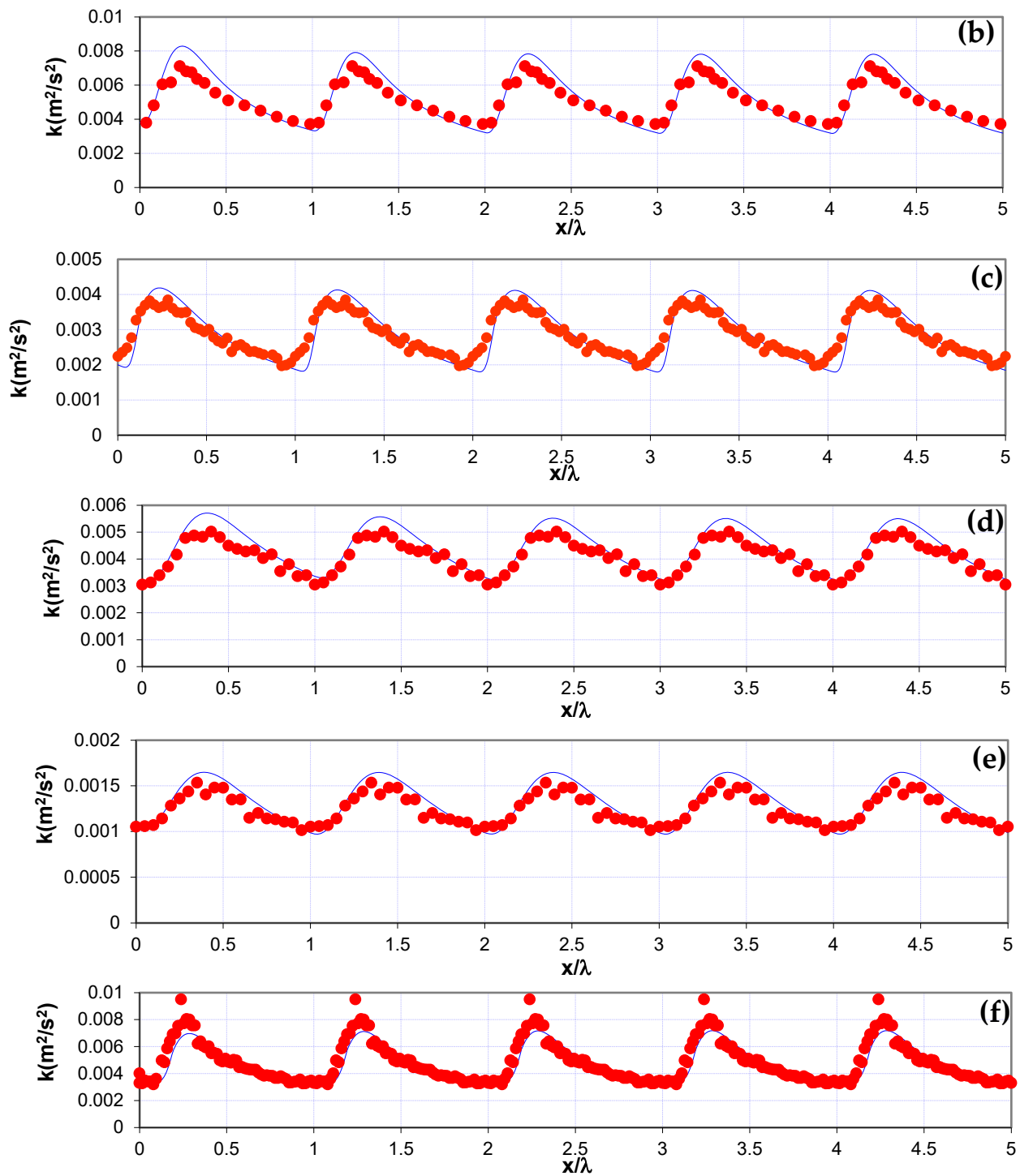
Figure 10. Depth-averaged predictions of MDAKE model using \zeta_k = 0.013 (solid line). Solid circles represent data of: (a) experiment T5, (b) experiment T6, (c) Run2, (d) Run4, (e) Run5, (f) experiment by Bennett and Best.
