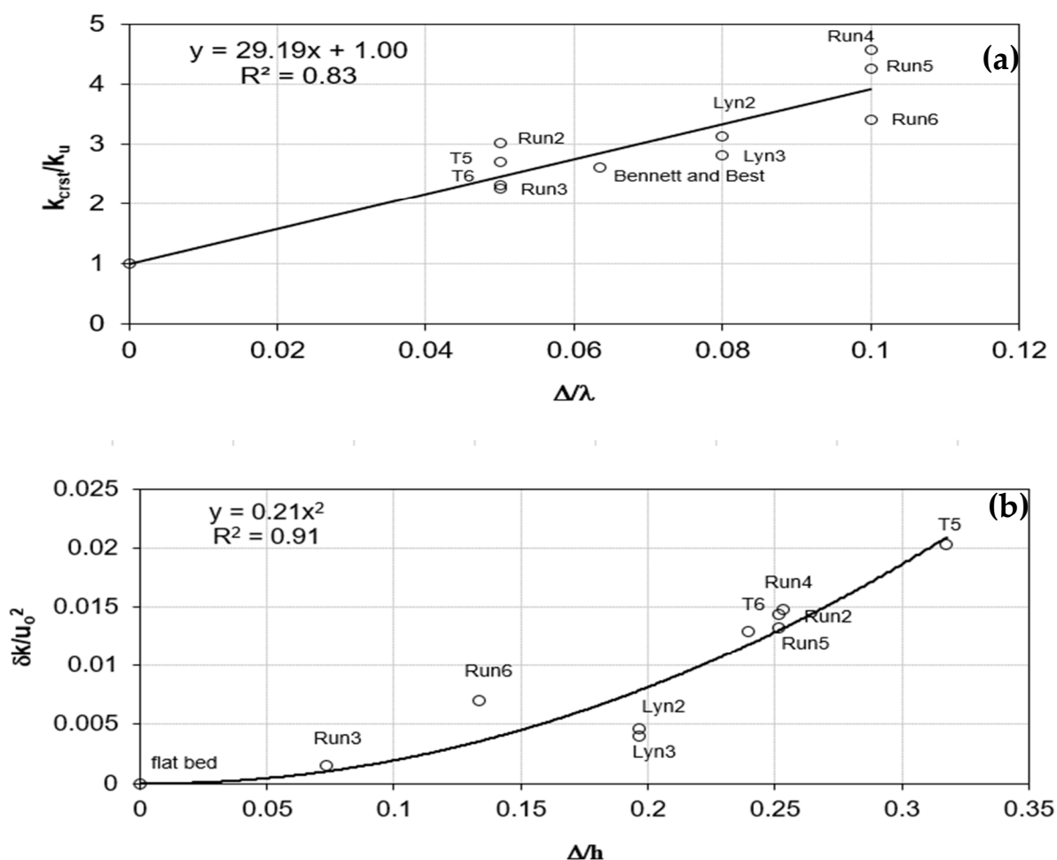
Figure 8. (a) Effect of bedform height on the equilibrium value of the depth-averaged turbulent kinetic energy over the crest. (b) Effect of bedform height on the net increase in the depth-averaged turbulent kinetic energy, \delta k , over bedforms (refer to Figure 3 for definitions).
