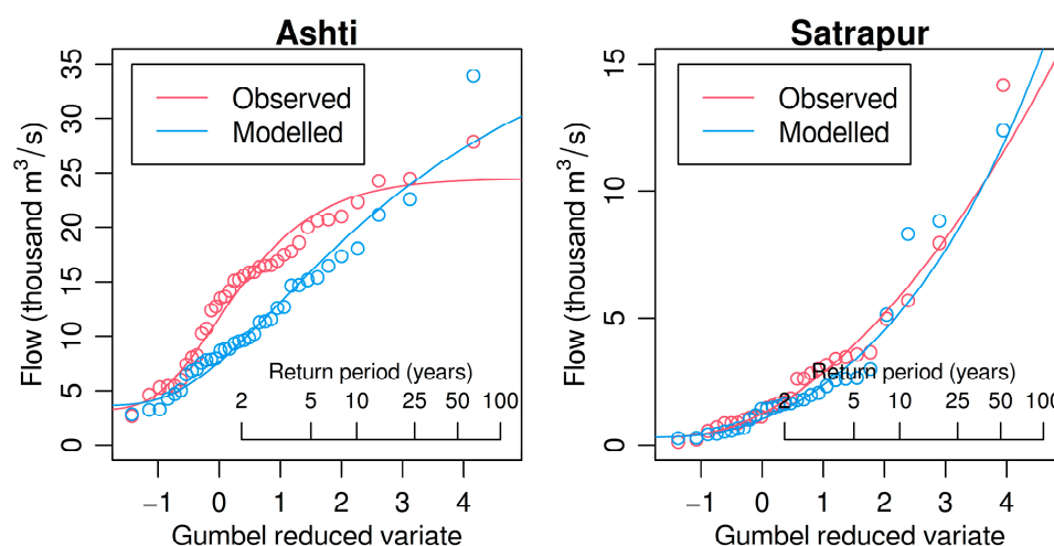
Figure 10. Observed and modeled flood frequency curves for Ashti and Satrapur (semi-lumped modeling).
