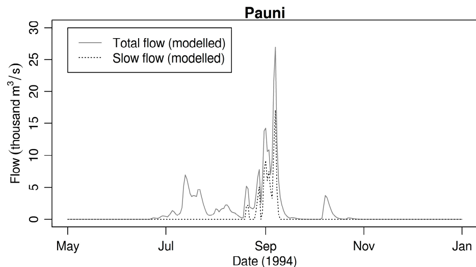
Figure 6. Modeled total flow and slow flow for Pauni, May–December 1994.
