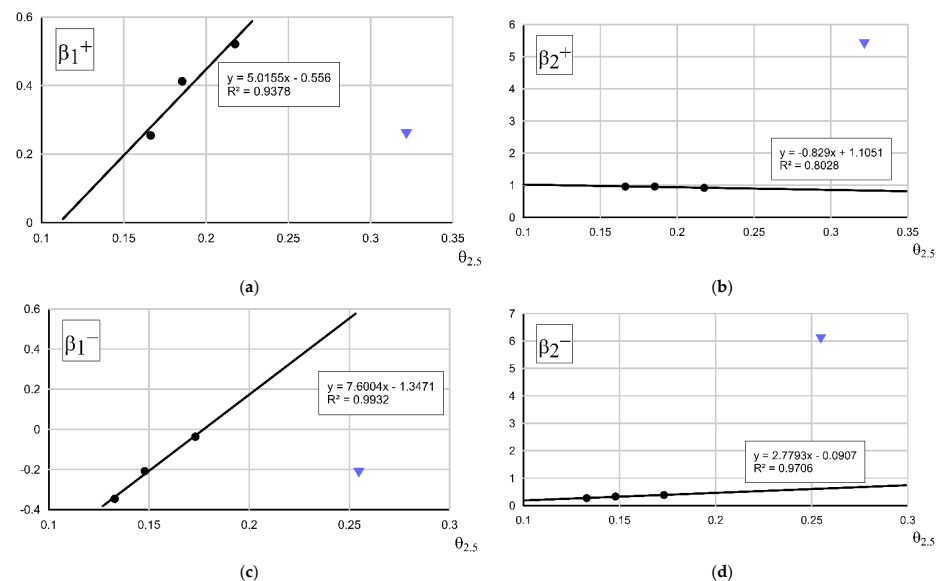
Figure 6. Plots of sediment flux correction factors over a sloping seabed: (a) fine fractions, crest phase; (b) coarse fractions, crest phase; (c) fine fractions, trough phase; (d) coarse fractions, trough phase.
