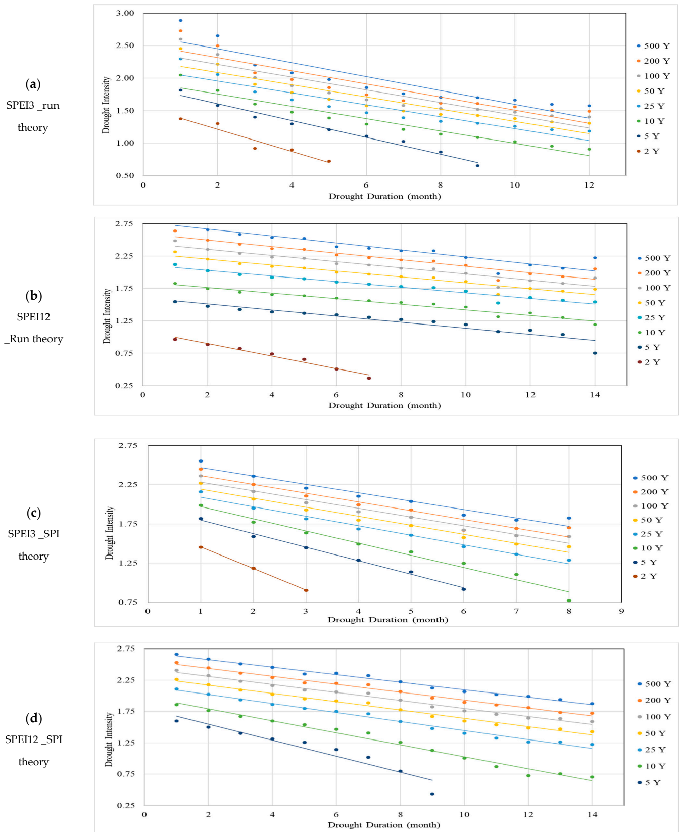
Figure 5. Resulting IDF curves using SPEI for both run and SPI theories for 3- and 12-month timescales: (a) IDF using SPEI3 based on run theory. (b) IDF using SPEI12 based on run theory. (c) IDF using SPEI3 based on SPI theory. (d) IDF using SPEI12 based on SPI theory.
