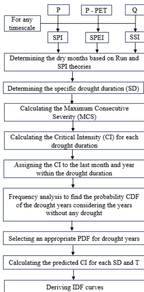
Figure 3. Methodological approach.
