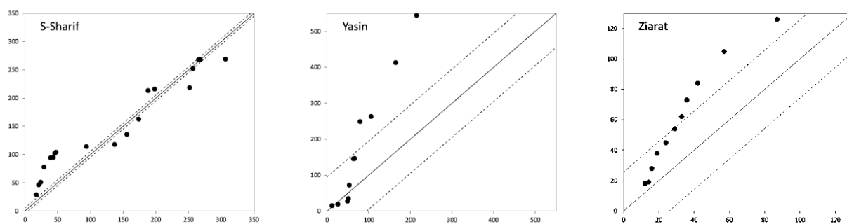
Figure A6. Results of R95p at 12 stations, obtained by using the ITA method.
