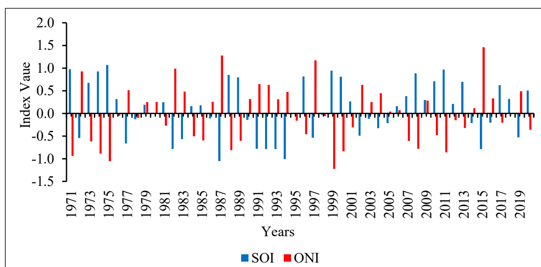
Figure 10. Comparison of SOI vs. ONI.
