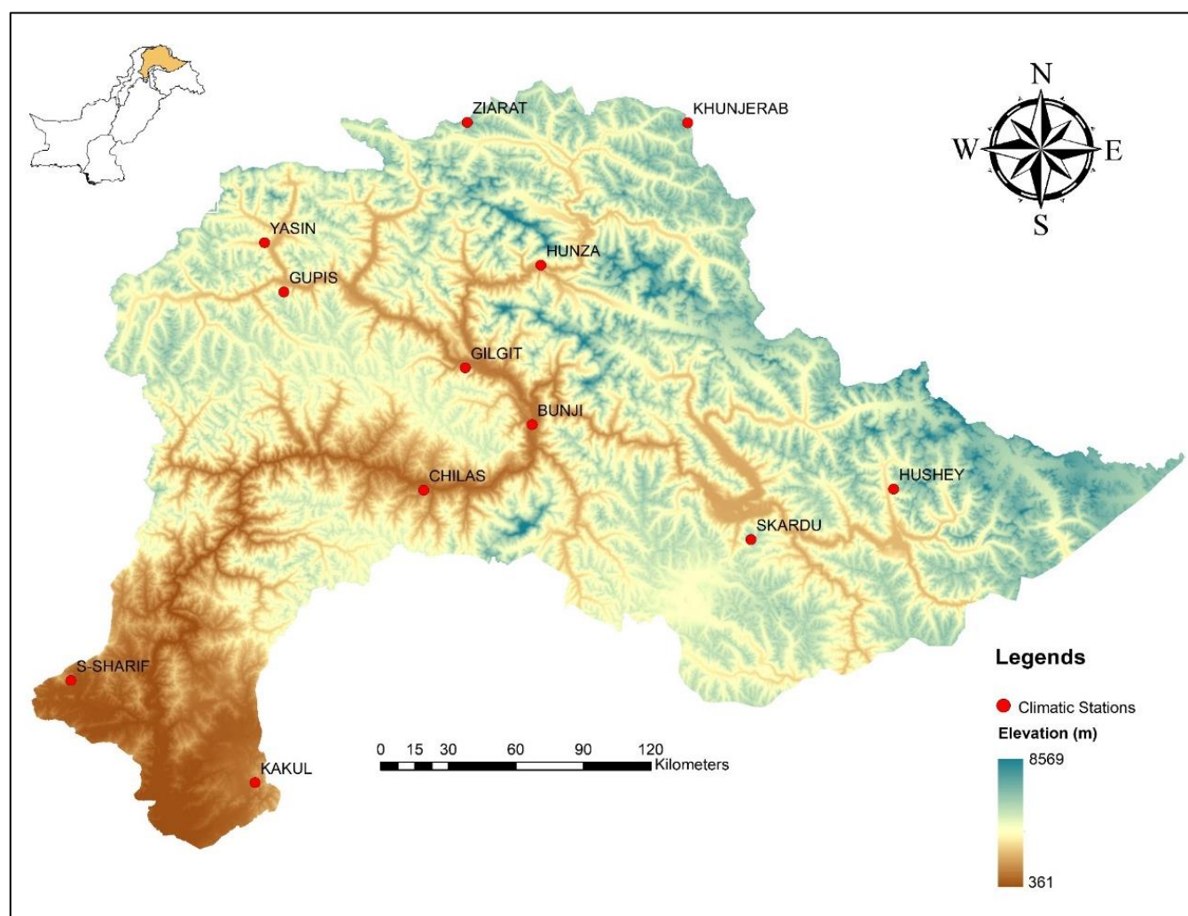
Figure 1. Study area (Upper Indus Basin) with climatic stations and elevation data.
