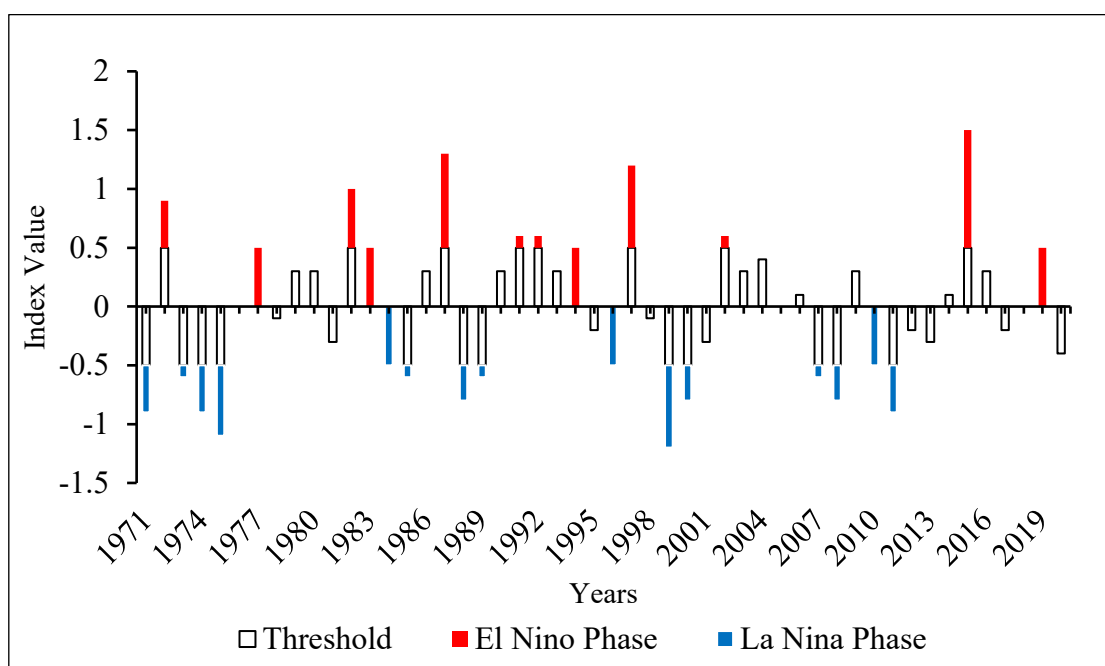
Figure 13. ENSO phases in ONI in the 1971–2020 period.
