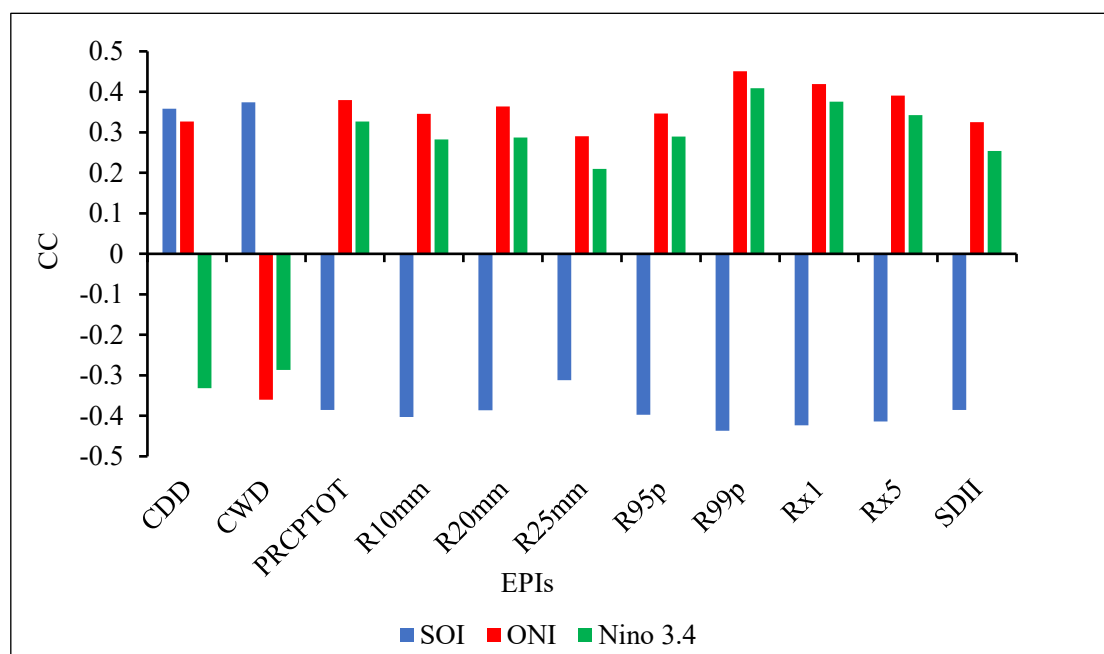
Figure 20. Overall correlation of ENSO with EPIs.
