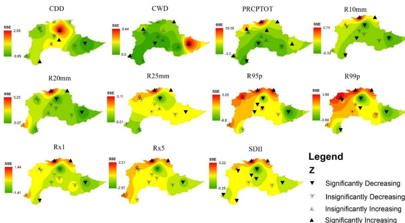
Figure 8. Spatial patterns of extreme precipitation indices in the Upper Indus Basin.
