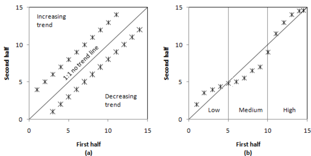
Figure 3. Representation of ITA graph and its components. (a) No trend, datasets, (b) upward and downward trend, datasets.
