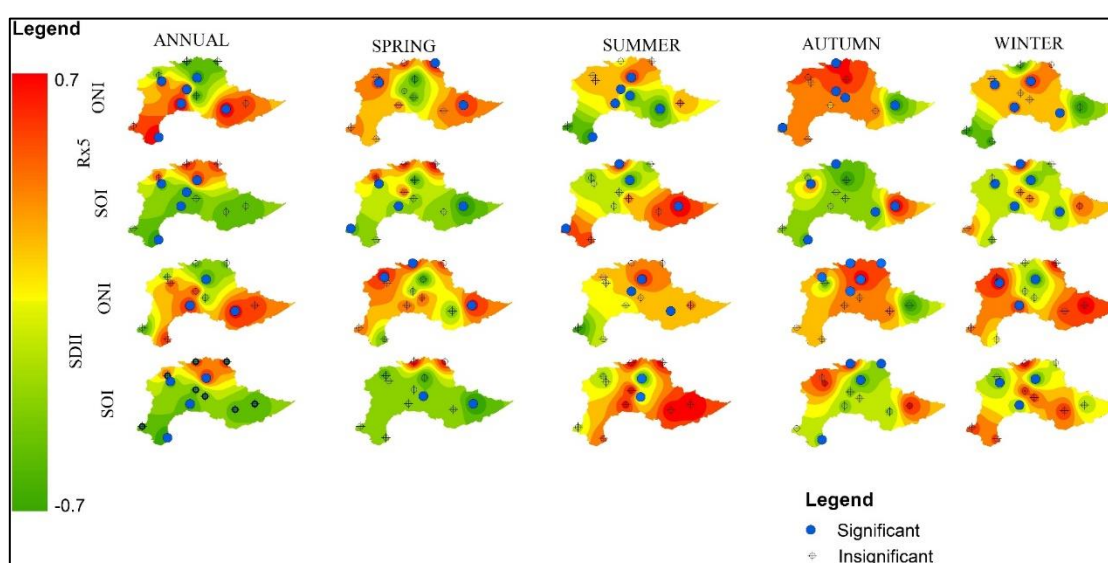
Figure 19. Spatial patterns of ENSO correlations with EPIs (SDII, Rx5).
