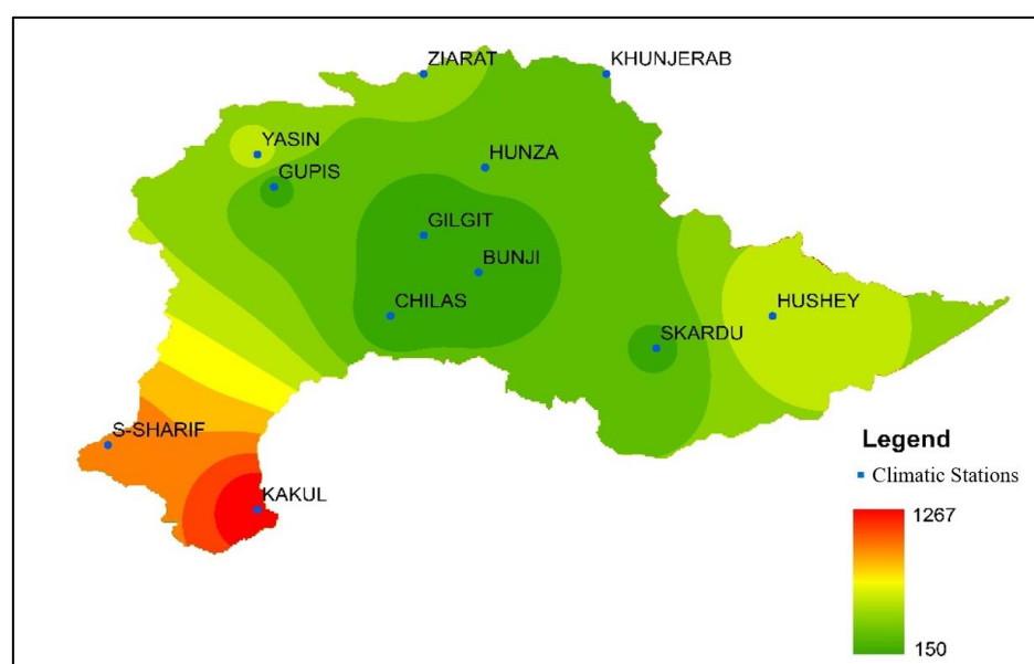
Figure 5. Spatial mean annual variation (mm).
