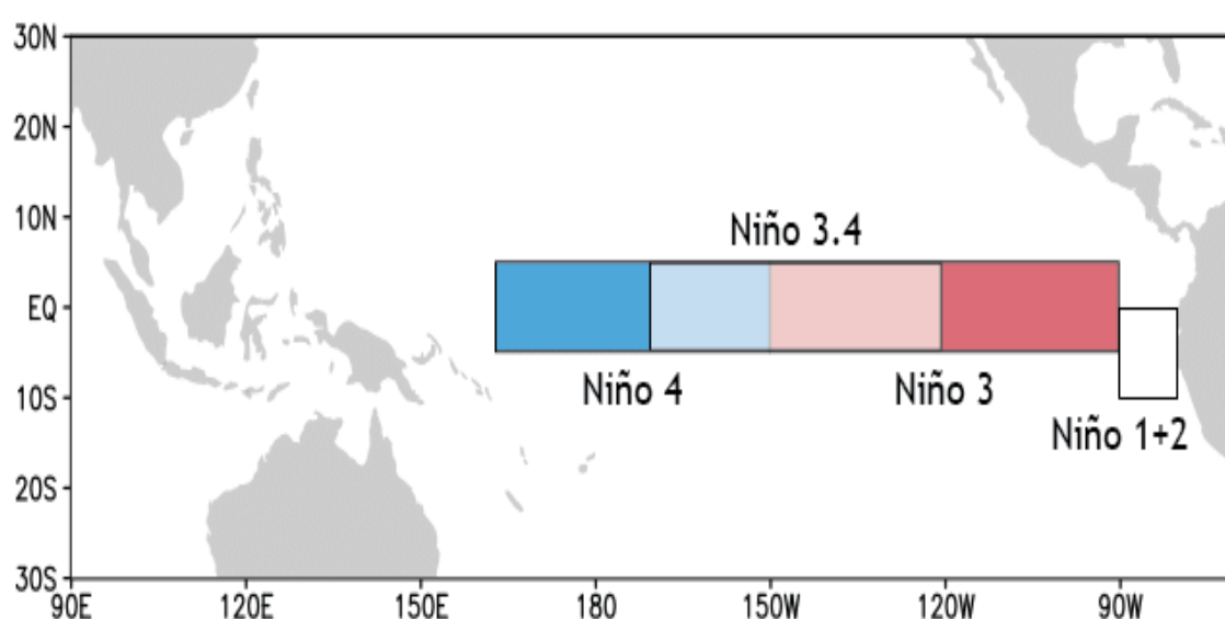
Figure 4. Sea surface temperature regions in the Pacific Ocean.
