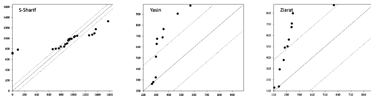
Figure A2. Results of PRCPTOT at 12 stations, obtained by using the ITA method.
