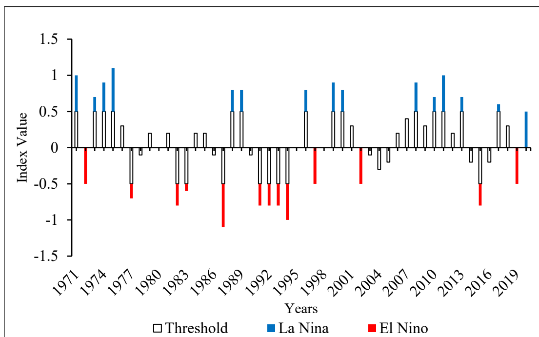
Figure 12. ENSO phases in SOI in the 1971–2020 period.
