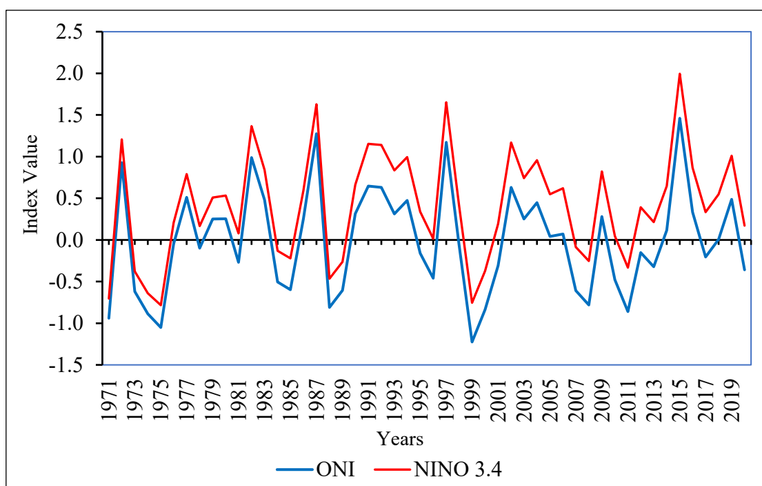
Figure 11. Comparison of ONI vs. NINO 3.4.
