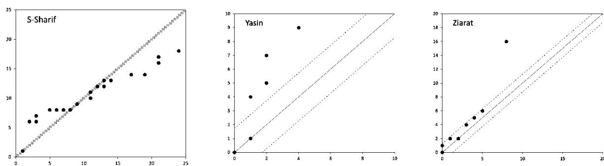
Figure A5. Results of R25mm at 12 stations, obtained by using the ITA method.
