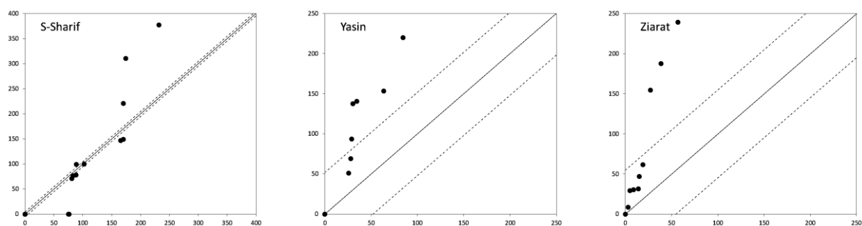
Figure A7. Results of R99p at 12 stations, obtained by using the ITA method.
