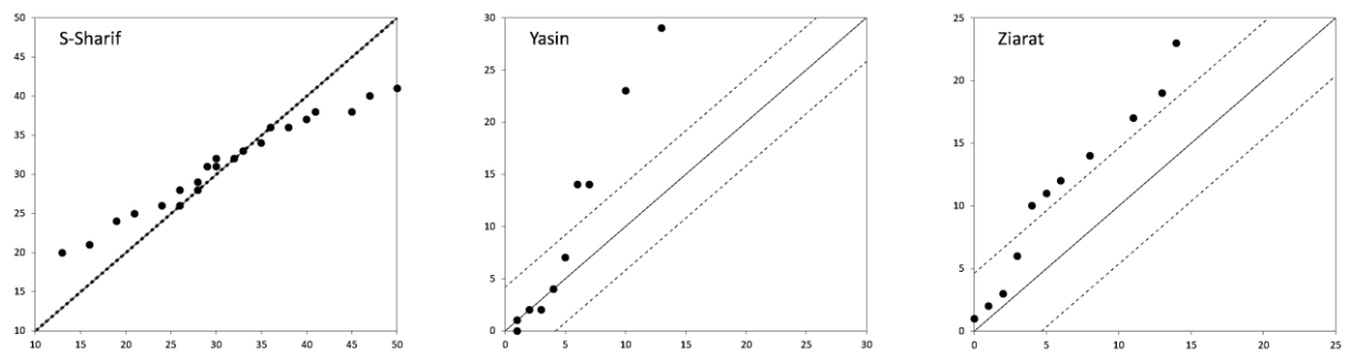
Figure A3. Results of R10mm at 12 stations, obtained by using the ITA method.
