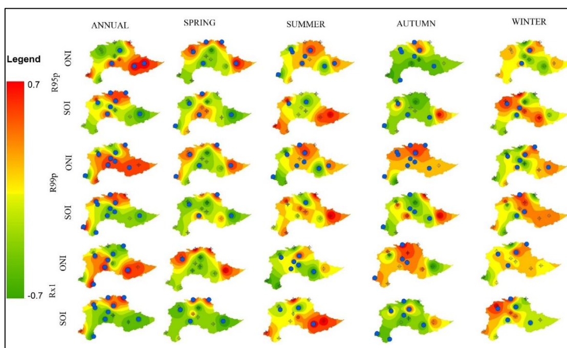
Figure 18. Spatial patterns of ENSO correlations with EPIs (Rx1, R99p and R95p).
