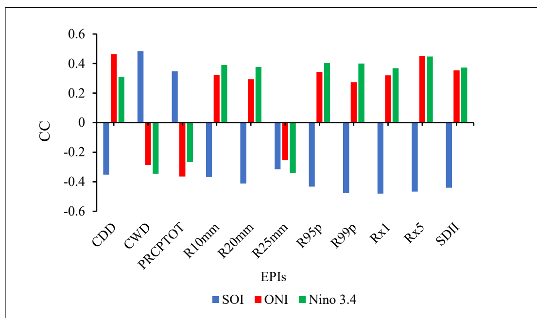
Figure 21. Highly elevated stations' correlations of ENSO with EPIs.
