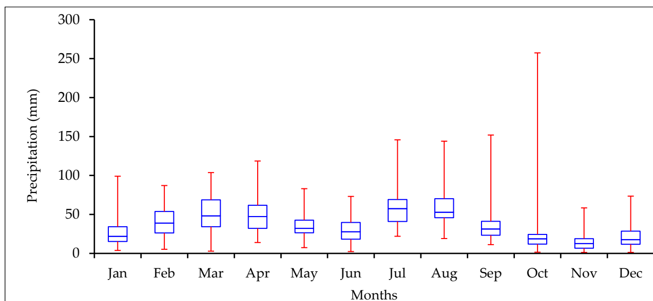
Figure 7. Temporal mean monthly variation.
