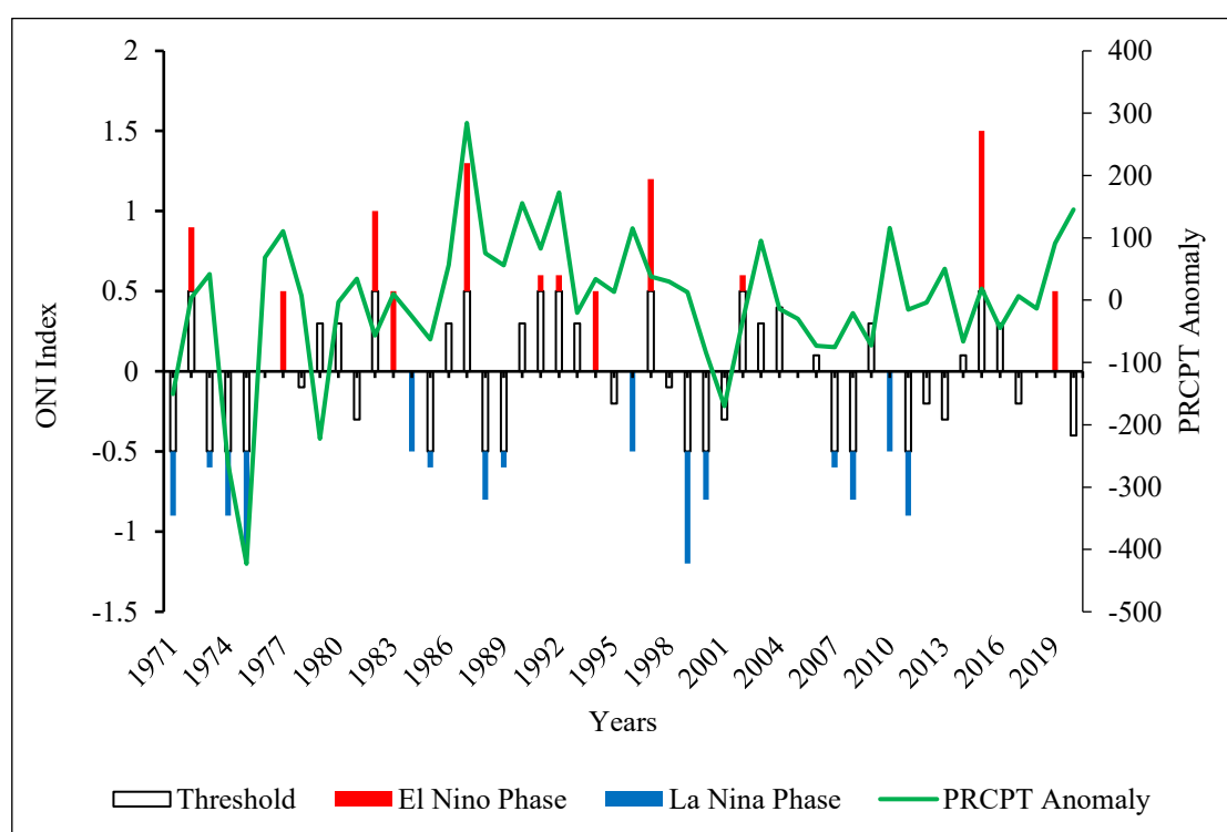
Figure 15. Precipitation in UIB during ENSO phases of ONI.
