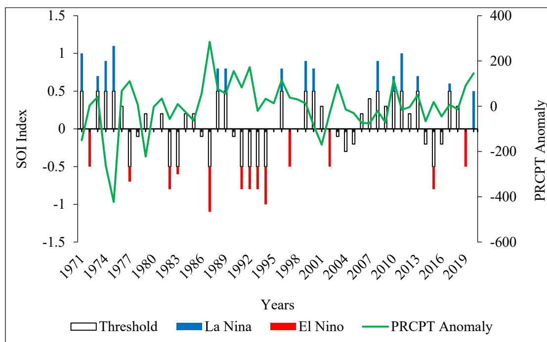
Figure 14. Precipitation in UIB during ENSO phases of SOI.
