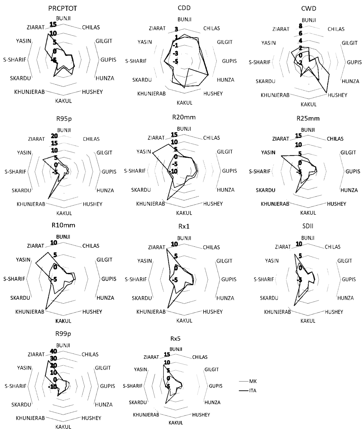
Figure 9. Radial graph representing MK test and ITA comparison.
