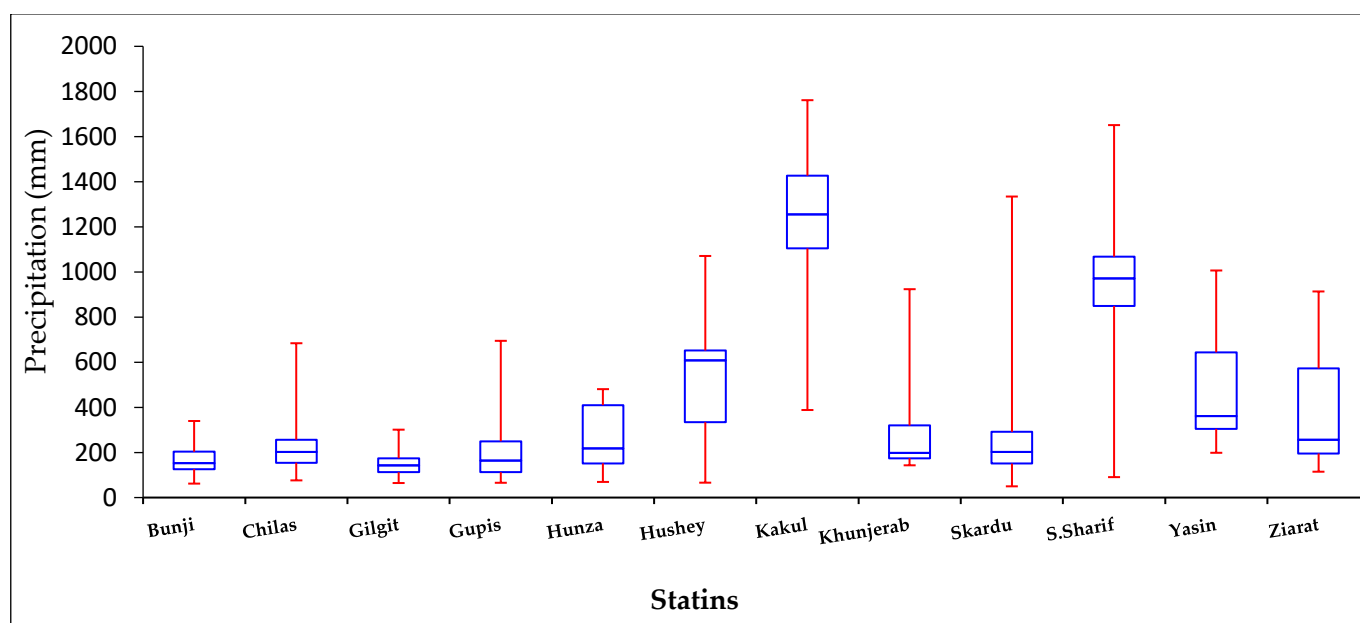
Figure 6. Temporal mean annual variation.
