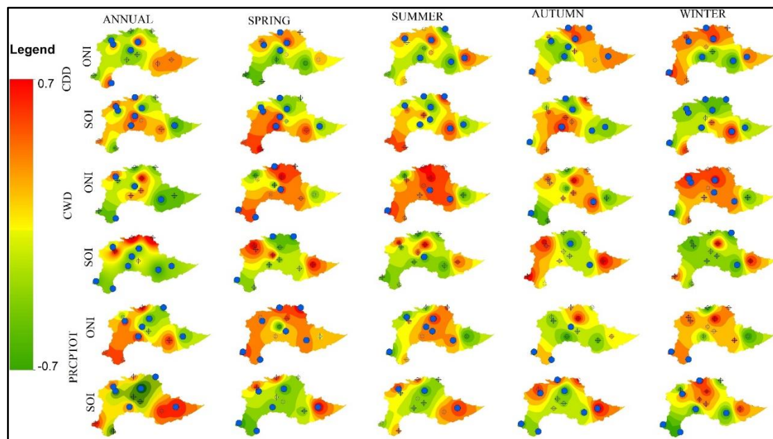
Figure 16. Spatial patterns of ENSO correlations with EPIs (PRCPTOT, CWD, CDD).
