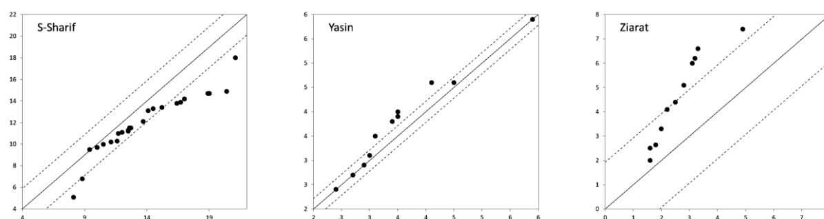
Figure A10. Results of SDII at 12 stations, obtained by using the ITA method.
