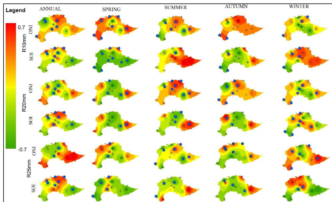
Figure 17. Spatial patterns of ENSO correlations with EPIs (R10 to R25).
