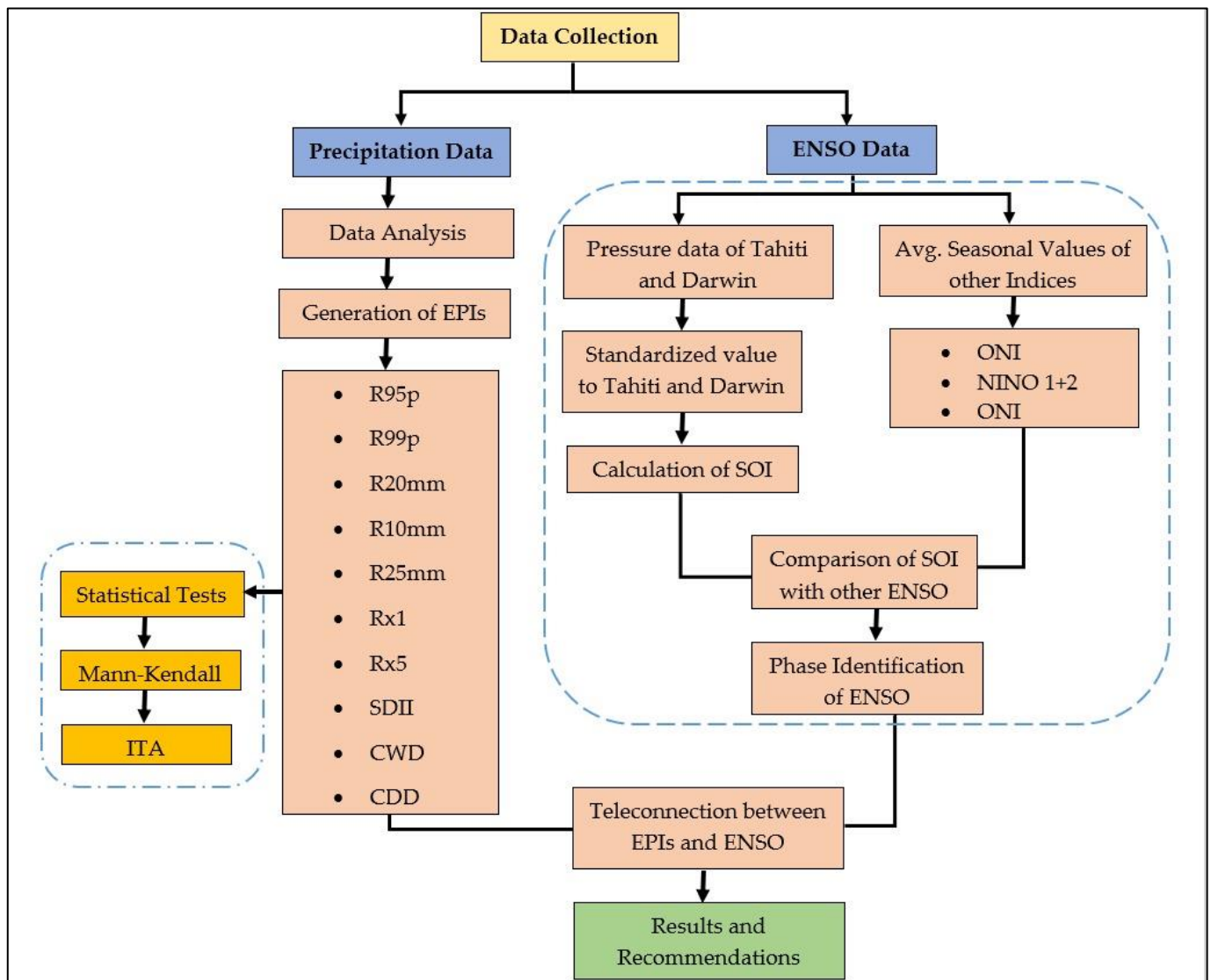
Figure 2. Schematic diagram of methodology.
