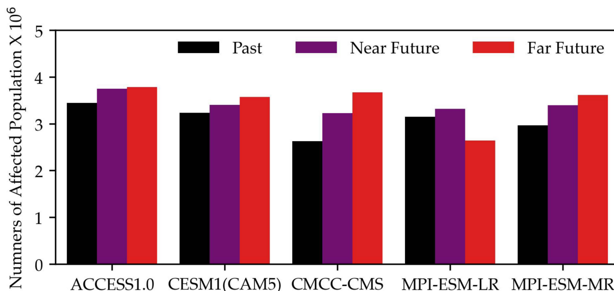
Figure 17. Number of affected people in the Sangu River basin in the past, near-future, and far-future for all selected GCMs.
