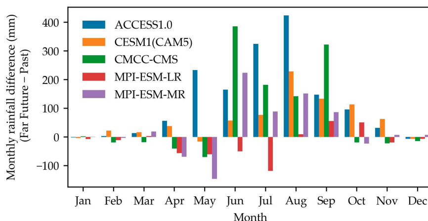
Figure 6. Monthly rainfall difference (far-future minus past) of the selected GCMs.
