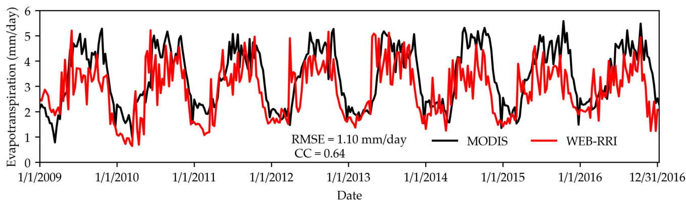
Figure 11. Comparison between basin-averaged WEB-RRI ET and MODIS ET from the year 2009 to 2016.
