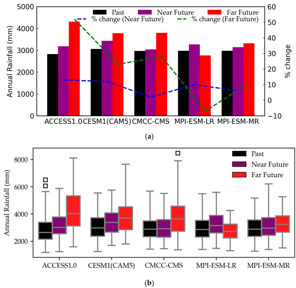
Figure 3. (a) Comparison of basin average annual rainfall among the past, near-future, and far future, and percentage change for both the near-future and far-future. (b) Box and Whiskers of annual rainfall of each GCMs for the past, near-future, and far-future. Outliers beyond \pm 2 times the interquartile range are shown by black squares.
