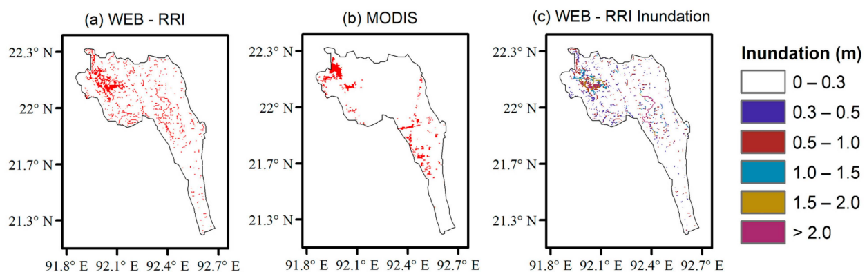
Figure 10. Comparison of flood inundation in the Sangu River basin for the flood of 2015: (a) WEB-RRI simulated inundation; (b) MLSWI using MODIS data; (c) WEB-RRI simulated inundation depth (m).
