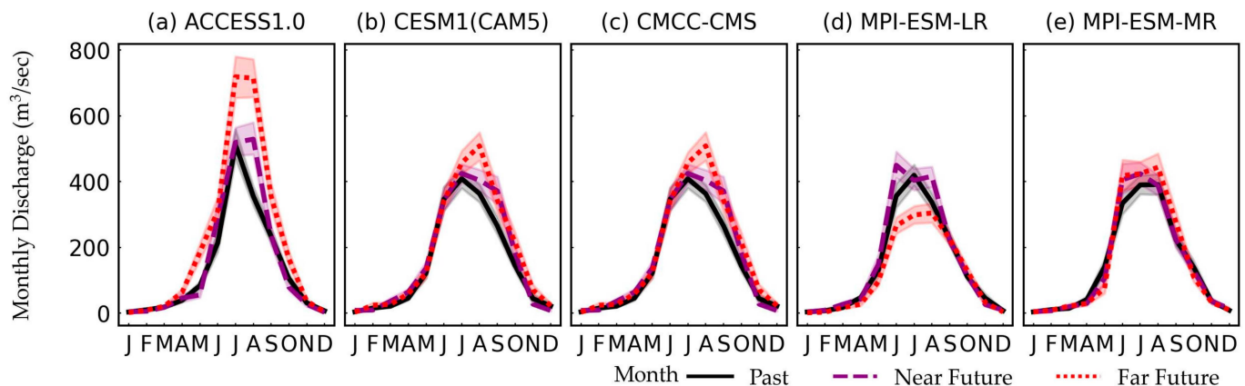
Figure 14. Comparison of monthly discharge among the past, near-future, and far-future. The solid line (past), dashed line (near-future) and dotted line (far-future) show the mean monthly discharge, and the shaded area is the 95th and 5th percentiles of monthly discharge.
