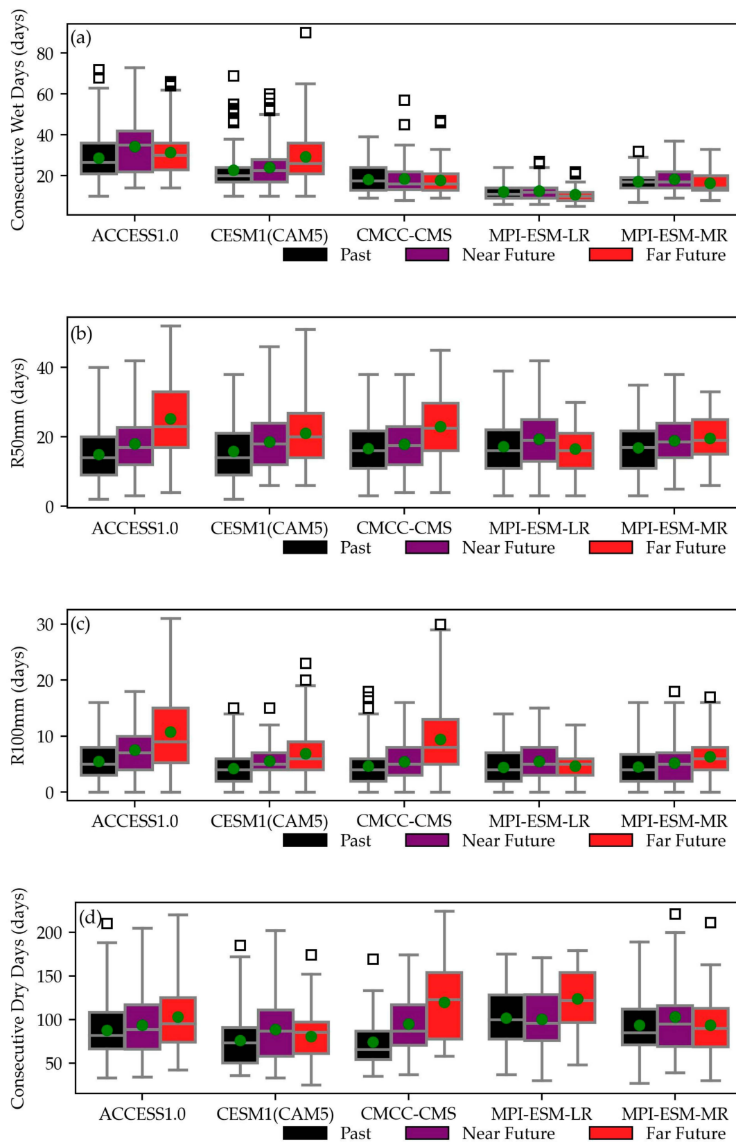
Figure 5. Box-whisker plot for (a) consecutive wet days (CWDs), (b) R50mm, (c) R100mm, and (d) consecutive dry days (CDDs). Green circles show the mean value. Outliers beyond \pm 2 times the interquartile range are shown by black squares.
