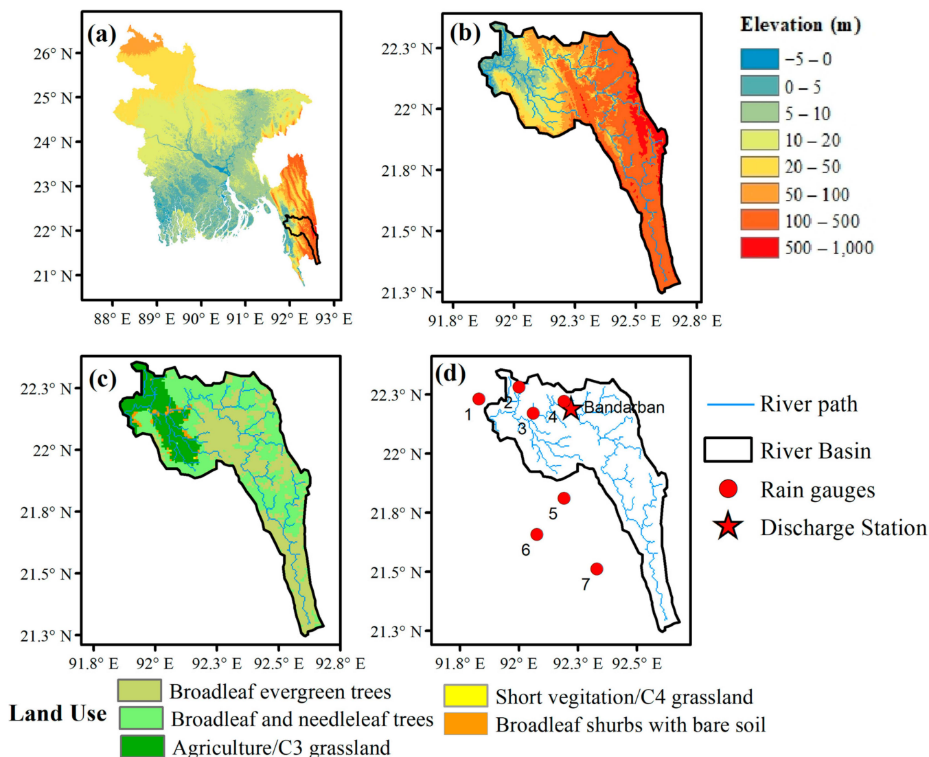
Figure 1. (a) Topographical map of Bangladesh indicating the Sangu River basin; (b) topography of Sangu River basin; (c) land use in the basin; (d) demarcation of rain-gauge and discharge station in the basin.
