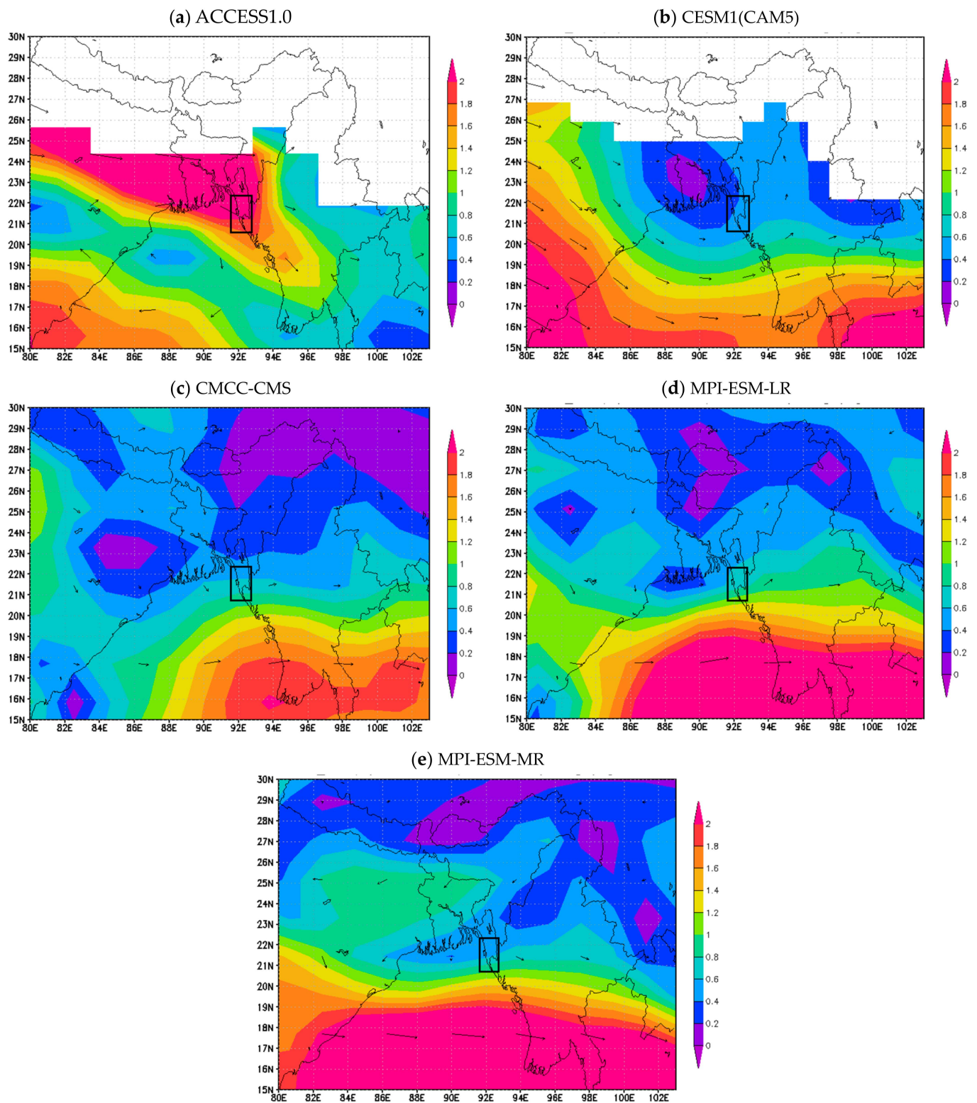
Figure 7. Wind speed ratio (far-future divided by past) for the month of June. (a) ACCESS1.0, (b) CESM1(CAM5), (c) CMCC-CMS, (d) MPI-ESM-LR, (e) MPI-ESM-MR. Study area is located within the black box. Arrows are wind direction.
