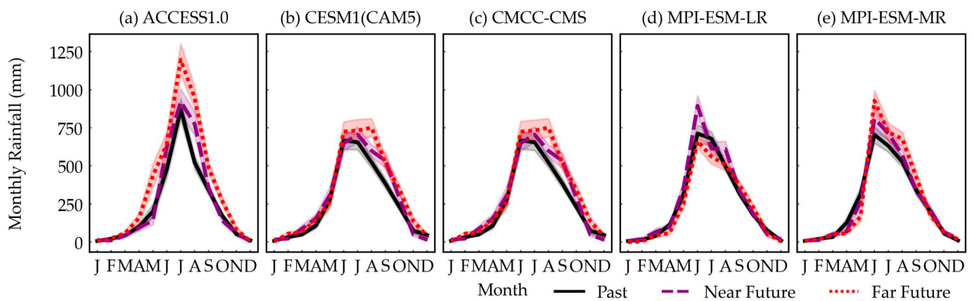
Figure 4. Comparison of monthly rainfall among the past, near-future, and far-future. The solid line (past), dashed line (near-future), and dotted line (far-future) show the mean monthly rainfall, and the shaded area is the 95th and 5th percentiles of monthly rainfall.
