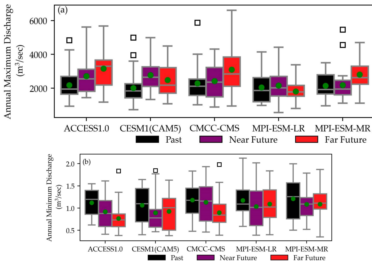
Figure 13. Box and Whiskers of (a) annual daily maximum discharge and (b) annual daily minimum discharge at the Bandarban gauging station for the selected GCMs. Green circles show the mean value. Outliers beyond \pm 2 times the interquartile range are shown by black squares.
