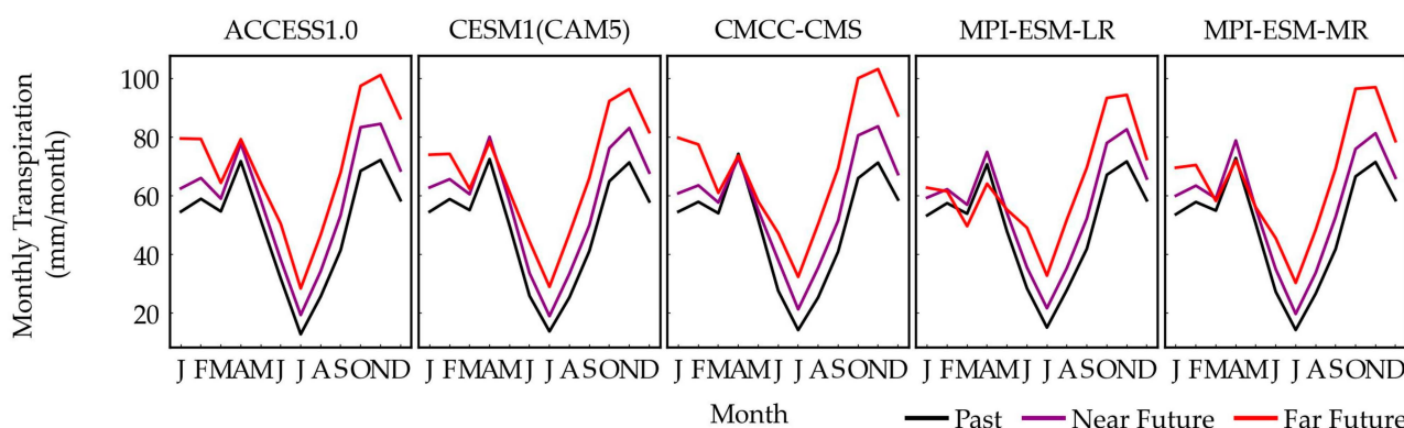
Figure 19. Monthly transpiration for all selected GCMs in the past, near-future, and far-future.
