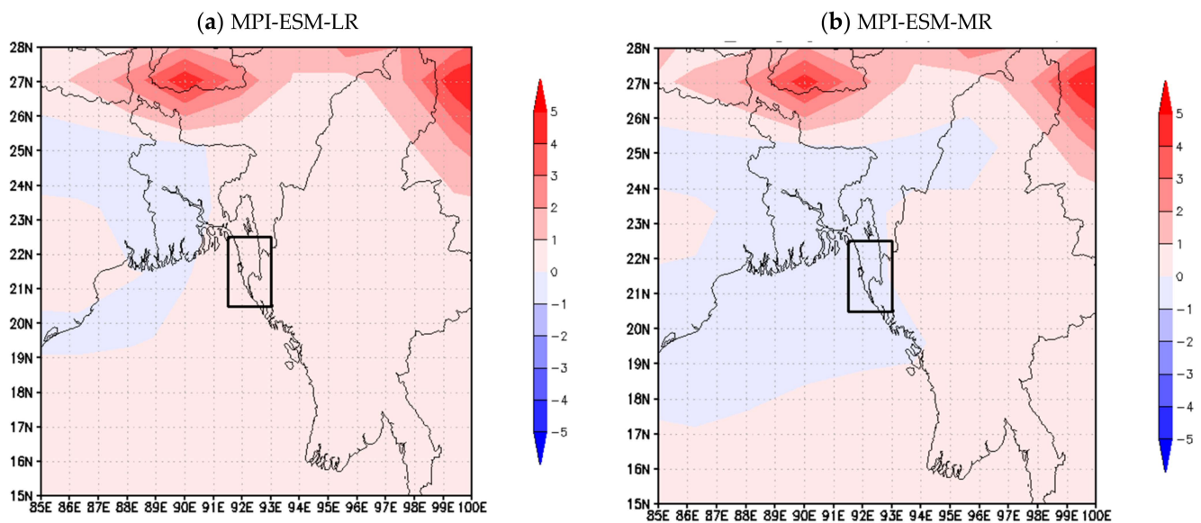
Figure 8. Pressure difference (far-future minus past) for the month of July. (a) MPI-ESM-LR, (b) MPI-ESM-MR. Study area is located within the black box.
