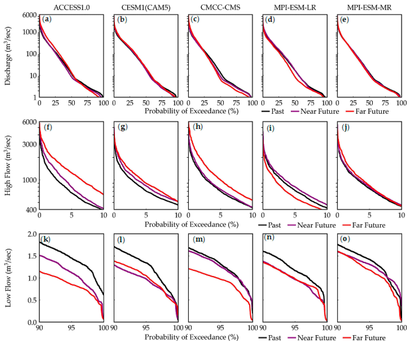
Figure 15. Flow duration curve for the past, near-future, and far-future. (a–e) Entire period, (f–j) high flows (probability of exceedance \leq 10\% ), and (k–o) low flows ( 90\% \leq probability of exceedance \leq 100\% ).
