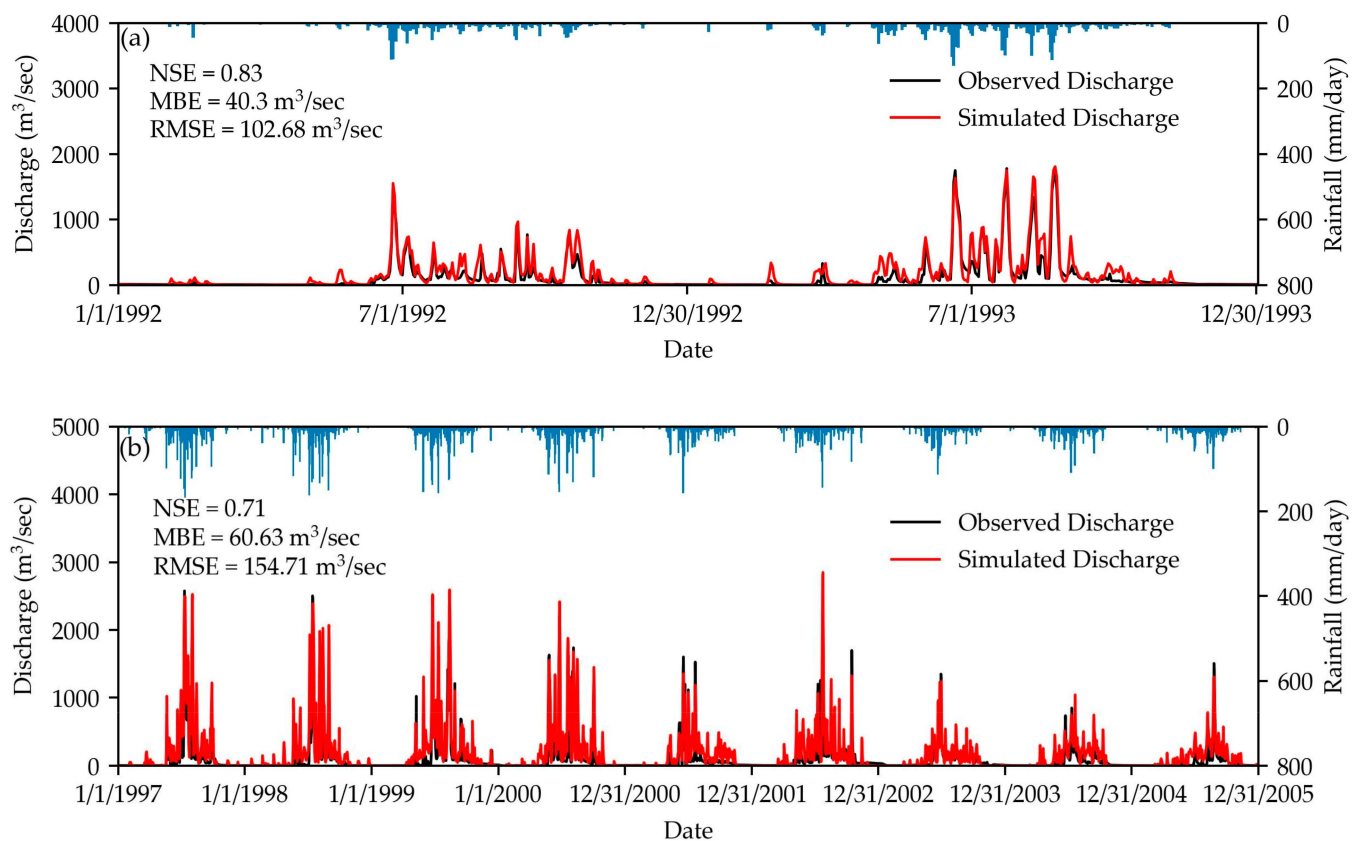
Figure 9. Comparison between observed discharge and simulated discharge (a) model calibration for 1992–1993, and (b) model validation for 1997–2005.
