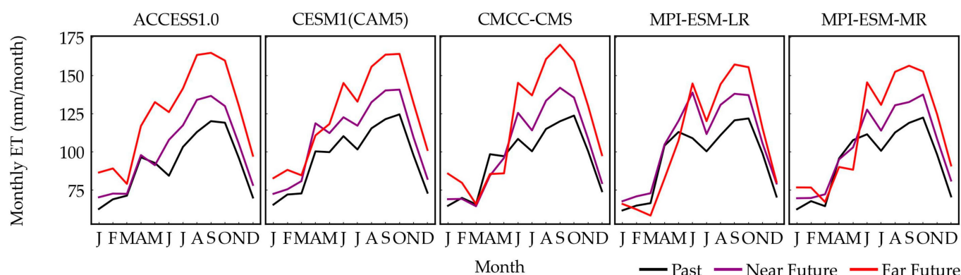
Figure 18. Monthly ET for the all selected GCMs in the past, near-future, and far-future.
