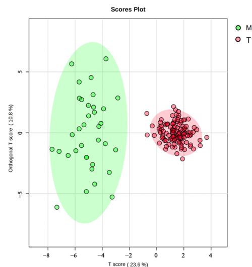
Figure 7. OPLS-DA of G. dybowskii from geographically distinct populations; T is the population from the Turks River, and M is the population from the Manas River; the vertical coordinate “Orthogonal T Score” indicates the orthogonal principal components test score, which responds to within-group differences. The horizontal coordinate “T Score” indicates the predictive principal component test score, which reflects the difference between groups.
