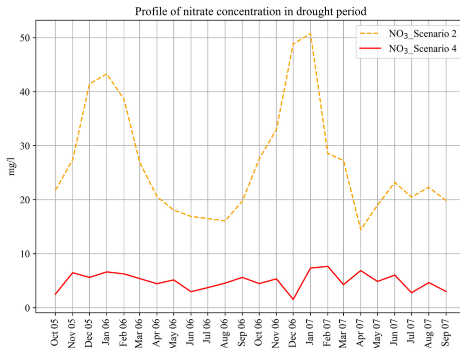
Figure 11. Evolution of nitrate concentration simulated using the GESCAL model for Scenarios 2 and 4 during the drought period.
