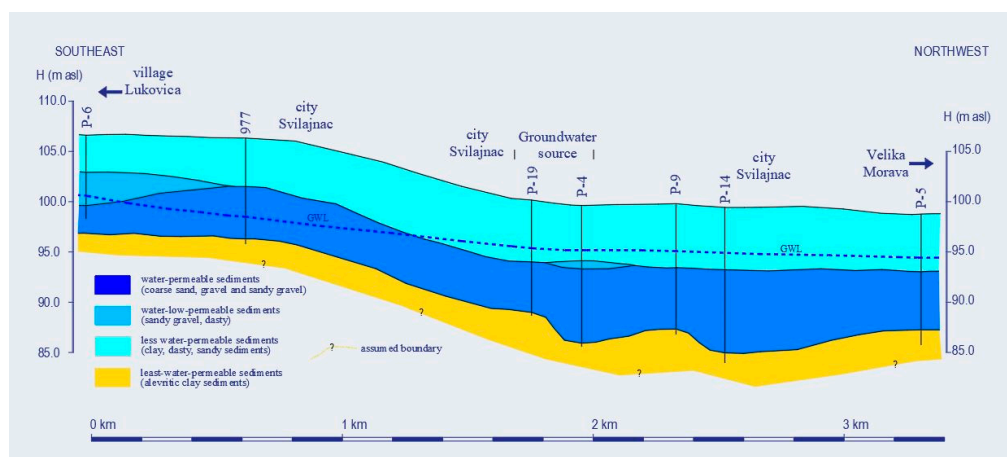
Figure 2. Hydrogeological profile of examined alluvial plain.
