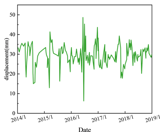
Figure 16. The extraction results of the displacement residual components for TJZ.
