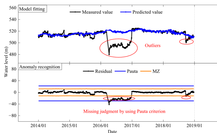
Figure 17. Anomaly early warning threshold of uplift pressure observation point YY10101 in GZ (burial depth: 5 m, sandstone stratum).
