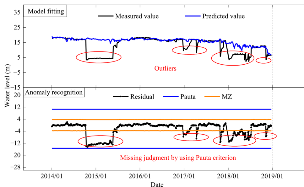
Figure 18. Anomaly early warning threshold of uplift pressure observation point YY813 in GZ (burial depth: 6.5 m, limestone interlayer; limestone strata exhibit higher permeability, causing greater pressure fluctuations than sandstone layers).
