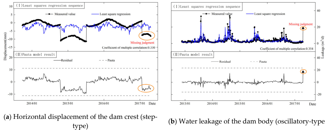
Figure 3. Statistical process control chart of step-type and oscillatory-type data sequences in a dam.
