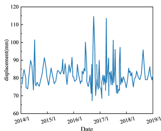
Figure 15. The extraction results of the displacement residual components for GZ.
