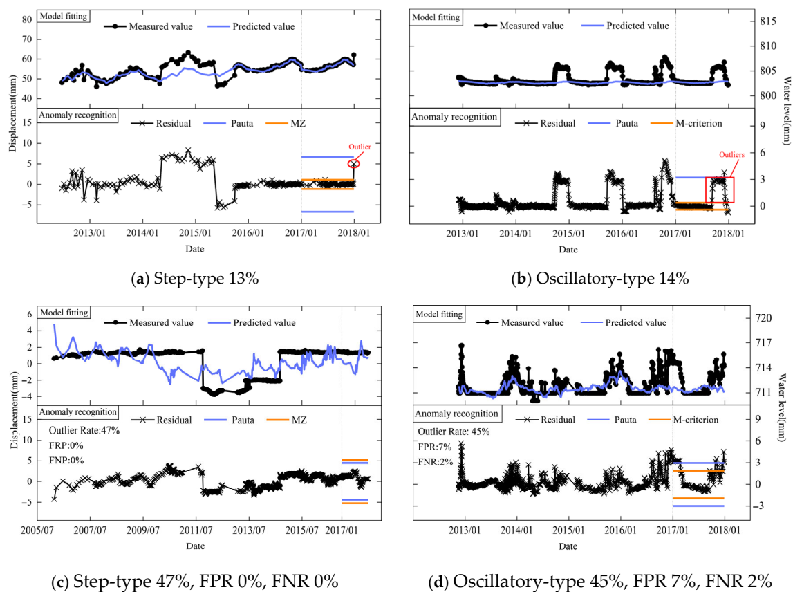
Figure 12. Statistical process control chart of anomaly identification of typical step-type and oscillatory-type data sequences. The percentage denotes the proportion of the outliers.
