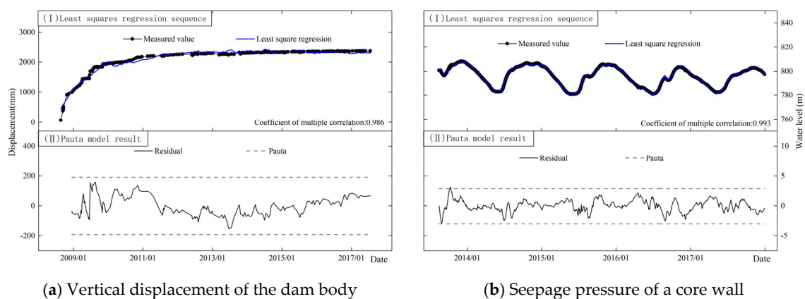
Figure 1. Statistical process control chart of data sequences obtained from typical measuring points in a dam.
