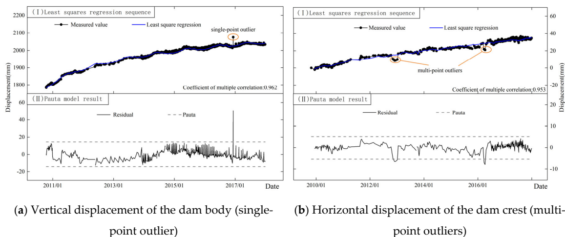
Figure 2. Statistical process control chart of data sequences with a small number of outliers.
