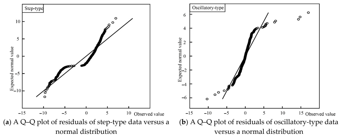
Figure 4. Normality tests of residuals of step-type and oscillatory-type monitoring data in a dam.
