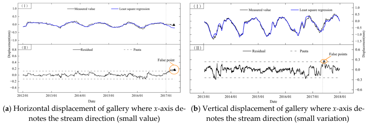
Figure 5. Statistical process control chart of small-value displacement sequences in XB dam. (I) Least squares regression sequence. (II) Pauta model result.
