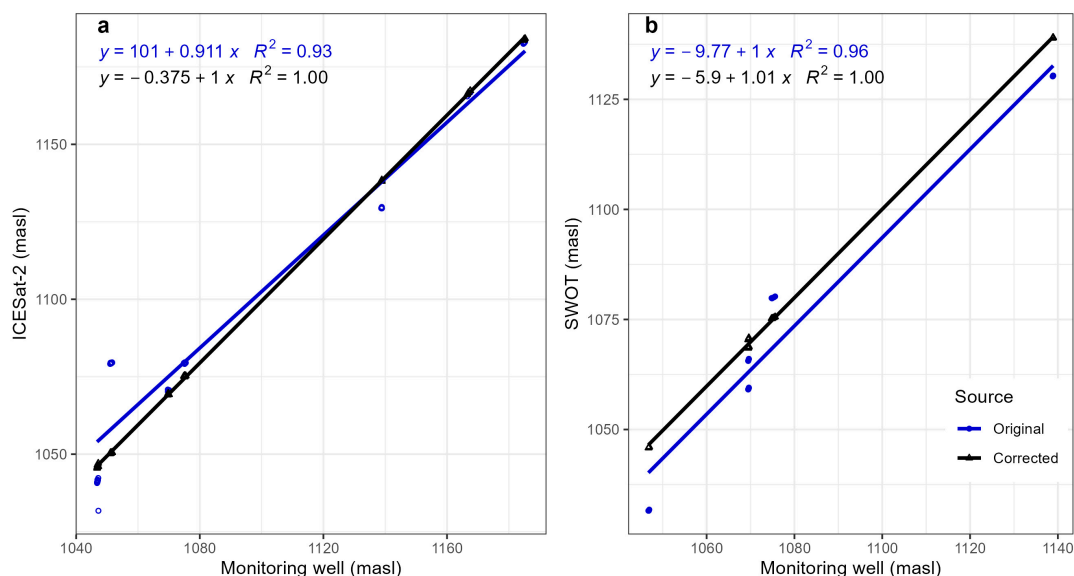
Figure 3. A comparison plot between the ICESat-2 (a) and SWOT (b) water level estimates in the Sandhills indicates high correlation and correspondence. Blue points are uncorrected LGLs, and black points are corrected for ambient hydraulic gradients between lakes and observation wells.
