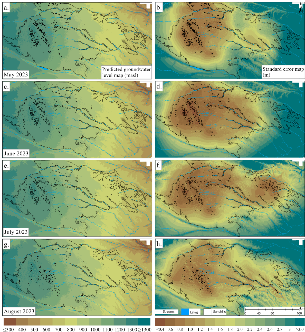
Figure 5. Monthly groundwater level maps estimated using a generalized additive model (GAM) in the Nebraska Sandhills. Maps on the left side (a,c,e,g) show the predicted groundwater level (masl) while the corresponding maps on the right (b,d,f,h) show the standard error (m) associated with the corresponding months.
