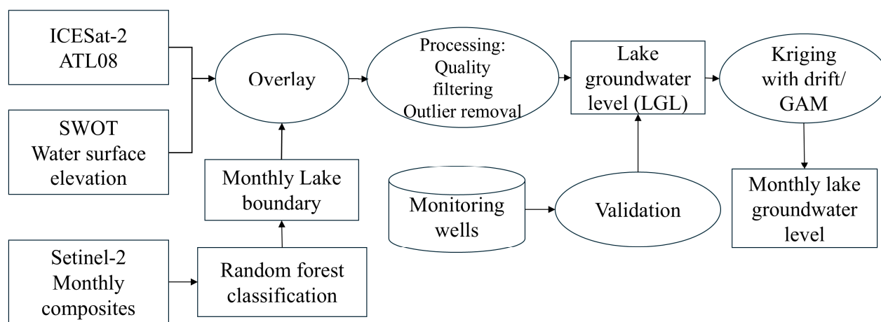
Figure 2. Workflow to compute monthly lake groundwater level (LGL) using satellite altimetry, kriging with an external drift, and a generalized additive model. Rectangular shapes indicate data/output, oval shapes indicate major process and database.
