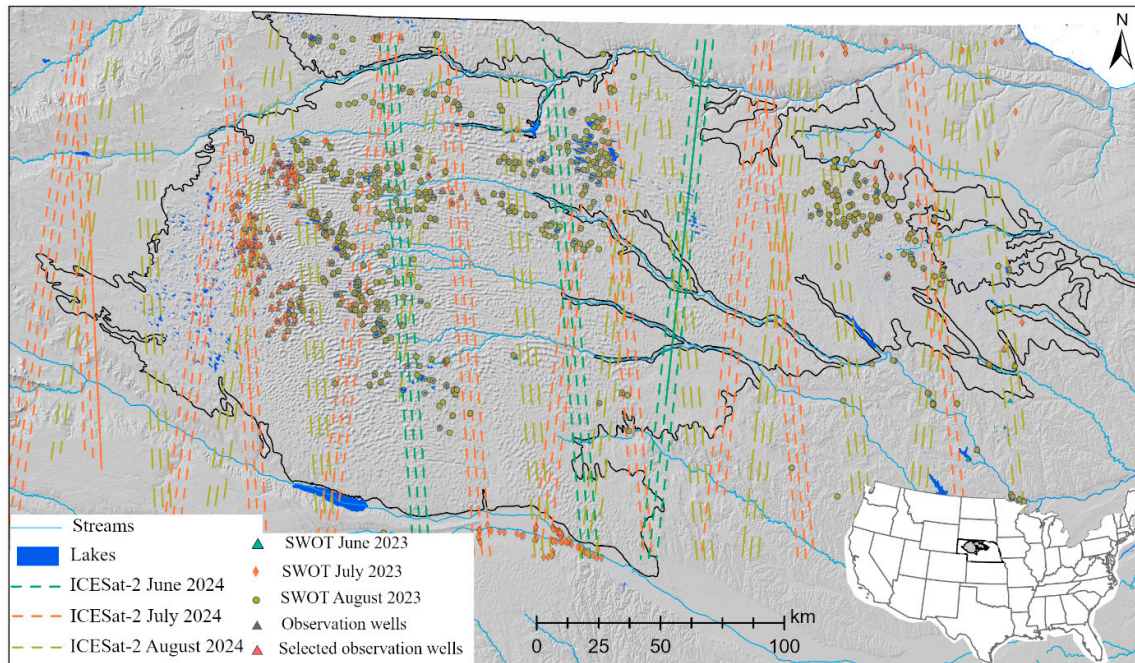
Figure 1. Distribution of lakes, satellite altimetry observations, and observation wells in the Nebraska Sandhills (Sandhills). ICESat-2 samples the central Sandhills during June and most of the Sandhills during July and August. SWOT samples cover most of the Sandhill lakes for each of the months considered for the study period. Therefore, a combination of ICESat-2 and SWOT enables monthly lake water level measurements and subsequent groundwater levels in the Sandhills. We selected observation wells near lakes and underlying unconfined aquifers to validate our estimations made from lake water levels.
