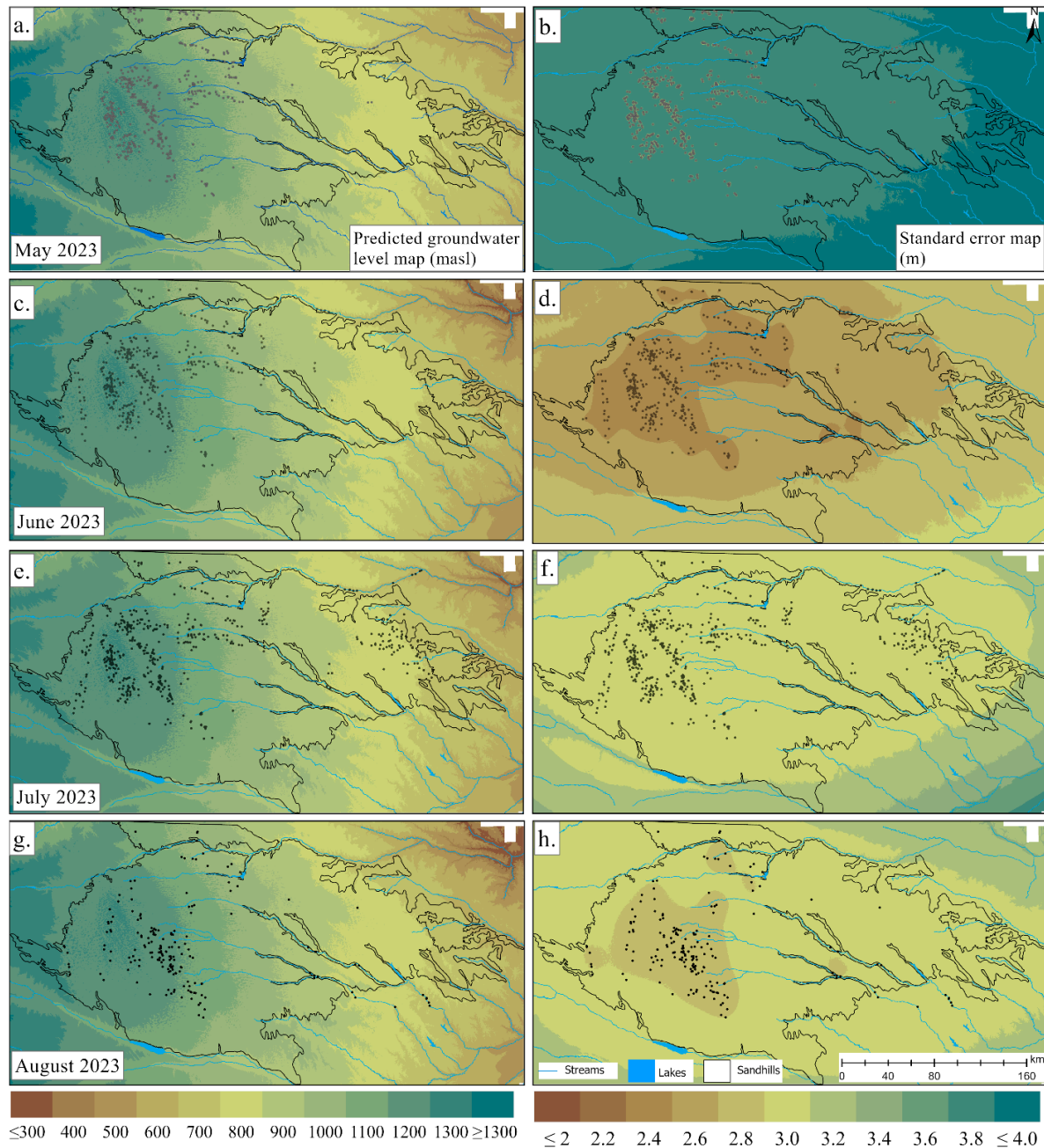
Figure 4. Monthly groundwater level maps estimated using kriging with an external drift in the Nebraska Sandhills. The left panels (a,c,e,g) show the predicted groundwater level (masl) while the right panels (b,d,f,h) show the standard error (m) associated with the corresponding months.
