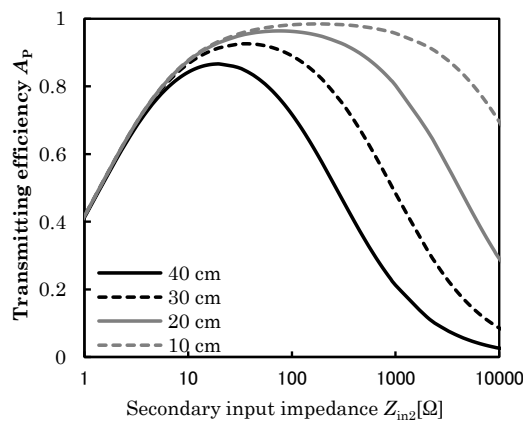
Figure 4: Relation efficiency and load resistance
