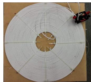
Figure 3: An antenna for Wireless power transfer
