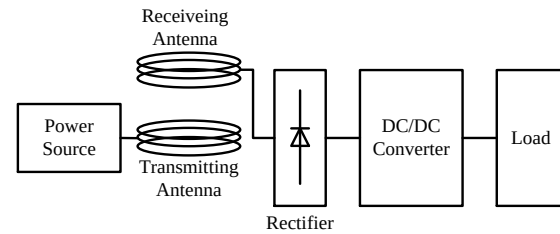
Figure 5: Impedance control by DC-DC converter
