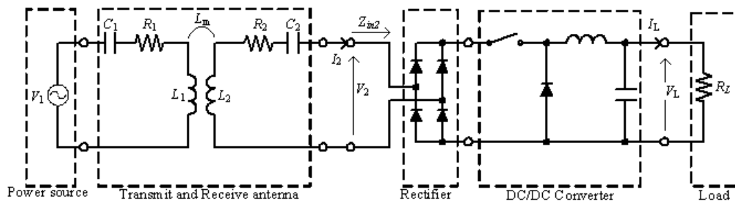
Figure:7 Circuit diagram of WPT system with DC-DC converter for maximize transmitting efficiency
