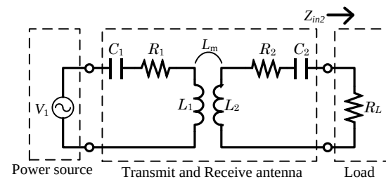
Figure 2: Equivalent circuit of magnetic resonant coupling with power source and load
