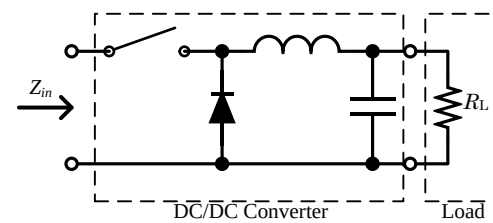
Figure 6: Buck converter
