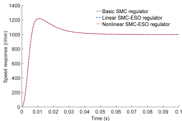
(a) Speed response.
