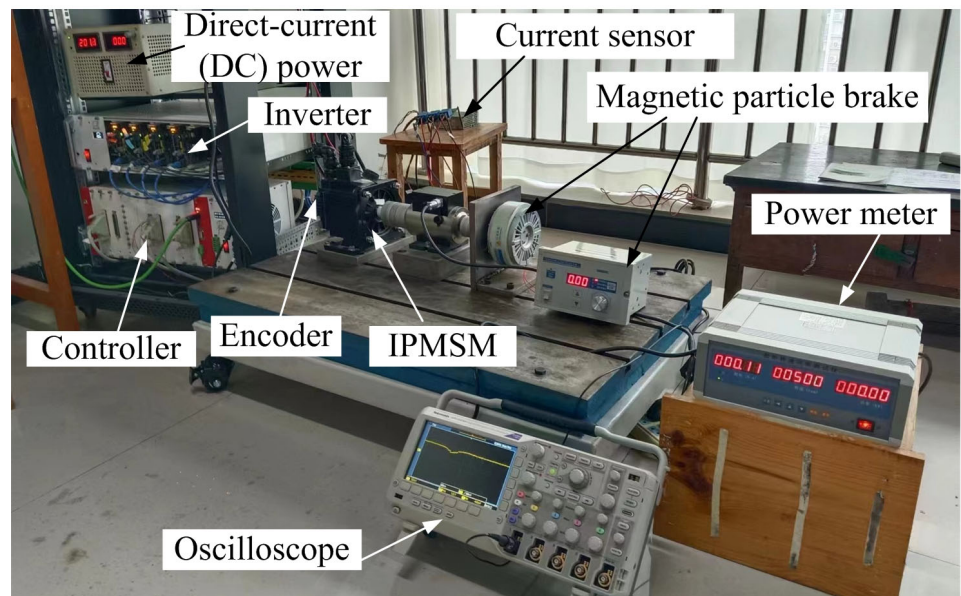
(b) Hardware Platform.
