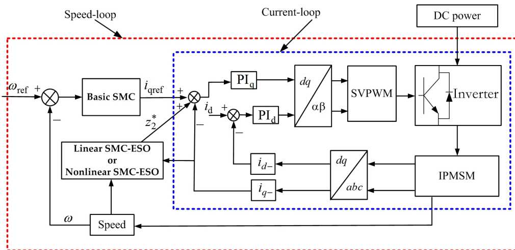
Figure 2. System frame of simulation model of IPMSM.
