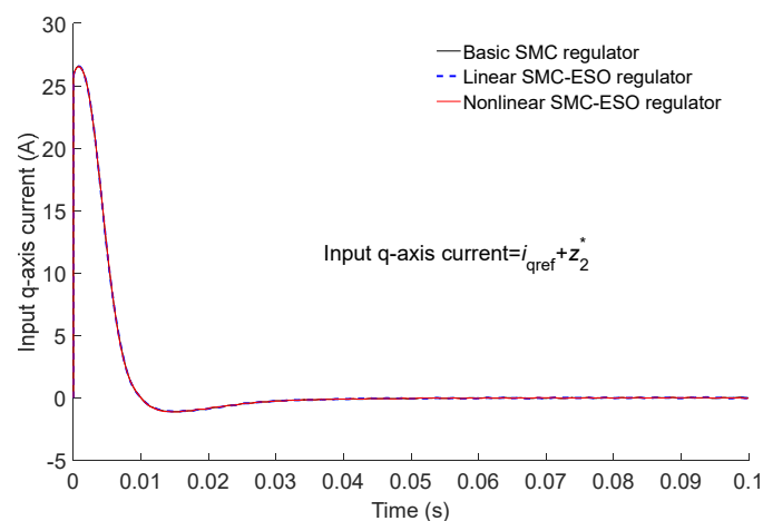
(b) Input q-axis current response.
