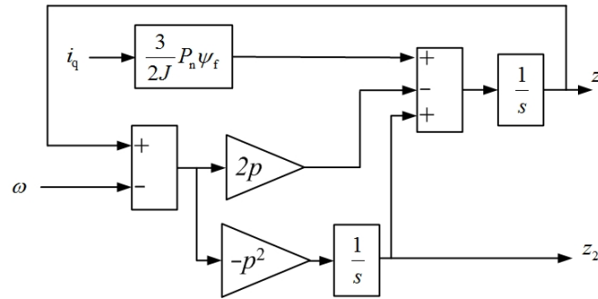
Figure 1. The basic structure of linear second-order ESO.
