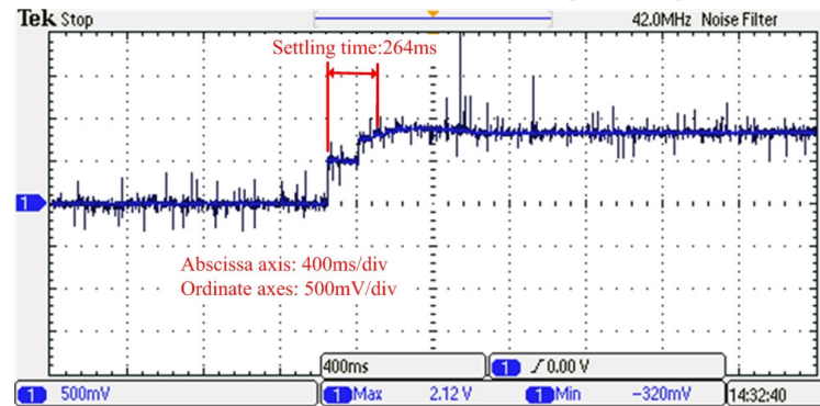
(c) Nonlinear SMC-ESO regulator of speed-loop.
