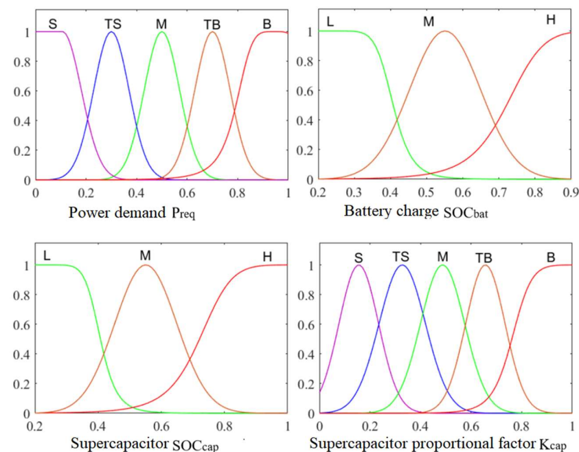
Figure 9. Membership function of fuzzy controller when driving.
