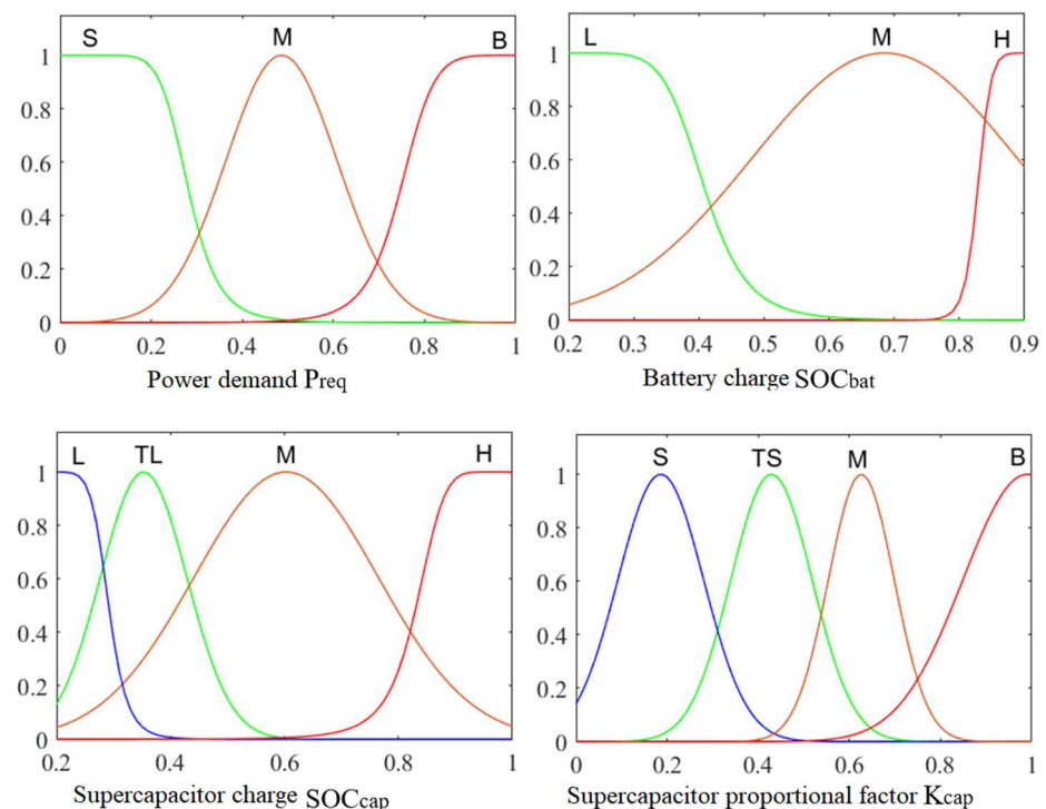
Figure 15. Optimized membership function of FLC when braking.
