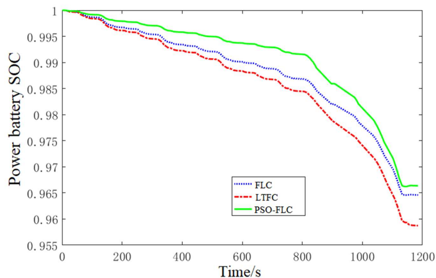
Figure 19. Comparison of battery SOC under different control strategies.
