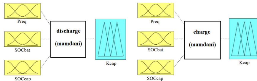
Figure 8. Structure of fuzzy logic controller in drive and brake modes.
