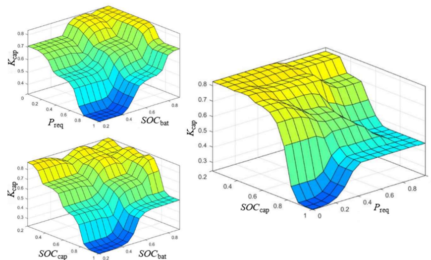
Figure 12. Relation between input and output when braking.
