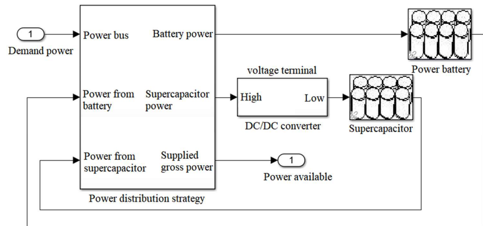
Figure 16. Top-level model of HESS.
