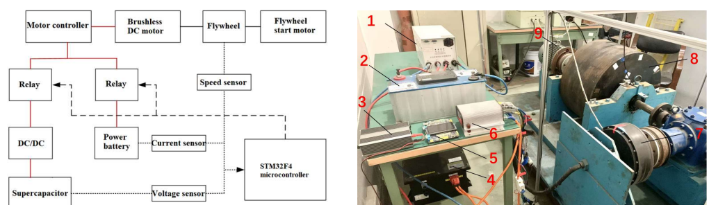
Figure 1. Experimental platform for HESS. 1. DC/DC converter; 2. supercapacitor; 3. DC power supply; 4. power battery; 5. microcontroller; 6. motor controller; 7. DC brushless motor; 8. flywheel; 9. flywheel start motor.
