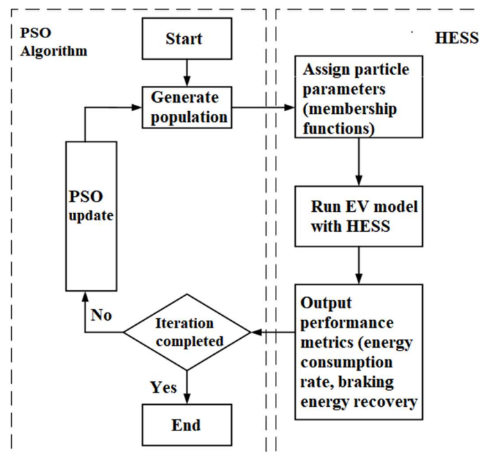
Figure 13. Flow chart of optimization model solution.
