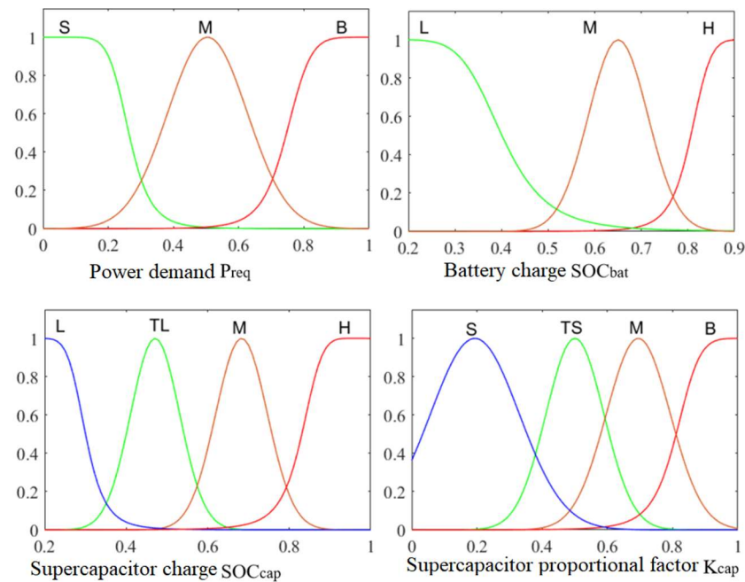
Figure 10. Membership function of fuzzy controller when braking.
