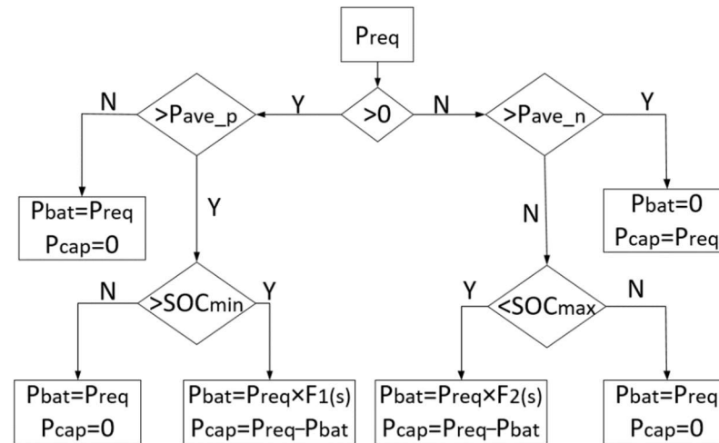
Figure 7. Basic flow of LTFC strategy.
