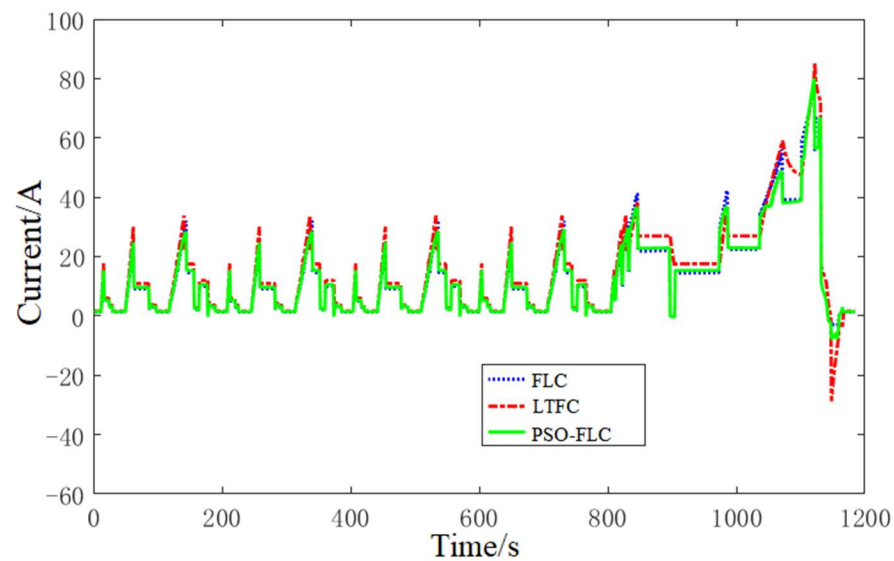
Figure 20. Comparison of battery current under different control strategies.
