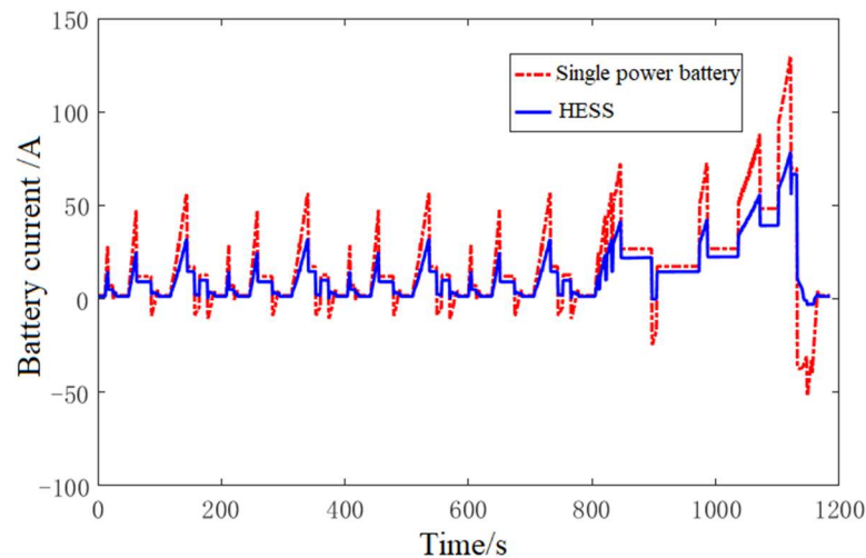
Figure 18. Comparison of battery current between pure battery system and hybrid energy storage system.
