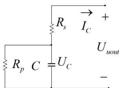
Figure 3. Supercapacitor RC model.
