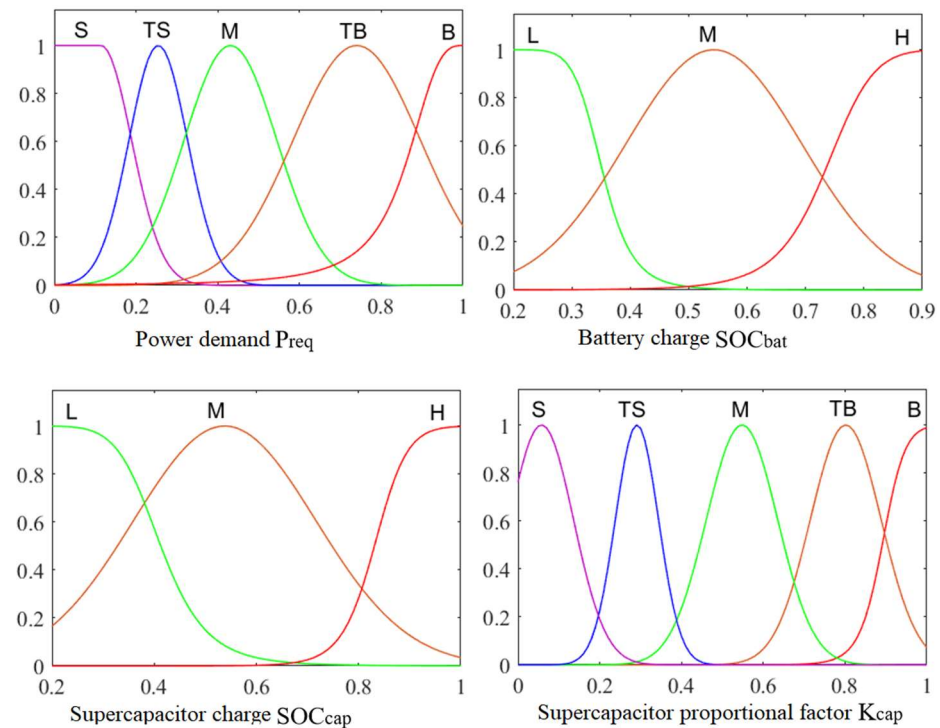
Figure 14. Optimized membership function of FLC when driving.
