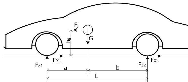
Figure 5. Force analysis of vehicle when braking.
