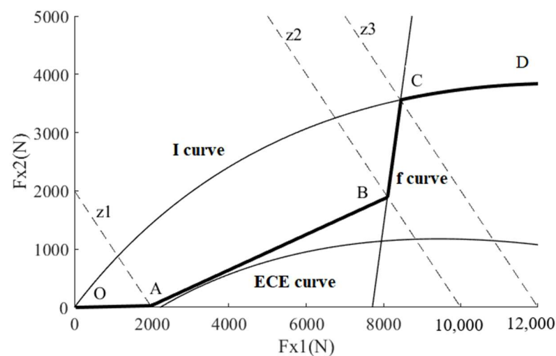
Figure 6. Schematic diagram of SBFDS.
