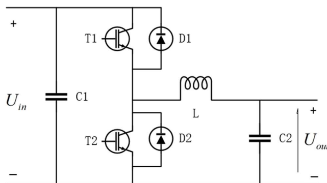
Figure 4. Simplified circuit of the bidirectional DC/DC converter.
