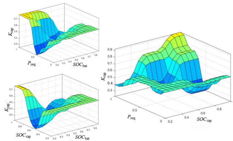
Figure 11. Relation between input and output when driving.
