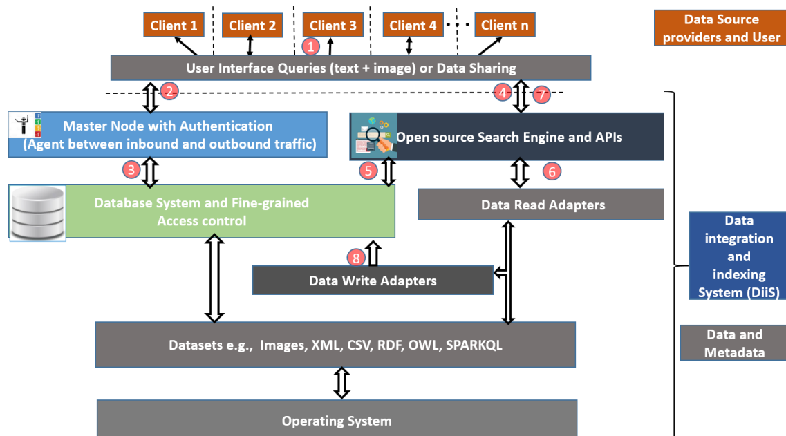
Figure 2. Architecture of proposed system.
