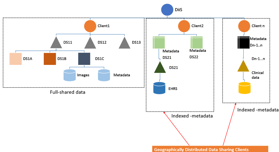
Figure 3. Hierarchical structure of Data Sources indexing (DS: Data Source).
