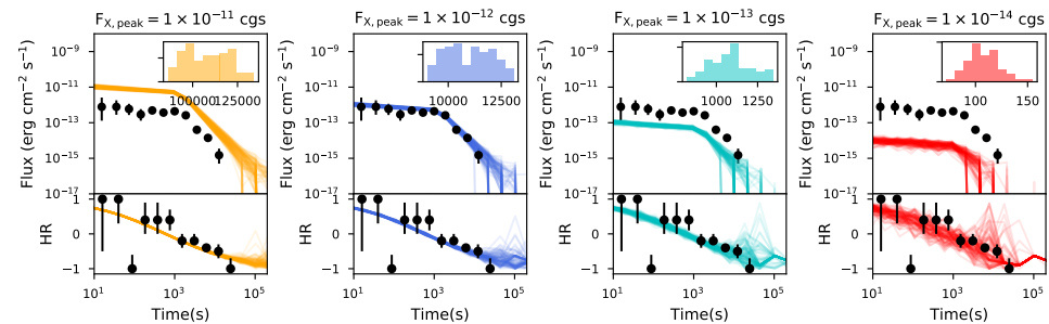
Figure 2. Simulated AXIS light curves ( upper panels ) and hardness ratios ( lower panels ) of FXTs with 5 ks 0.5–8 keV peak fluxes of 1 \times 10^{-11} , 1 \times 10^{-12} , 1 \times 10^{-13} , and 1 \times 10^{-14} \text{ erg s}^{-1} \text{ cm}^{-2} , assuming the light-curve properties of CDF-S XT2 (Chandra light curve shown as black points; [18]). We adopt a hardness ratio given by H-S/H+S , where S = 0.5\text{--}2 \text{ keV} and H = 2\text{--}8 \text{ keV} . The colored light curves denote 100 AXIS realizations to demonstrate the error distribution. The inset histogram shows the number of counts for the simulated AXIS light curves; the real AXIS light curve will also incur some gaps due to the low-Earth orbit. AXIS will be capable of probing subtle spectral variations and temporal structure for many dozens of bright FXTs, and will broadly characterize the flux and spectral evolution for hundreds of faint FXTs.
